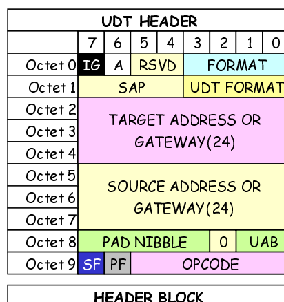
Figure B.1: UDT header Block
