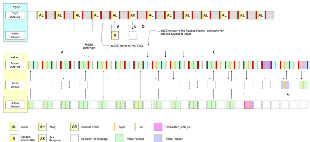
Figure 6.37: Payload Interrupt
