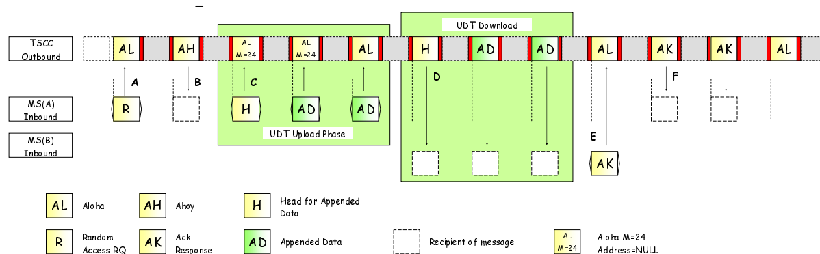
Figure 6.59: Example of a Dynamic Group Numbering Assignment transfer
