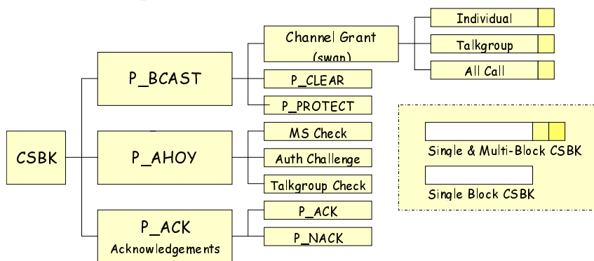
Figure 7.3: Hierarchy for Outbound channel CSBKs/MBCs on a payload channel
