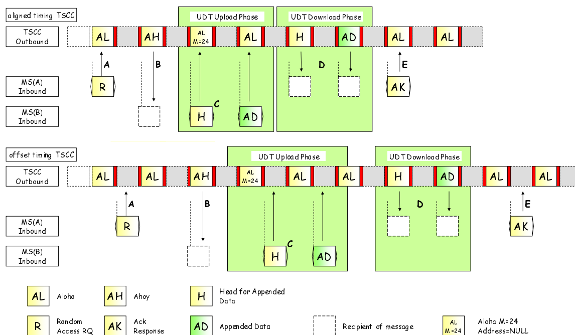
Figure 6.60: Example of a UDT Short Data Polling Transfer
