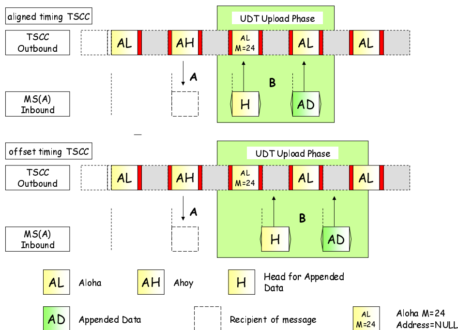
Figure 6.61: Example of UDT Short Data Polling from a Gateway
