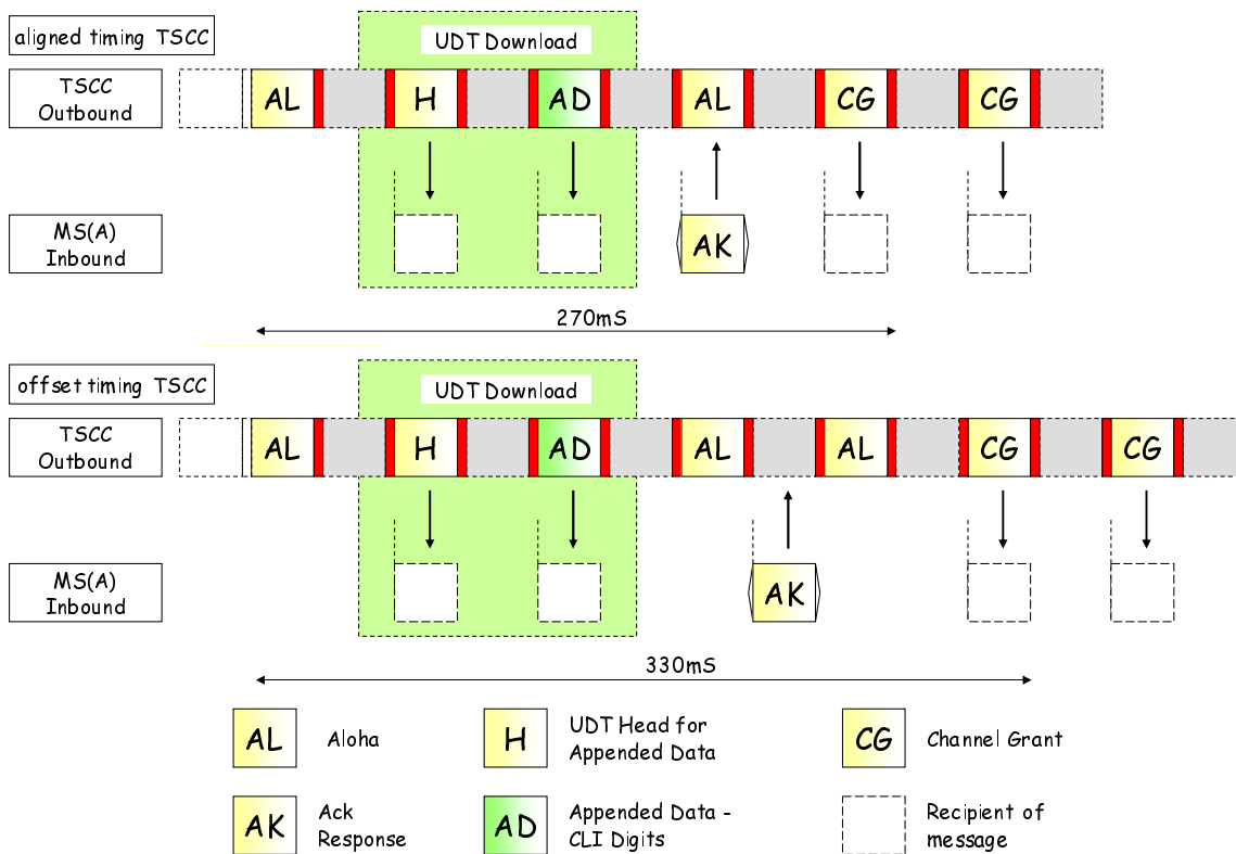
Figure 6.45: Call from the PSTN/PABX using the UDT Mechanism
