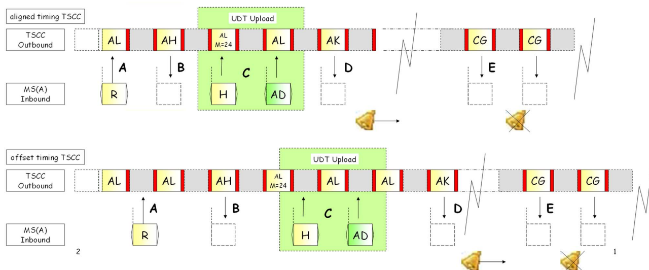
Figure 6.49: Example of Multi-part call procedure (Local Ringing Call Accepted)
