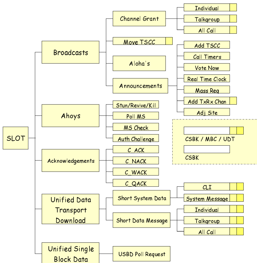
Figure 5.3: TSCC CSBK/MBC/UDT/USBDD Outbound Channel Structure
