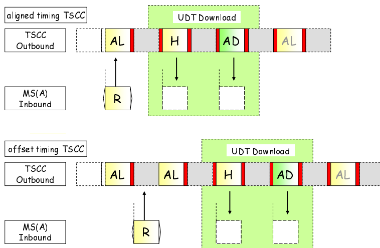
Figure 6.66: TSCC Provides Diverted Address to MS
