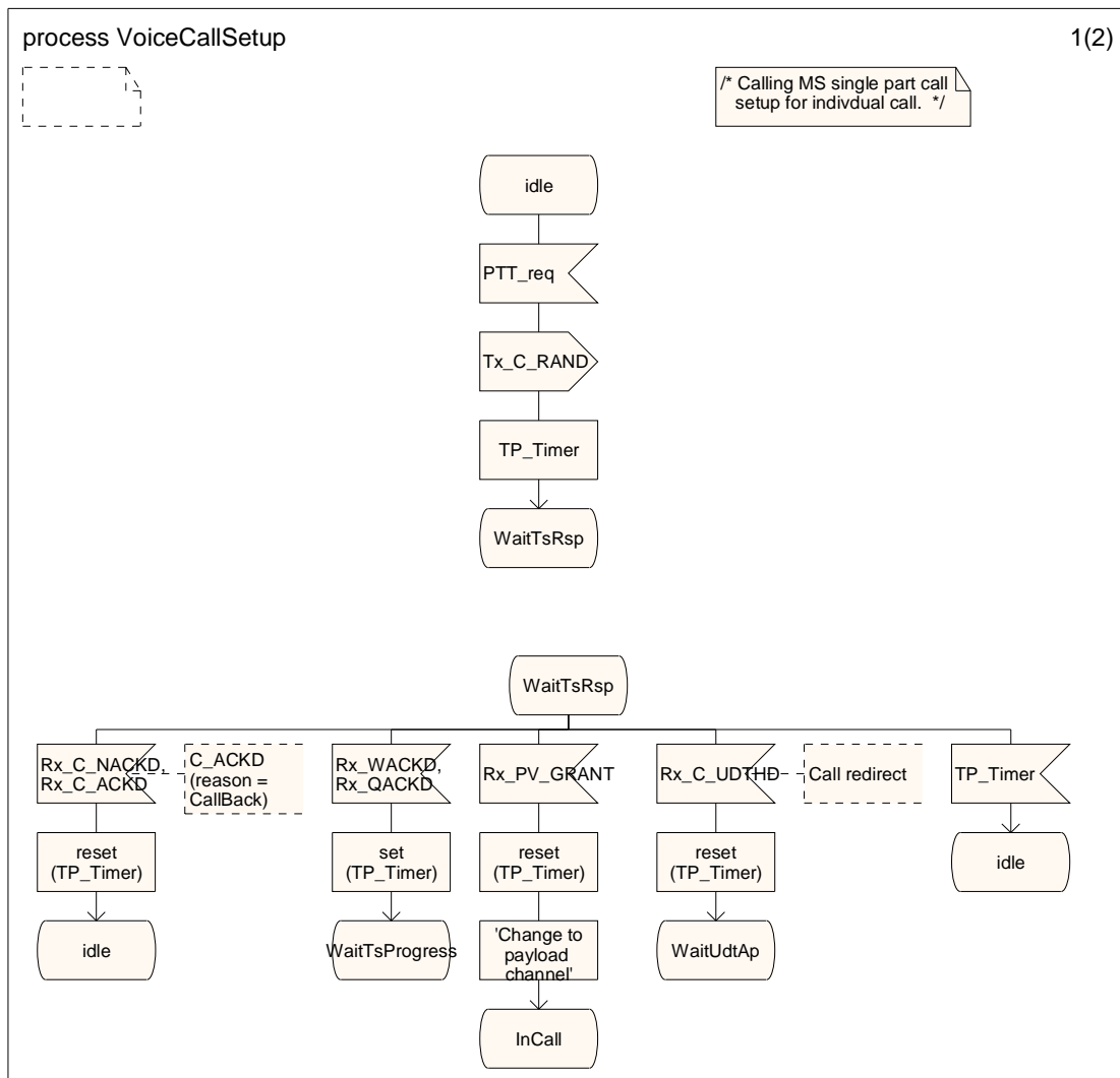
Figure 6.53 (sheet 1 of 2): Single Part OACSU Voice Call Setup SDL
