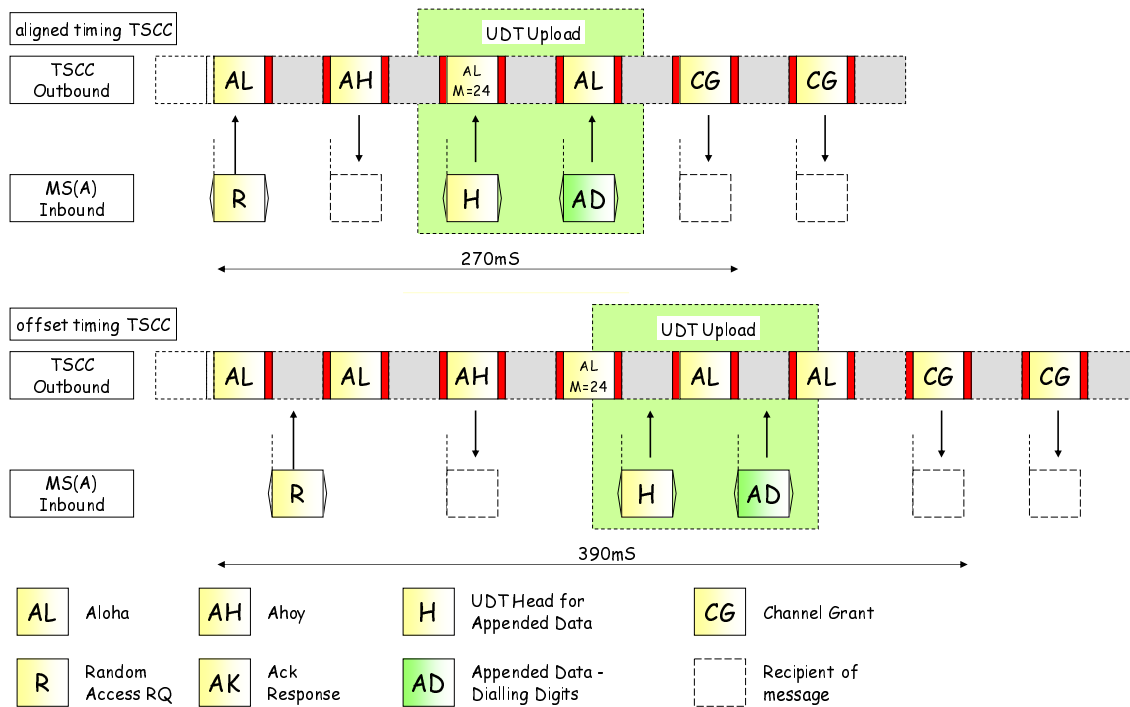
Figure 6.44: MS to PABX/PSTN Call using the UDT Mechanism
