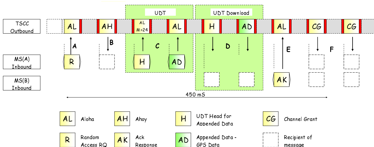
Figure 6.38: UDT Mechanism Carrying Supplementary Data for a Voice Call
