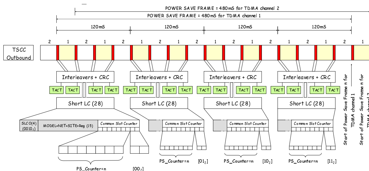
Figure 6.29: Power Save Frame Structure
