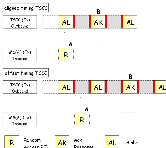
Figure 6.24: Registration with Single Talkgroup Subscription/Attachment
