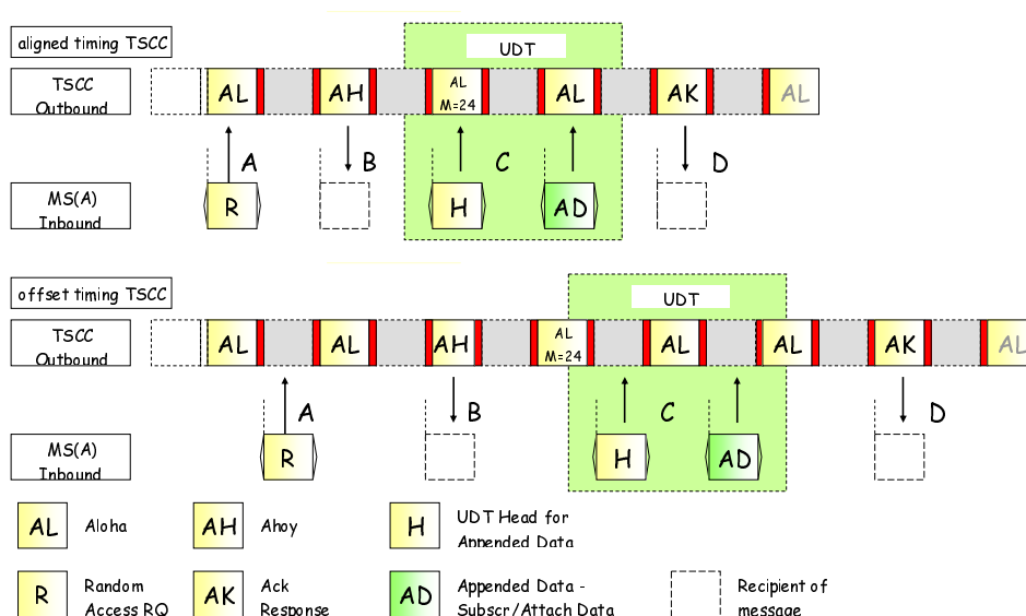
Figure 6.25: Registration with Talkgroup list Subscription/Attachment
