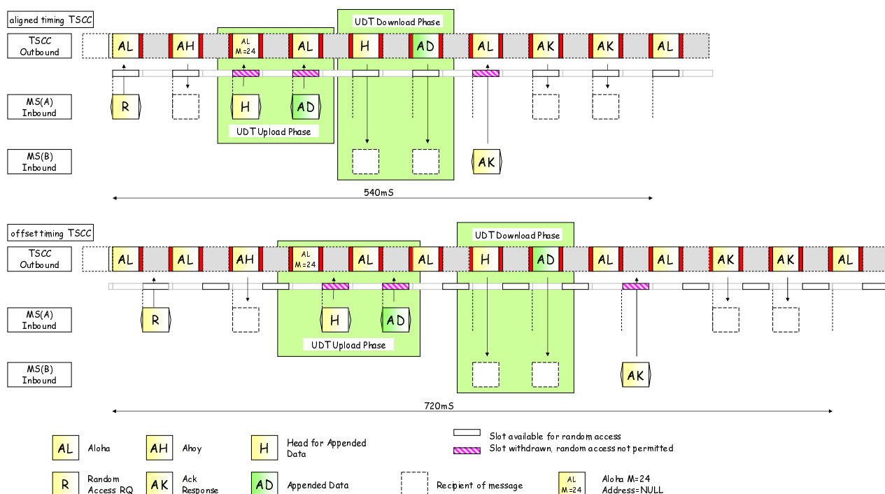
Figure 6.43: A UDT Short Data Call using the UDT Mechanism
