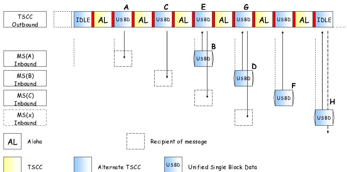
Figure 6.70: Example of Unified Single Block Data Polling. Response Delay = 90 mS using Aligned Timing (Response Delay = 01_2 )
