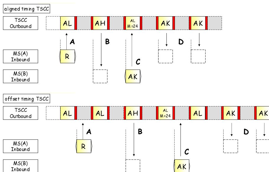
Figure 6.64: Example of the Status Polling Service
