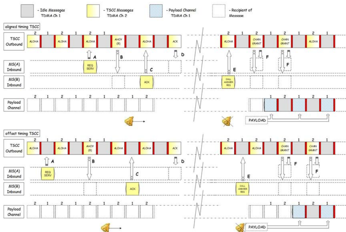
Figure 6.51: Call Answer Mechanism for FOACSU
