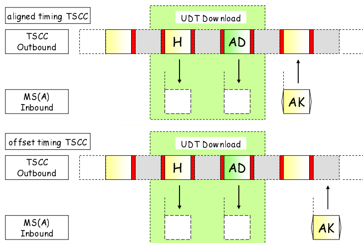
Figure 6.37: Supplementary_User Data Service outbound
