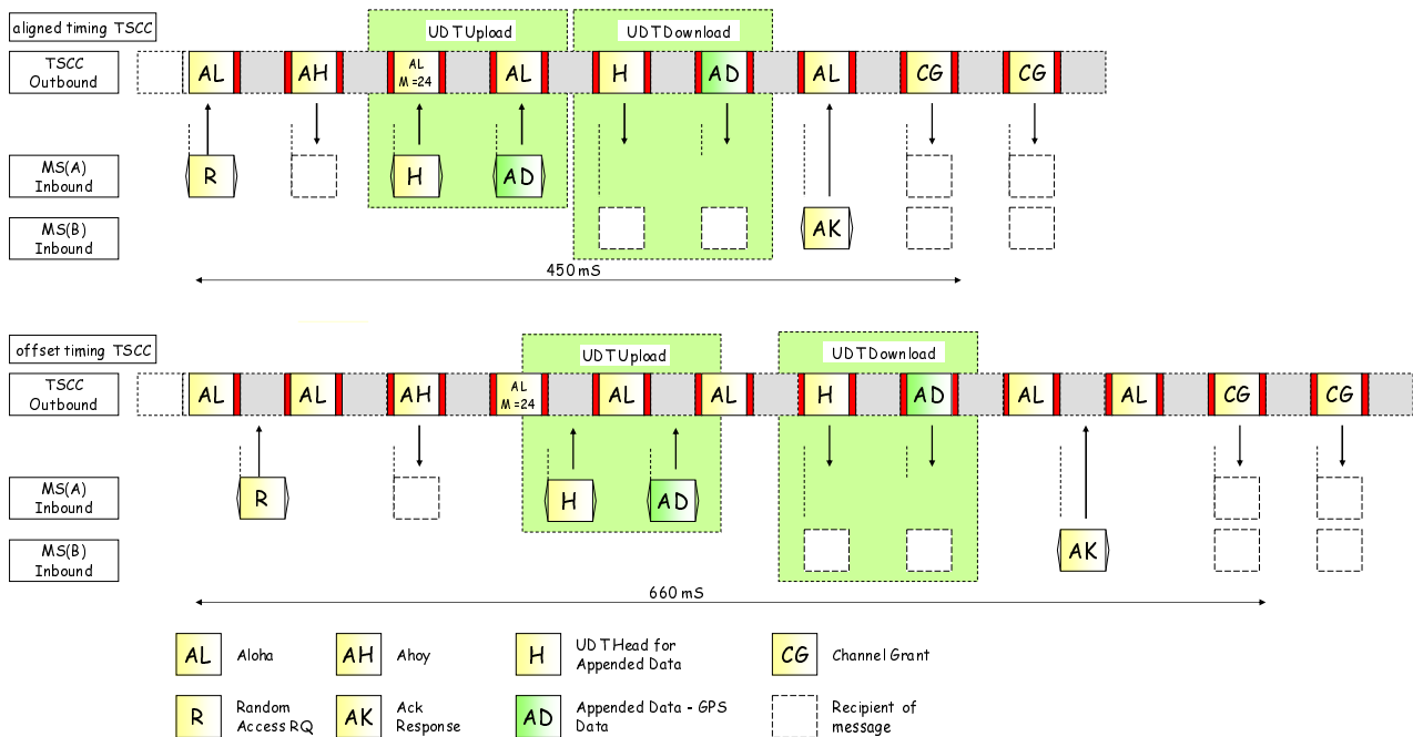
Figure 6.46: UDT Mechanism carrying Supplementary Data
