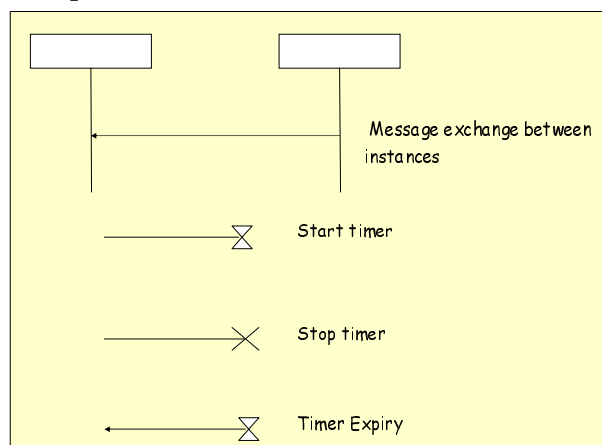
Figure F.1: SDL Notation
