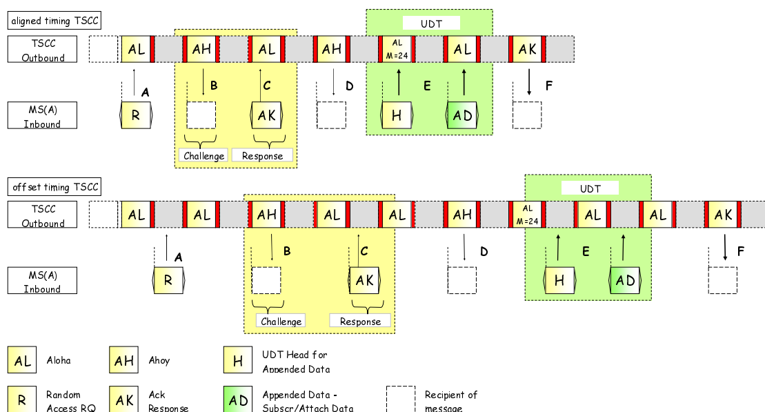
Figure 6.27: Authentication and Talkgroup List Subscription/Attachment
