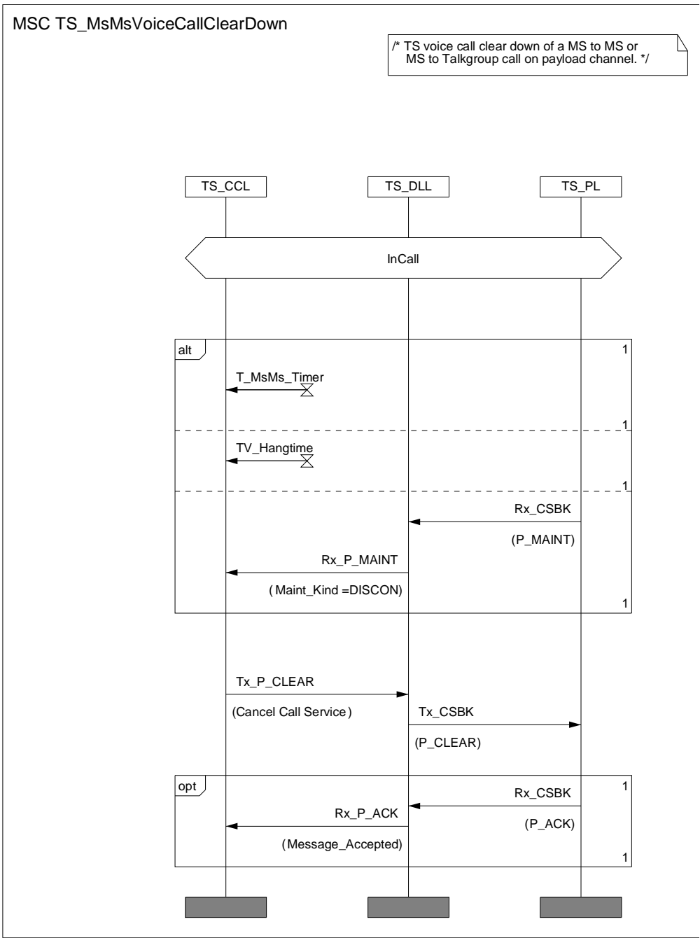
Figure 6.56: Voice Call Termination MSC
