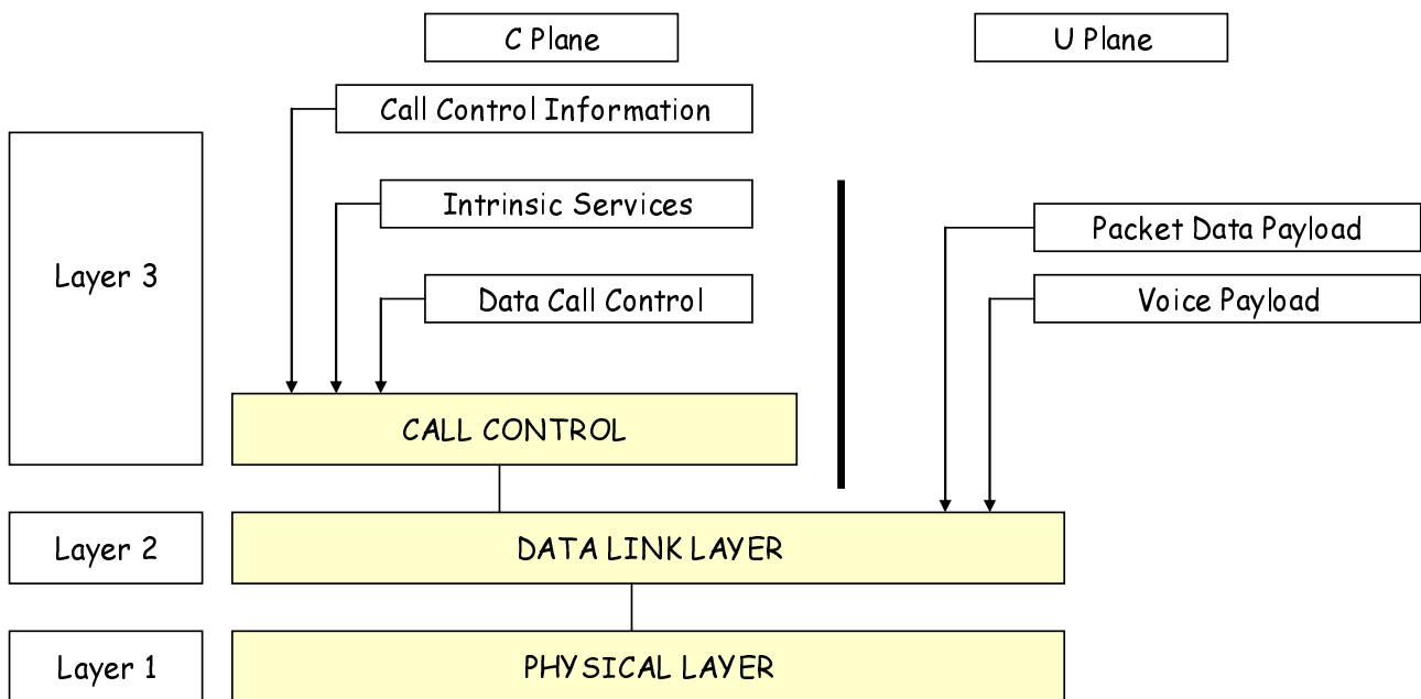
Figure 4.1: DMR protocol stack
