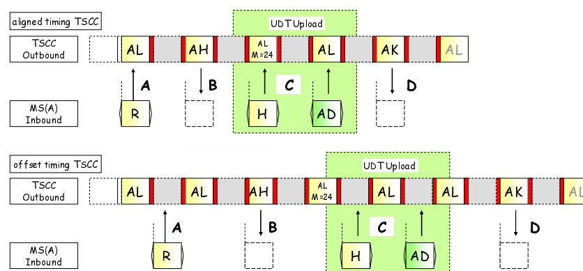
Figure 6.34: MS IP Connection Advice
