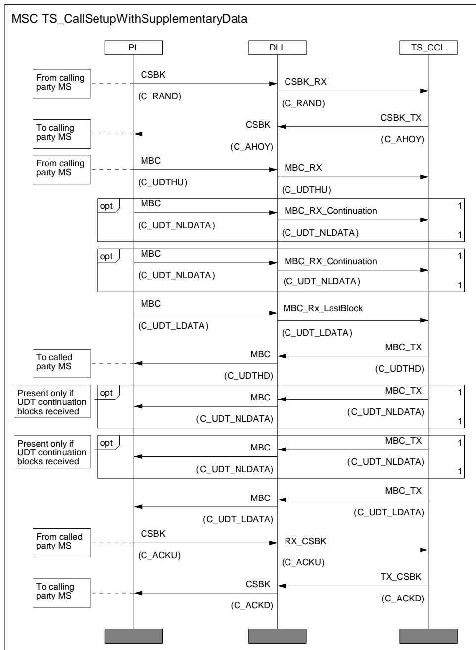
Figure 6.55: MS OACSU Call Set-up with Supplementary Data
