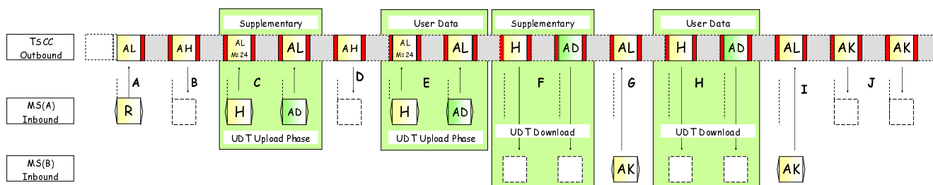
Figure 6.39: UDT mechanism Carrying Supplementary User Data for a UDT Short Data Call
