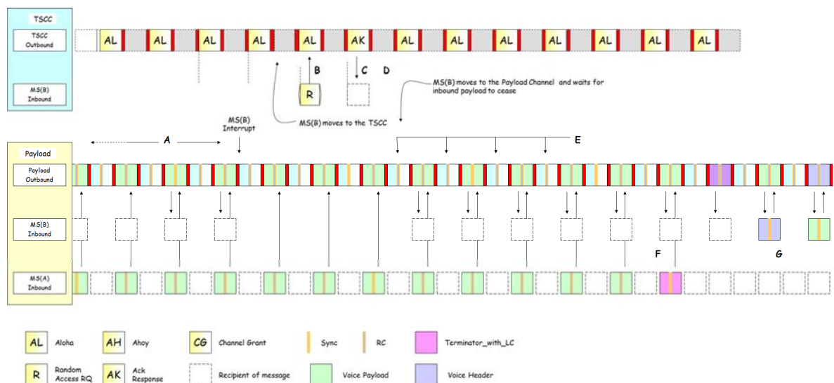
Figure 6.40: Payload Interrupt MS De-key
