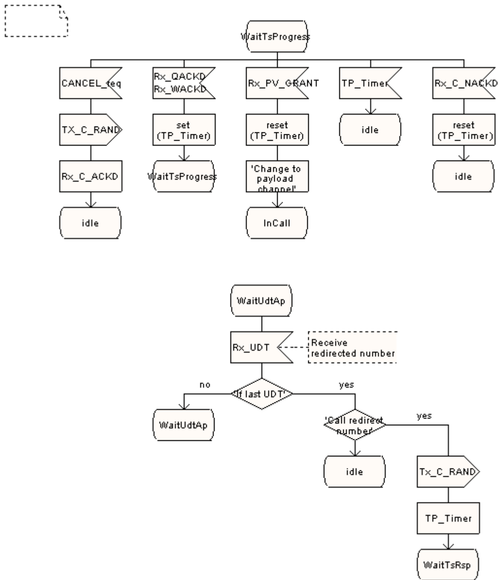
Figure 6.54 (sheet 2 of 2): Single Part OACSU Voice Call Setup SDL
