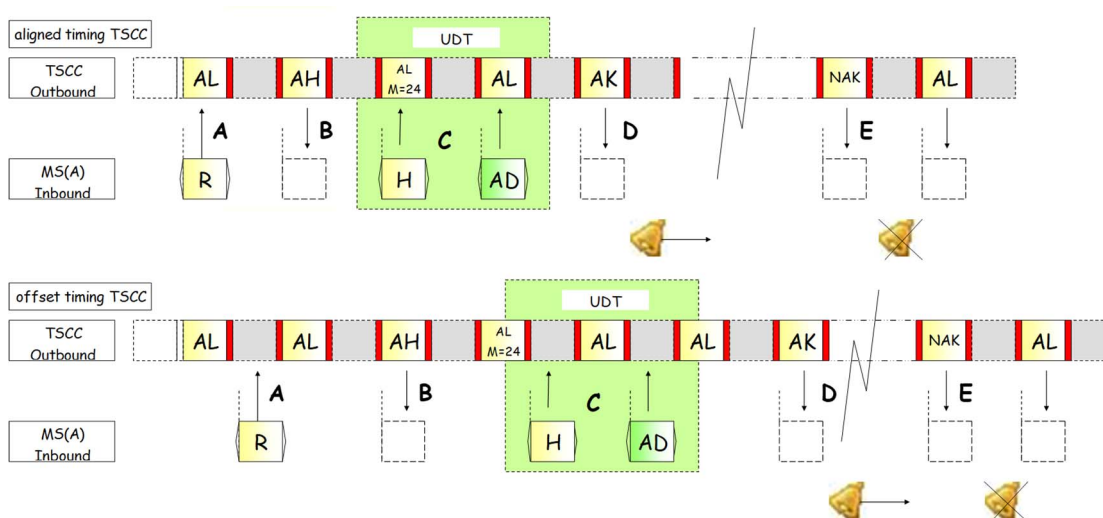
Figure 6.50: Example of Multi-part Call Procedure (Local Ringing Call is Refused)
