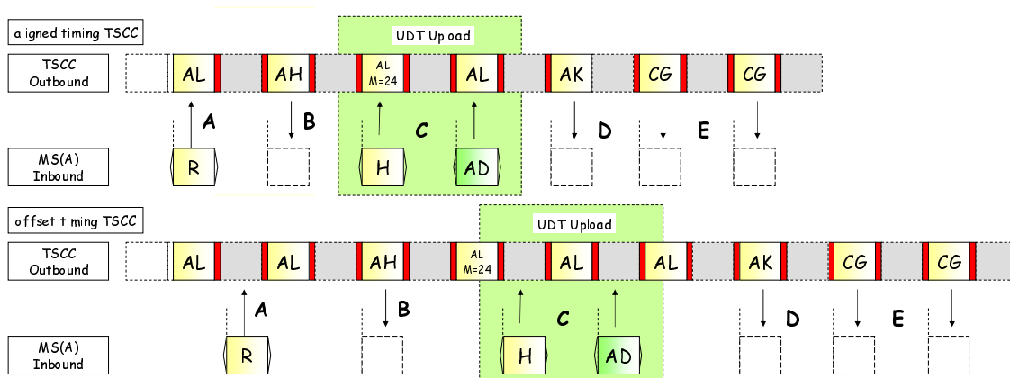
Figure 6.47: Example of Multi-part Call Procedure In Band Ringing (Call Accepted)
