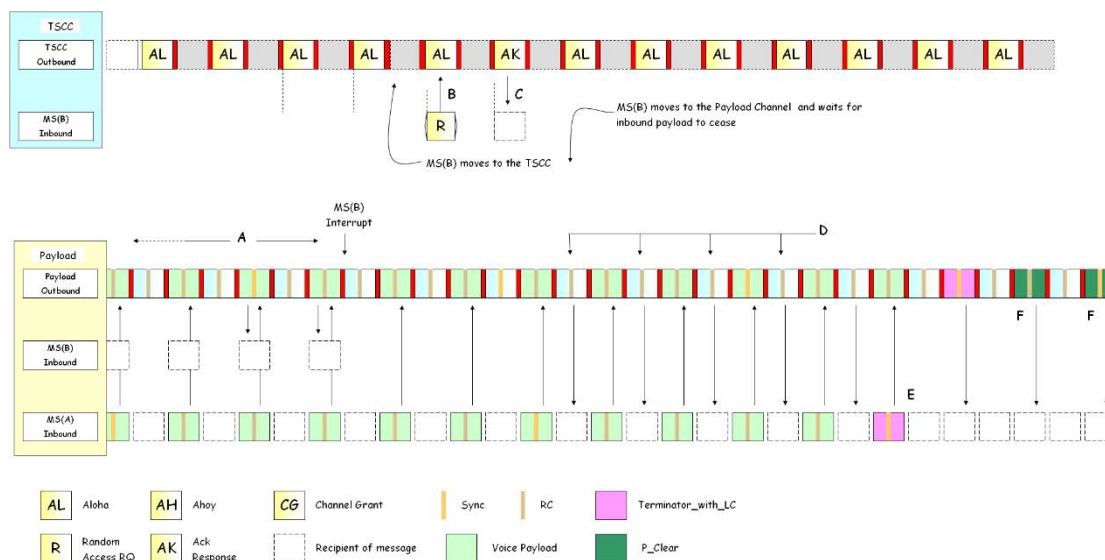
Figure 6.41: Ambient Listening Service MS De-key
