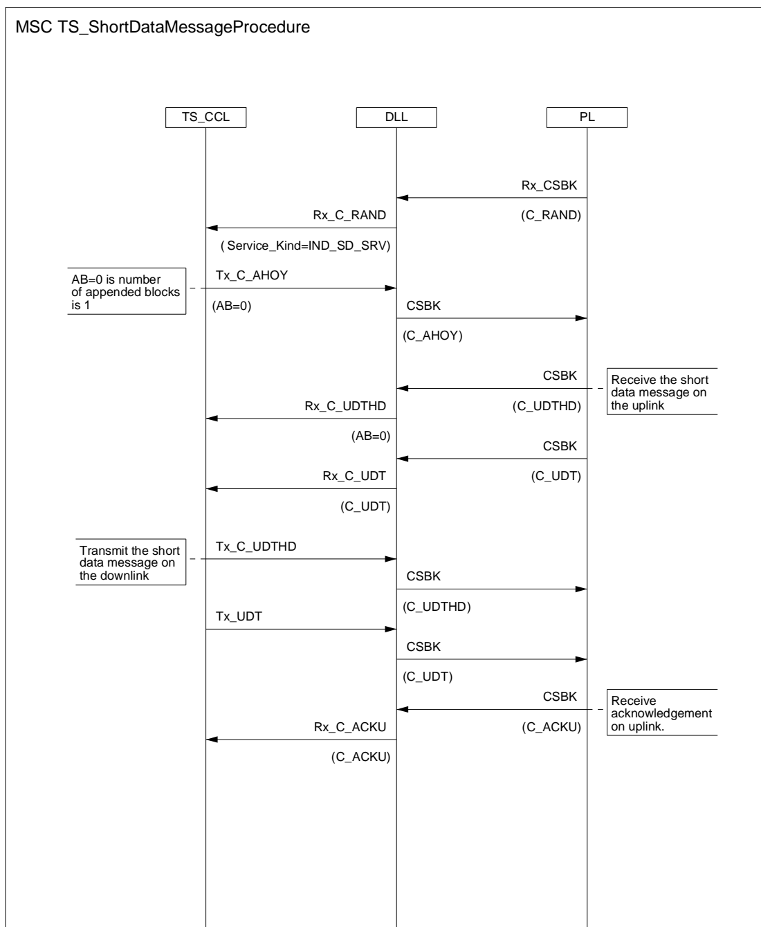
Figure 6.59: UDT Short Data Message MSC
