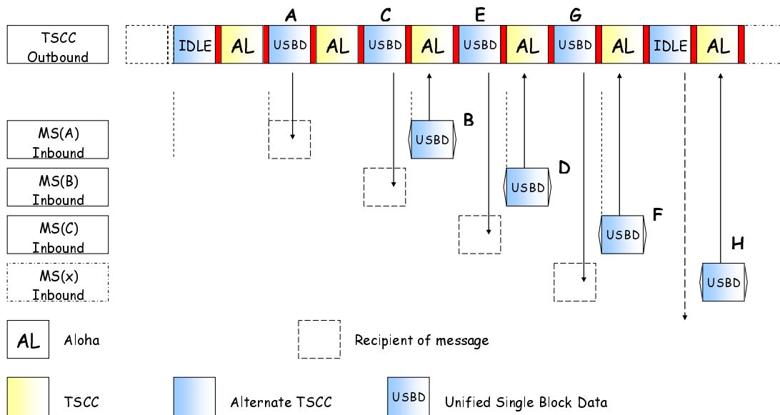
Figure 6.69: Example of Unified Single Block Data Polling Service on TSCCAS using Offset Timing (Response Delay = 00_2 )
