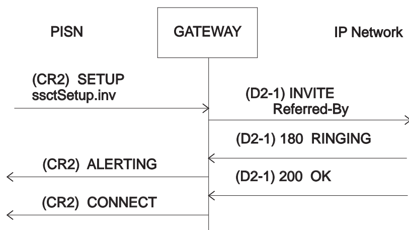
Figure 6: Example of message flows on receipt of a SETUP message with ssctSetup invoke APDU
