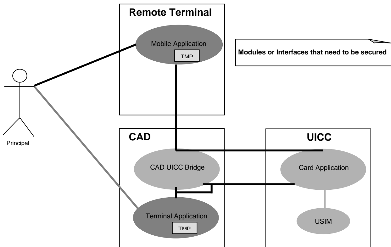
Figure 4: Distributed application
