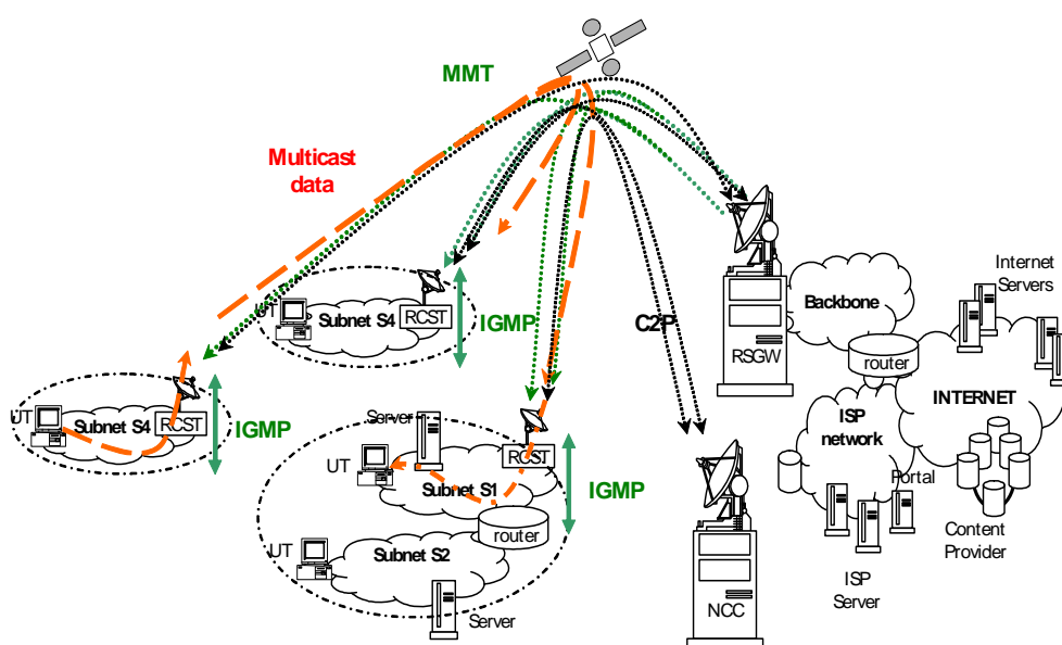
Figure E.2.4: Mesh IP multicast network topology
