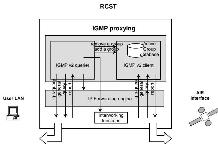
Figure E.2.2: IGMP proxying overview
