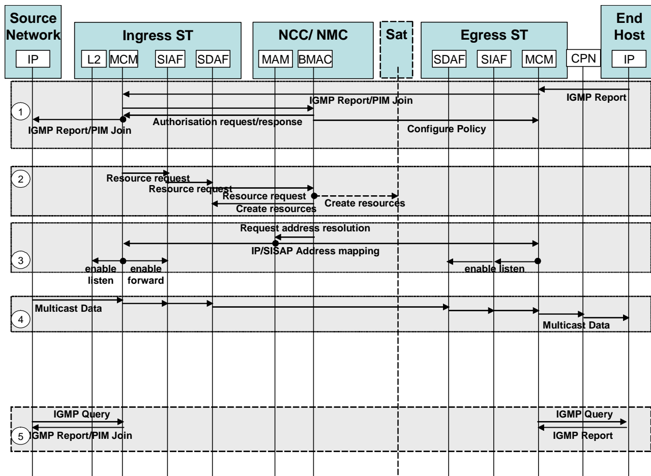
Figure 7.2: Star Pull Scenario Messages
