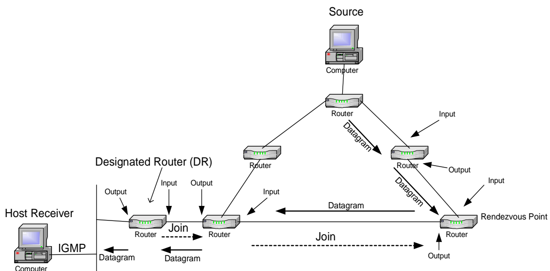
Figure D.4.3: PIM-SM Message Input/Output Convention
