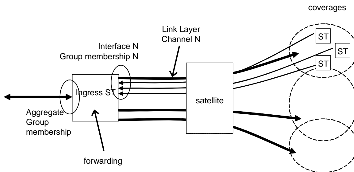
Figure 6.3: Forwarding and PIM join/prune or IGMP reporting scheme
