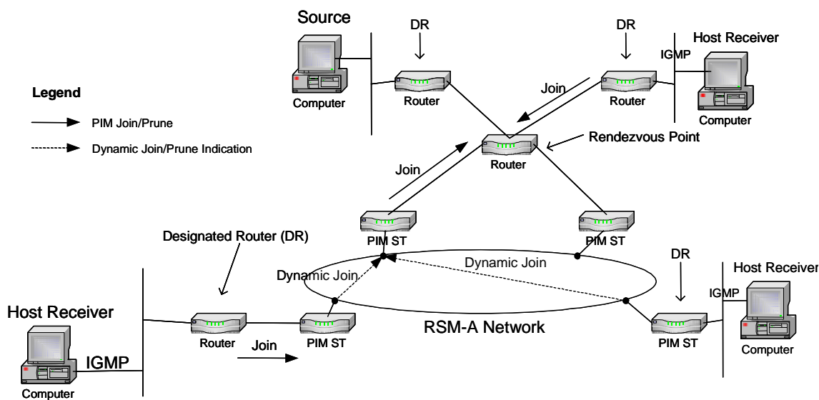
Figure D.5.1: Multicast Delivery Tree Establishment
