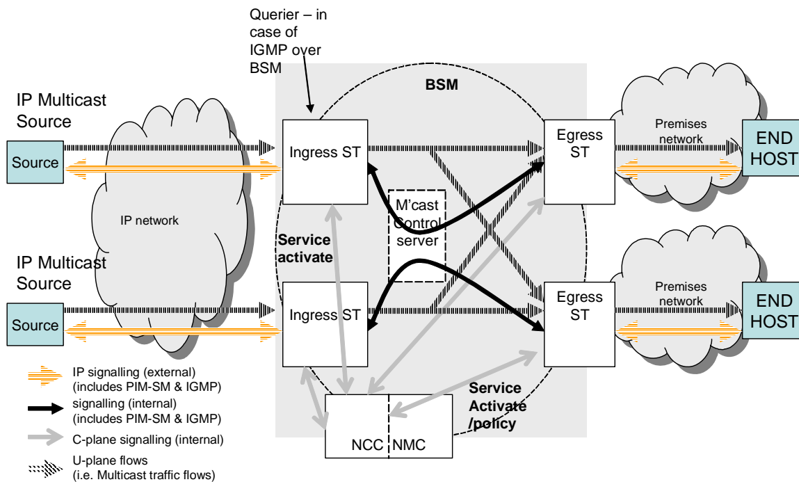
Figure 3.4: Mesh Pull Scenario
