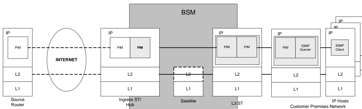
Figure 5.8: PIM-over-BSM Architecture with PIM external to STs
