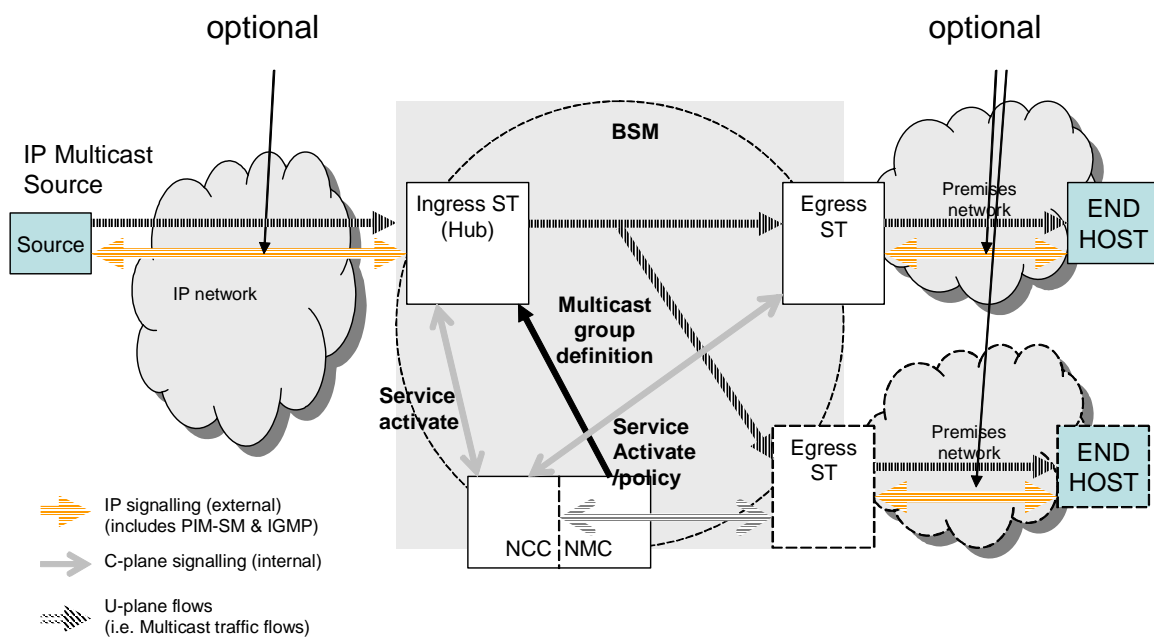
Figure 3.1: Star Push Scenario
