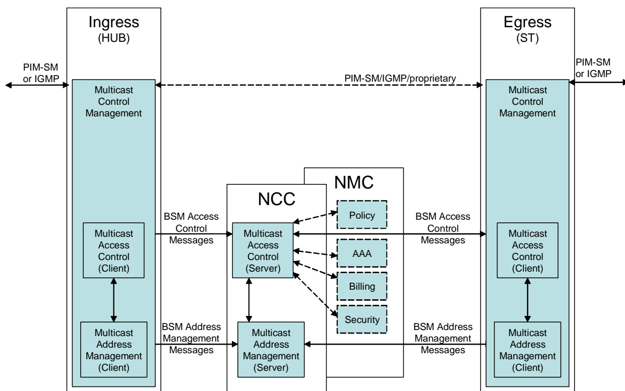
Figure 5.2: BSM Multicast Source Management Control Plane Architecture (Star Pull)
