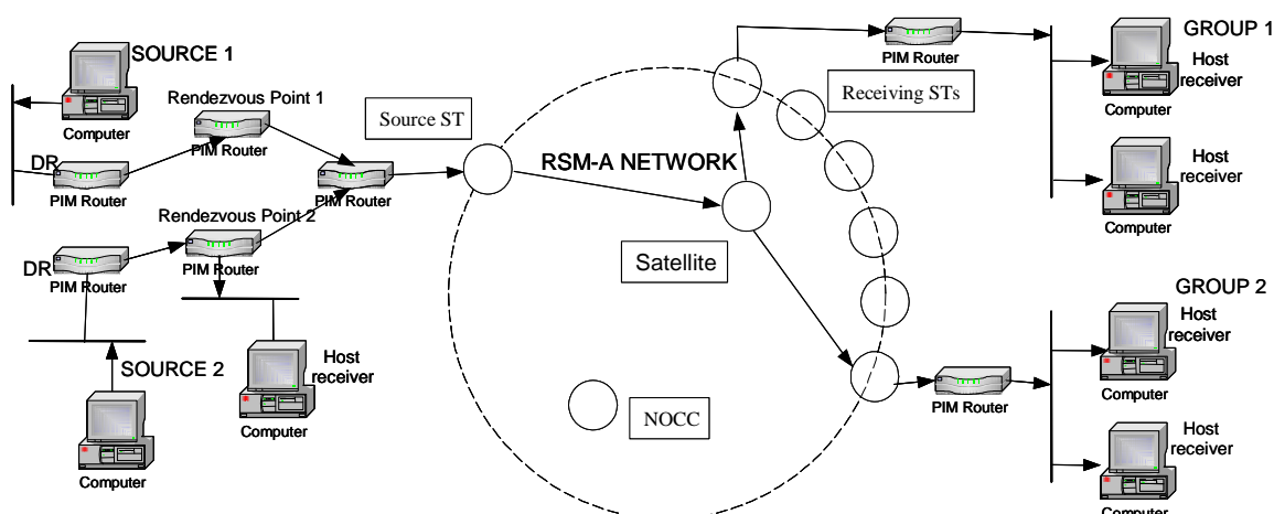
Figure D.5.2: Multicast Datagram Forwarding in RSM-A using PIM-SM STs
