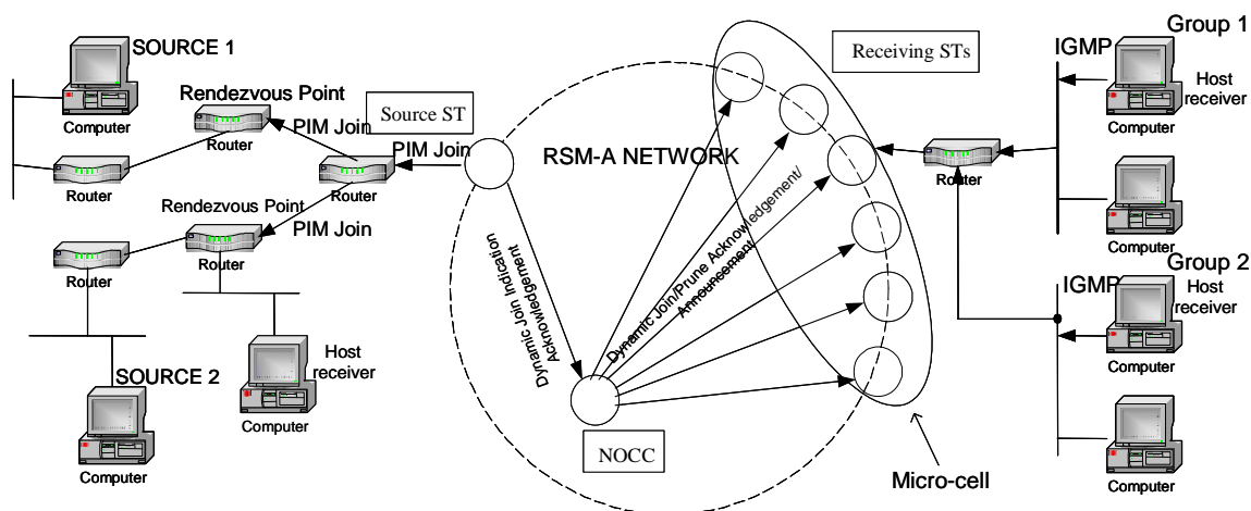
Figure D.4.5: RSM-A Dynamic Join/Prune Acknowledgement
