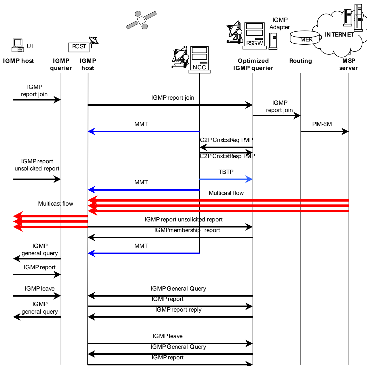
Figure E.2.3: Star IP Multicast scenario example
