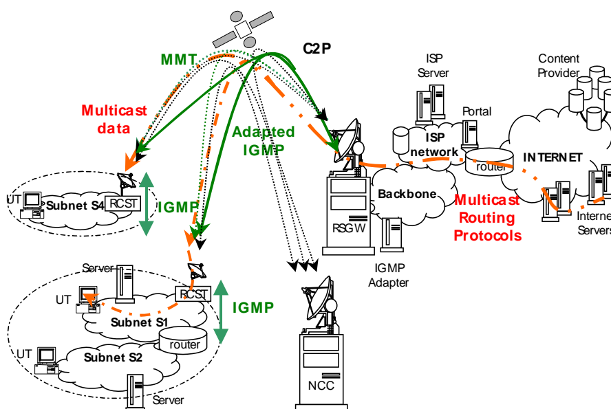
Figure E.2.1: RSM-B Star IP dynamic multicast
