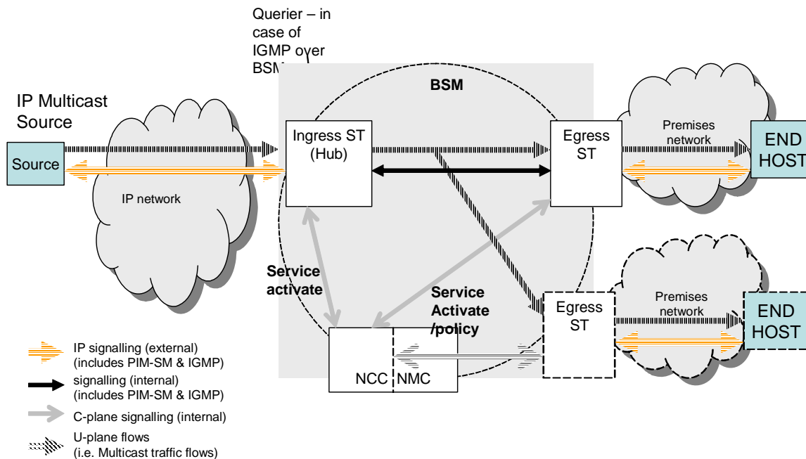
Figure 3.2: Star Pull Scenario
