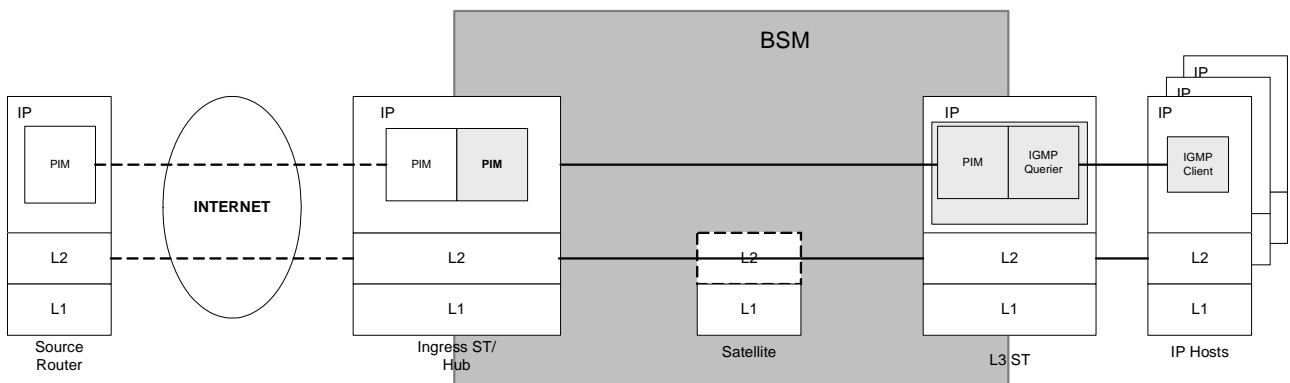
Figure 5.7: PIM-over-BSM Architecture with PIM external to Ingress and IGMP external to Egress STs
