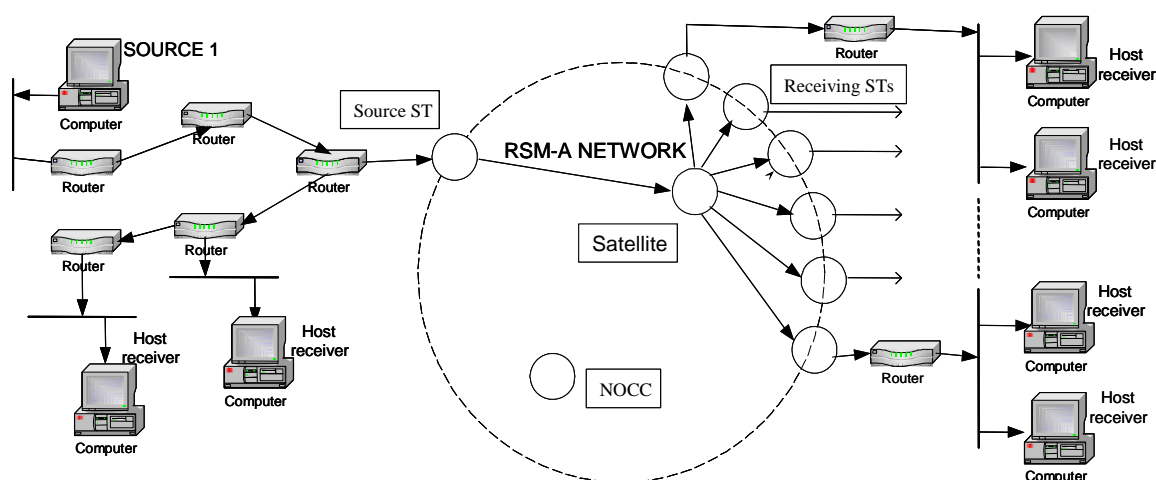
Figure D.4.2: On-demand Static Multicast Traffic over RSM-A
