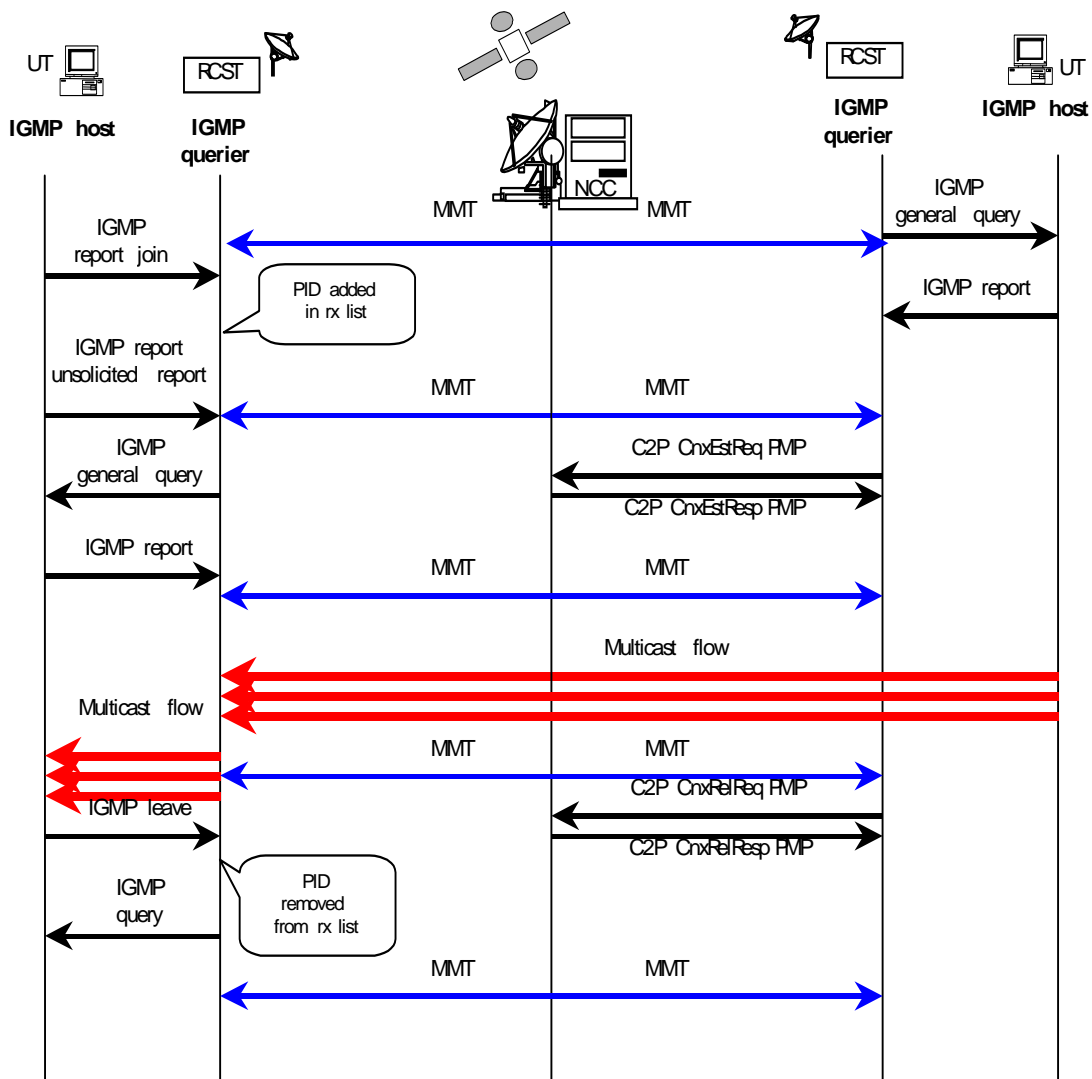
Figure E.2.6: Mesh IP Multicast scenario example
