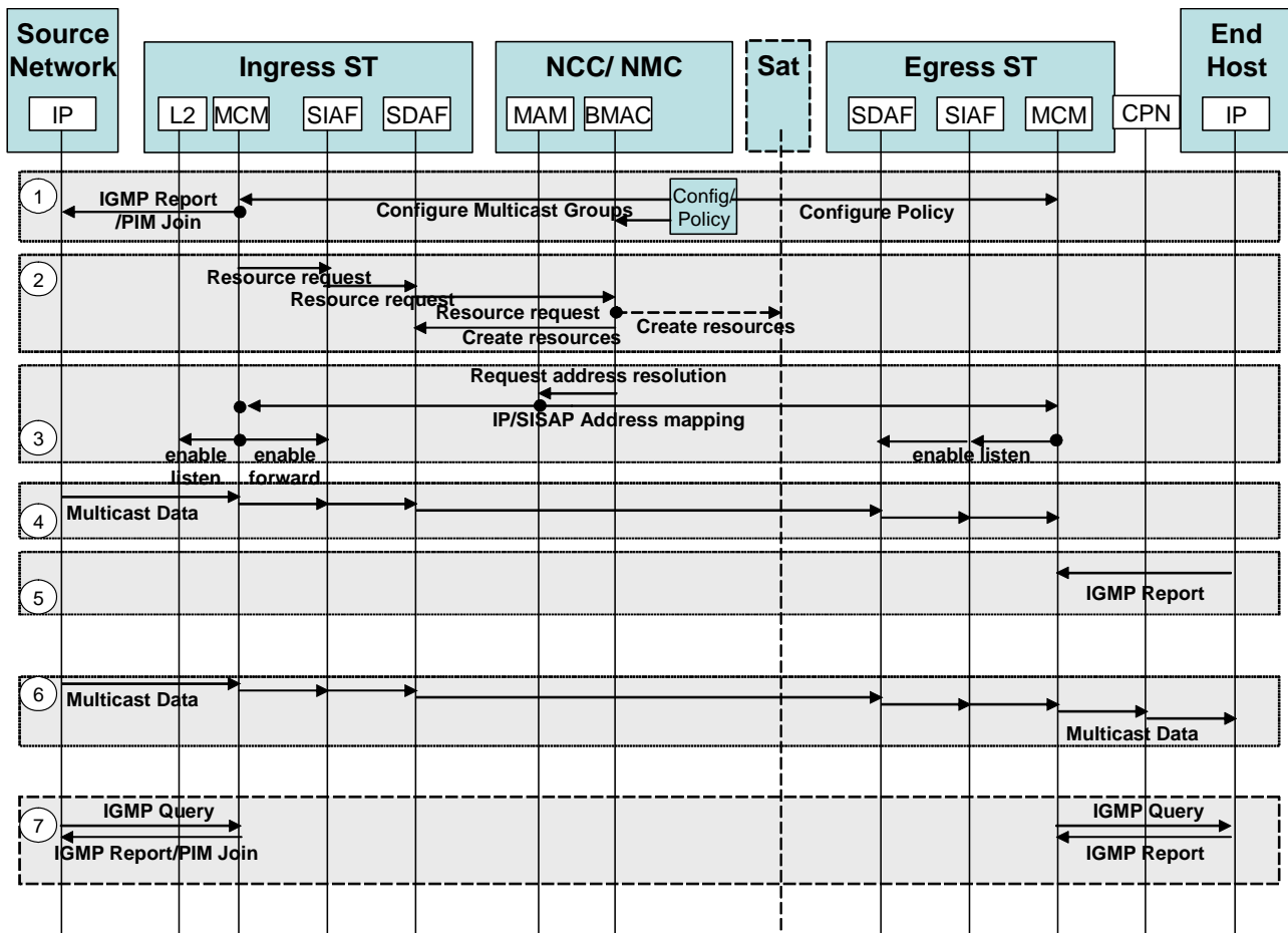
Figure 7.1: Push Scenario Messages
