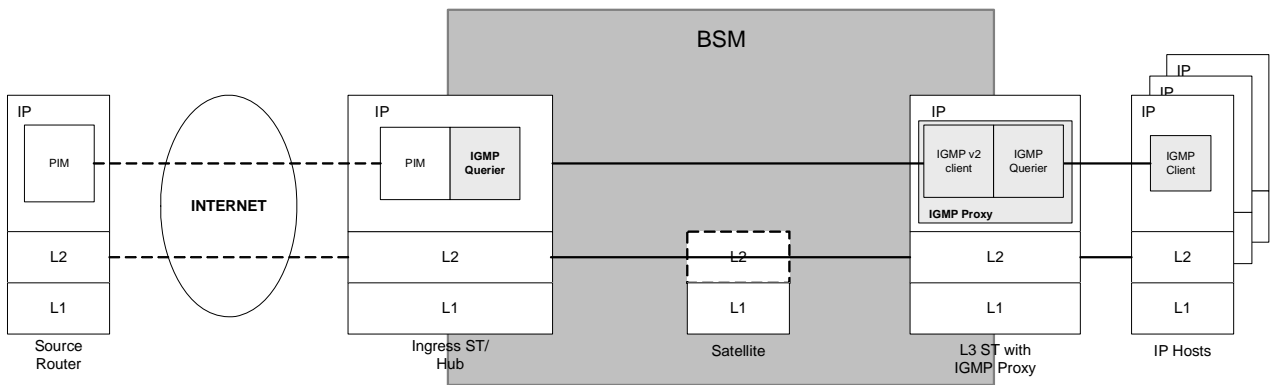
Figure 5.5: IGMP-over-BSM Architecture with Egress ST Layer 3 Forwarding
