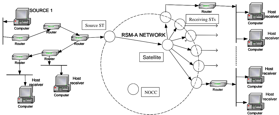
Figure D.3.2: Scheduled Multicast Traffic over RSM-A
