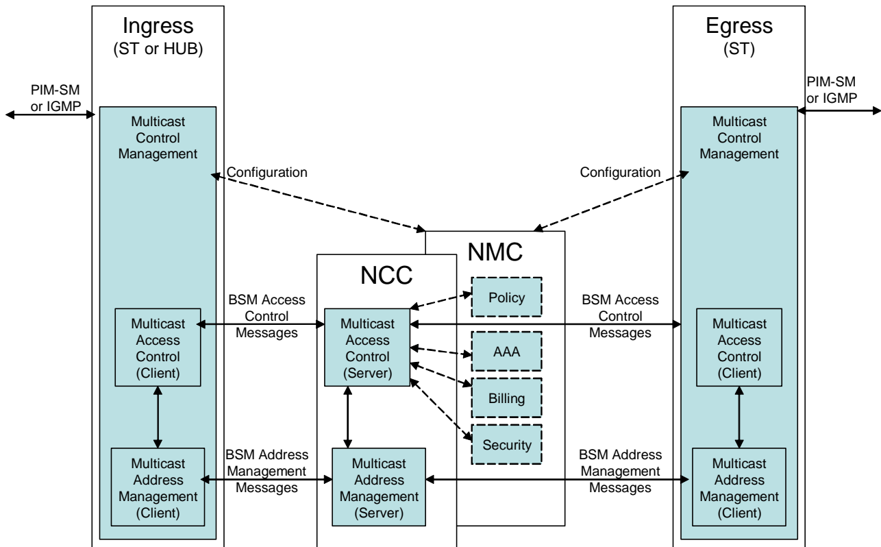
Figure 5.1: BSM Multicast Source Management Control Plane Architecture (Star and Mesh Push)
