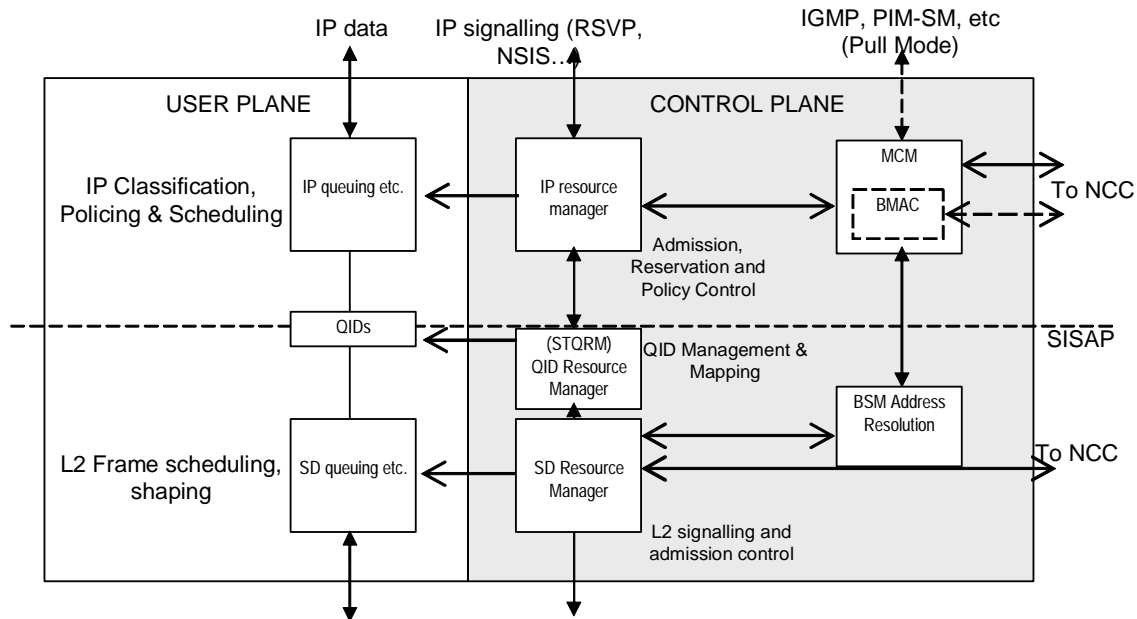
Figure 5.9: Ingress ST multicast resource management functional relationships
