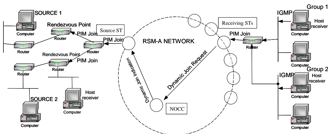
Figure D.4.4: RSM-A Dynamic Join
