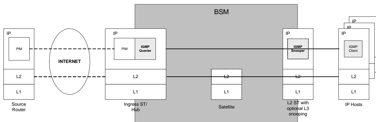
Figure 5.4: IGMP-over-BSM Architecture with Egress ST Layer 2 (Switching) and optional IGMP snooping
