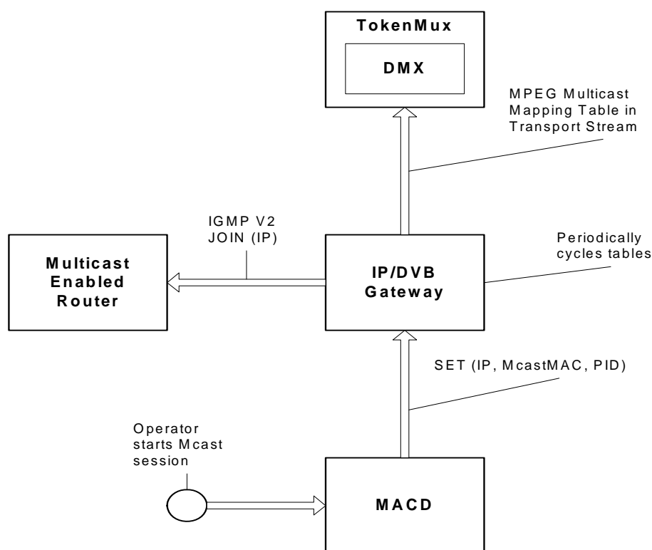
Figure C.4.2: Invoking a multicast receive session: Hub side
