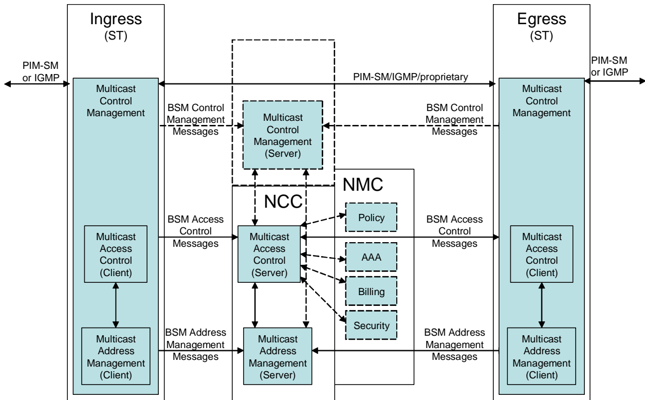
Figure 5.3: BSM Multicast Source Management Control Plane Architecture (Mesh Pull case)
