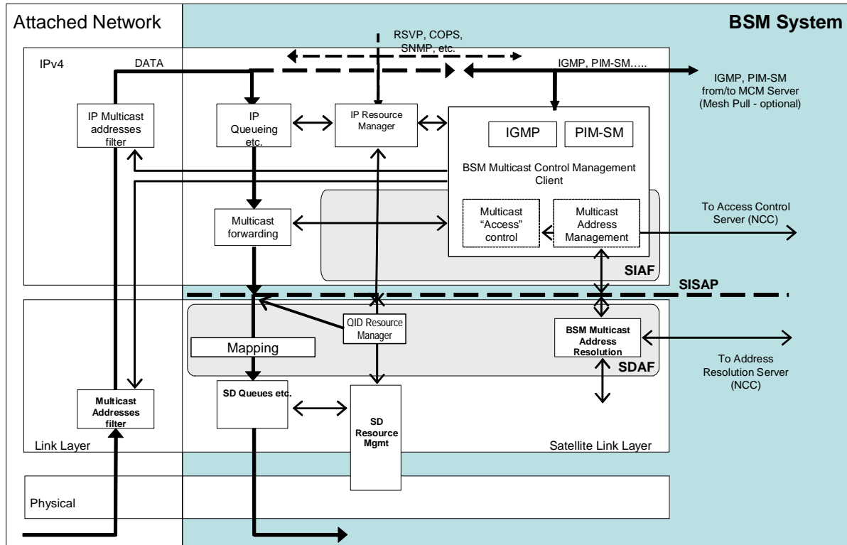
Figure 6.1: BSM Multicast Ingress ST protocol stack
