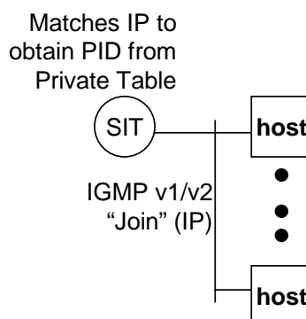
Figure C.4.1: Invoking a multicast receive session: SIT side
