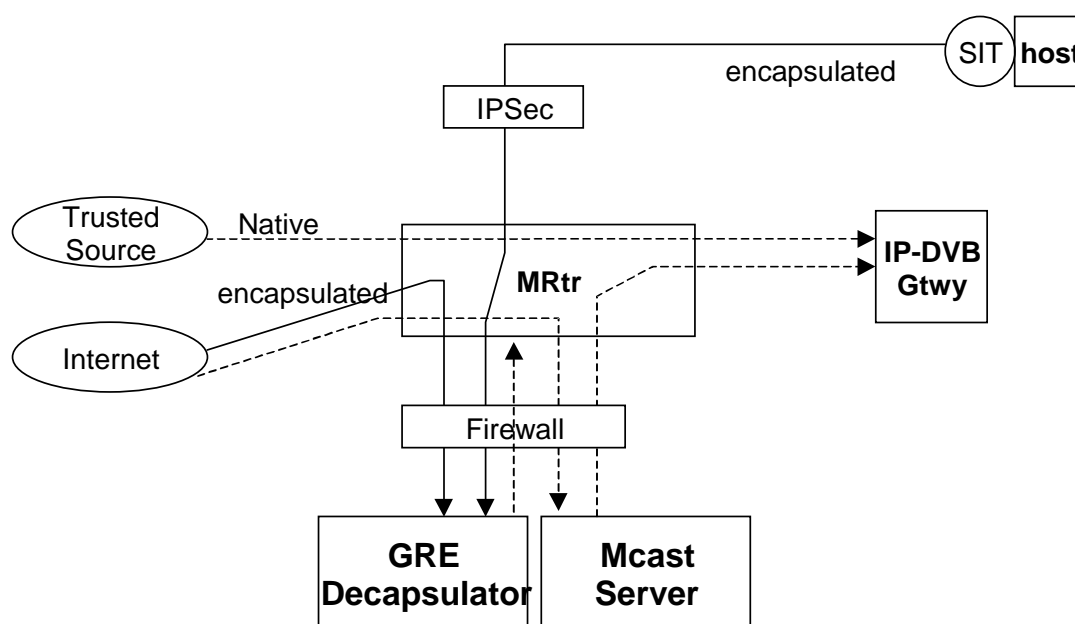
Figure C.5.1: Multicast source transmission model
