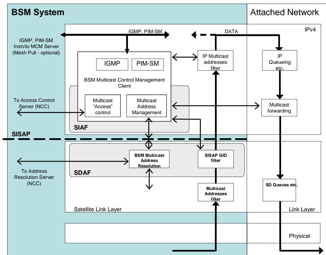
Figure 6.2: BSM Multicast Egress ST protocol stack
