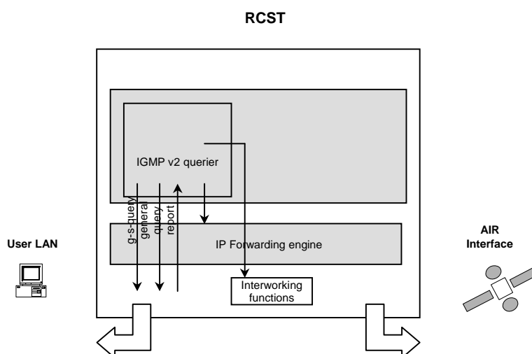
Figure E.2.5: IGMPv2 querier overview
