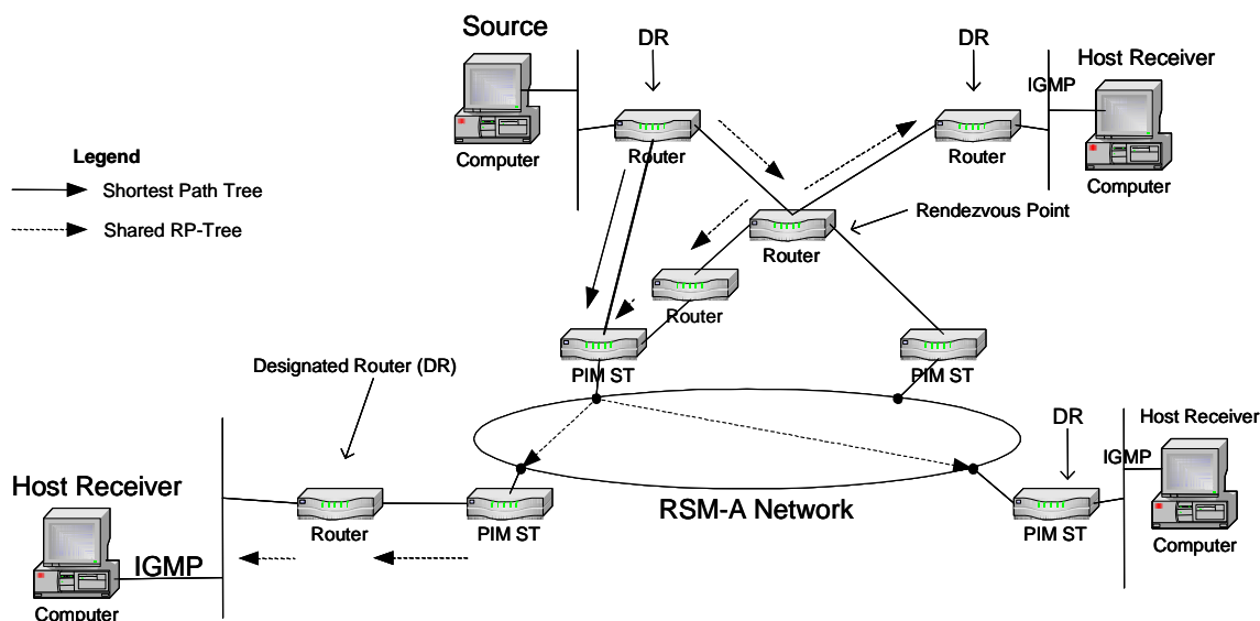
Figure D.5.3: PIM-SM - Switching to Shortest Path Tree
