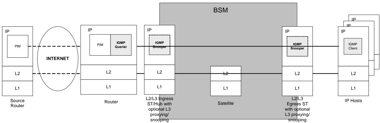
Figure 5.6: IGMP-over-BSM Architecture with IGMP external to BSM and optional IGMP proxying or snooping at Ingress and Egress
