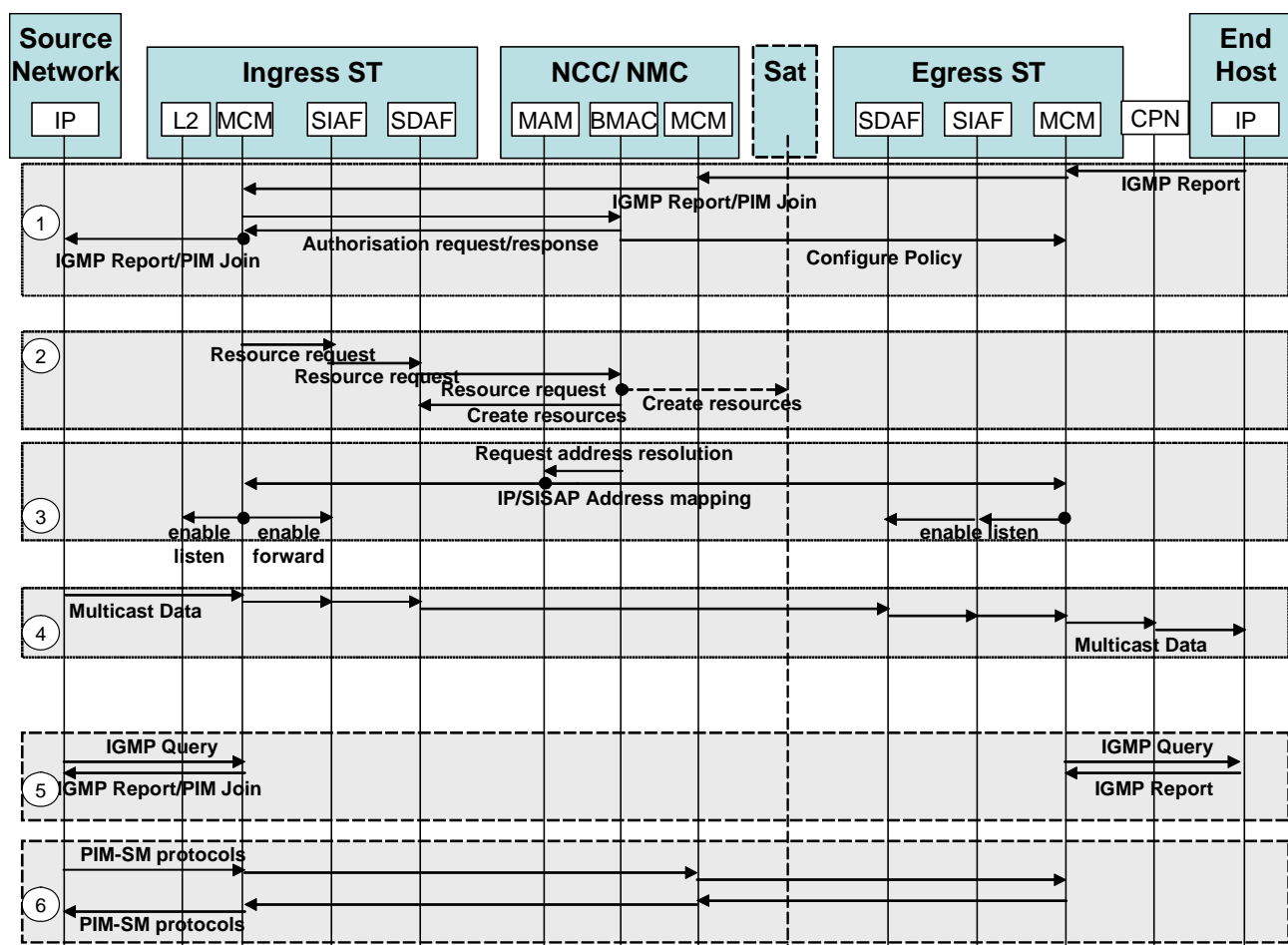
Figure 7.3: Mesh Pull Scenario Messages
