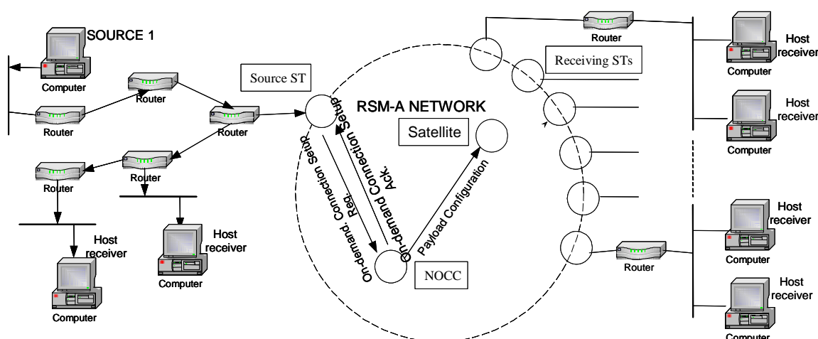
Figure D.4.1: On-demand Multicast Connection Setup
