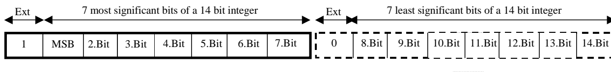
Figure 3.1: Informative example for the vluimsbf8 data type
