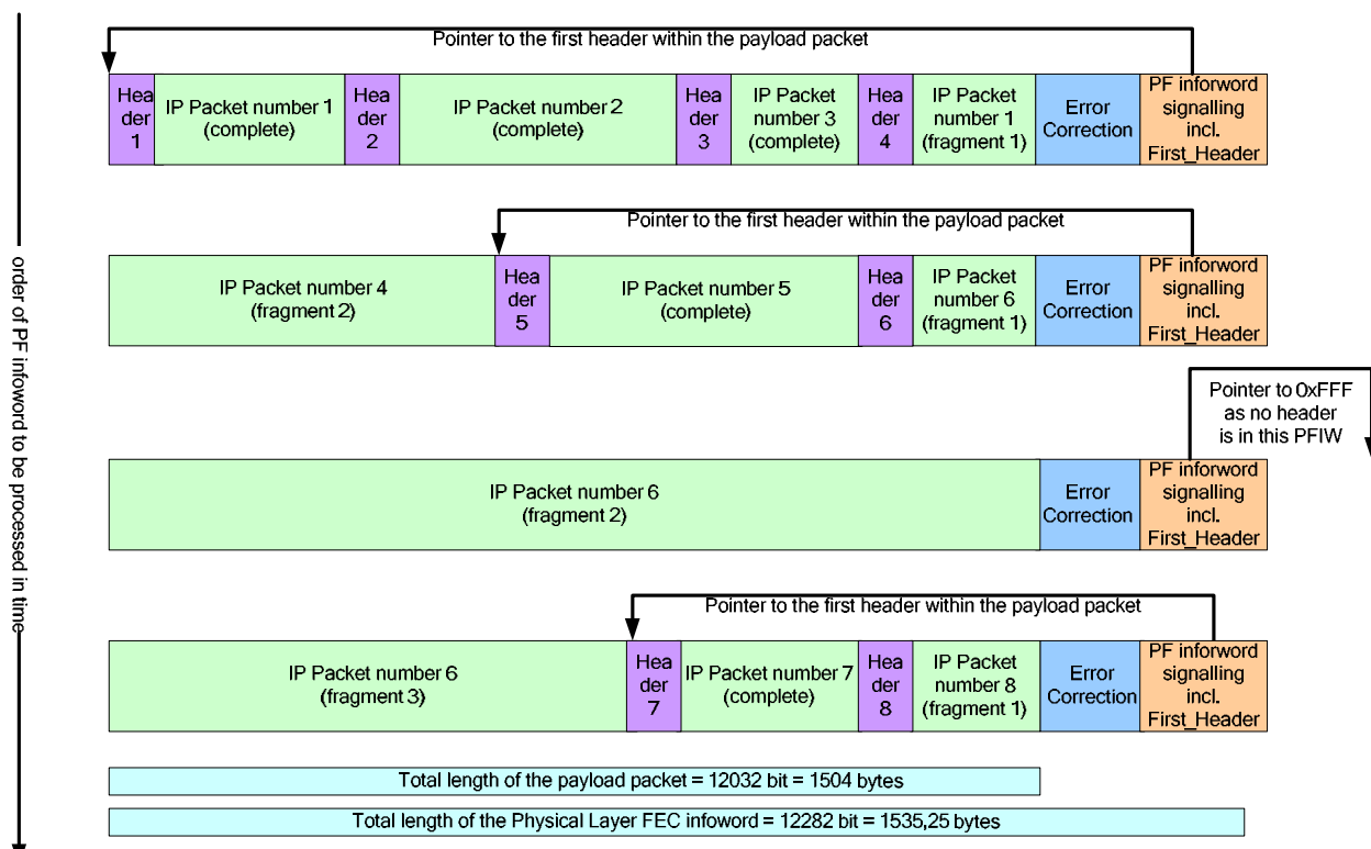
Figure 3: Description of IP packet encapsulation
