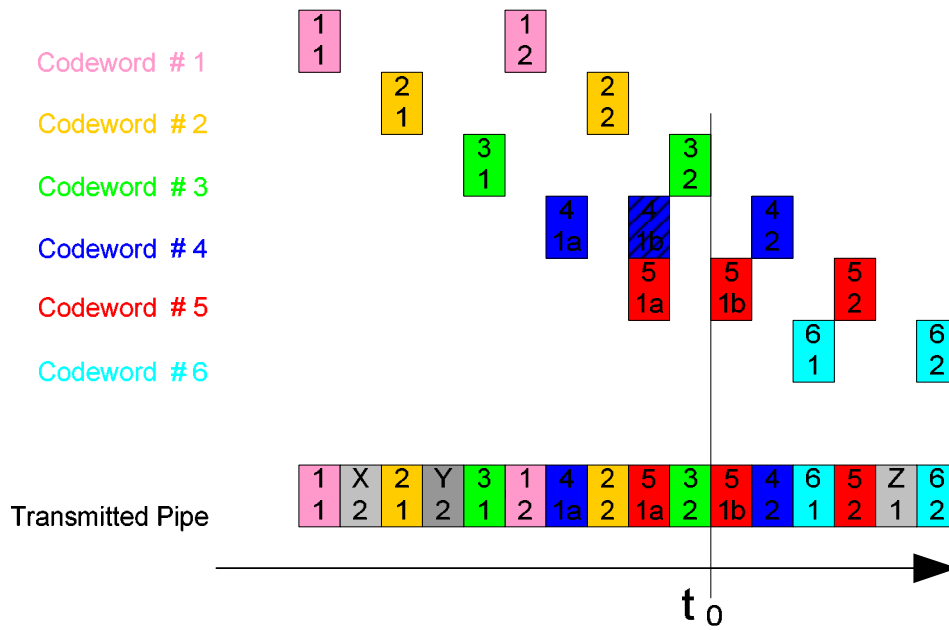
Figure 9: Shorter disperser delay after reconfiguration
