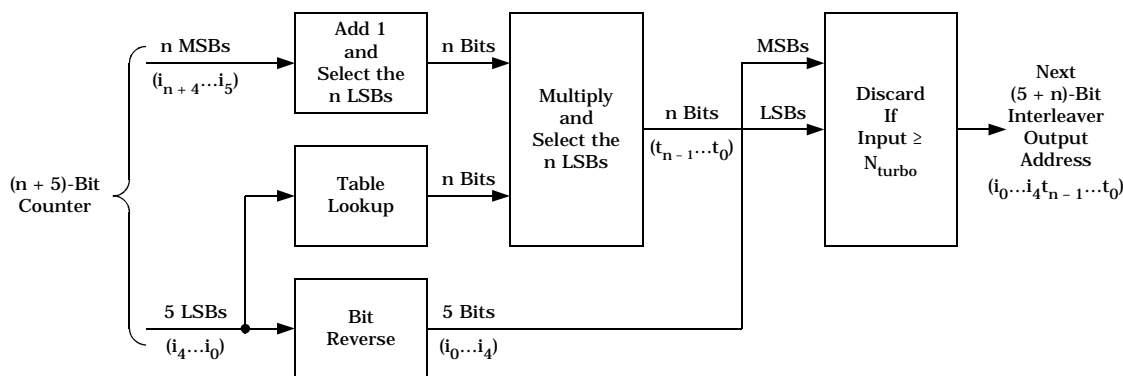
Figure 5: Turbo interleaver output address calculation procedure
