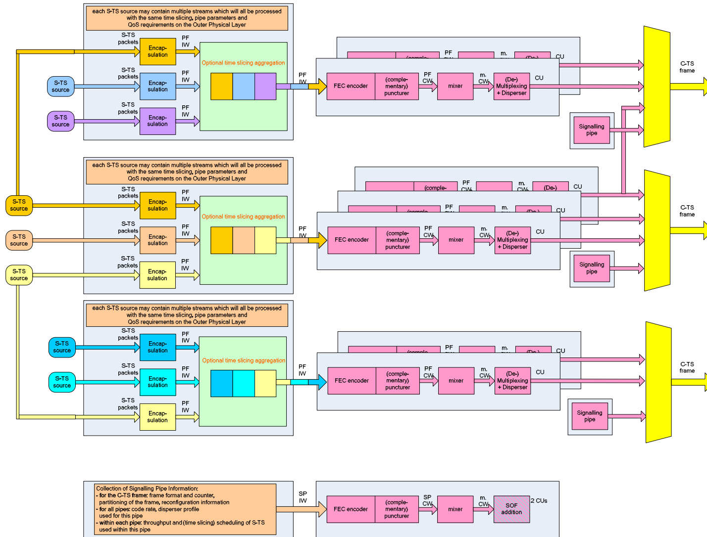
Figure 1: General overview of the OPL functionality
