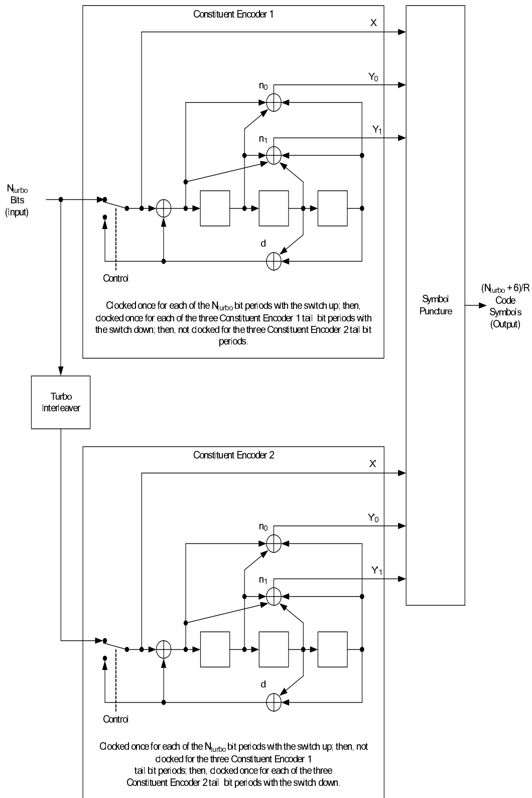
Figure 4: Turbo encoder
