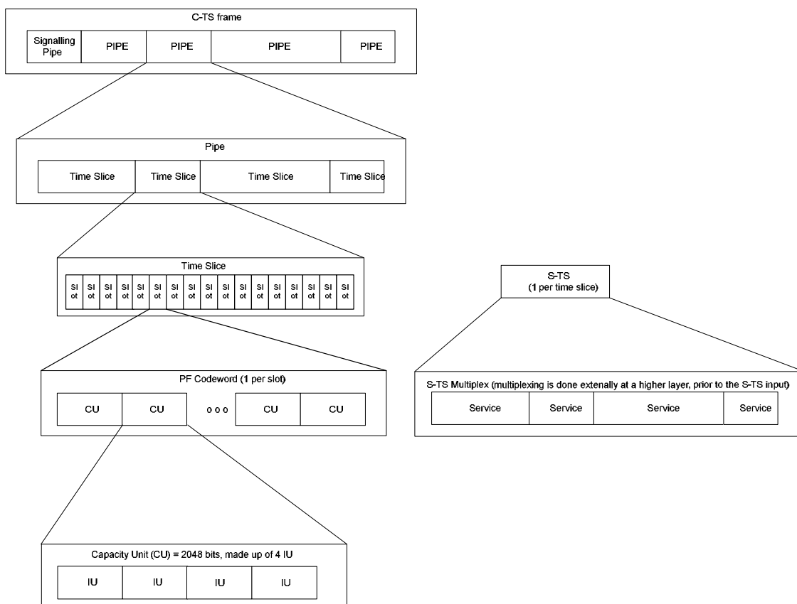
Figure 8: Overview on the C-TS multiplex
