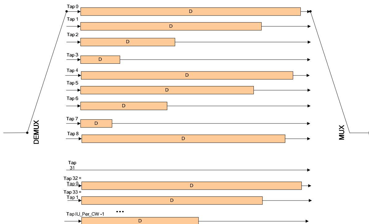
Figure 6: Example of a disperser profile
