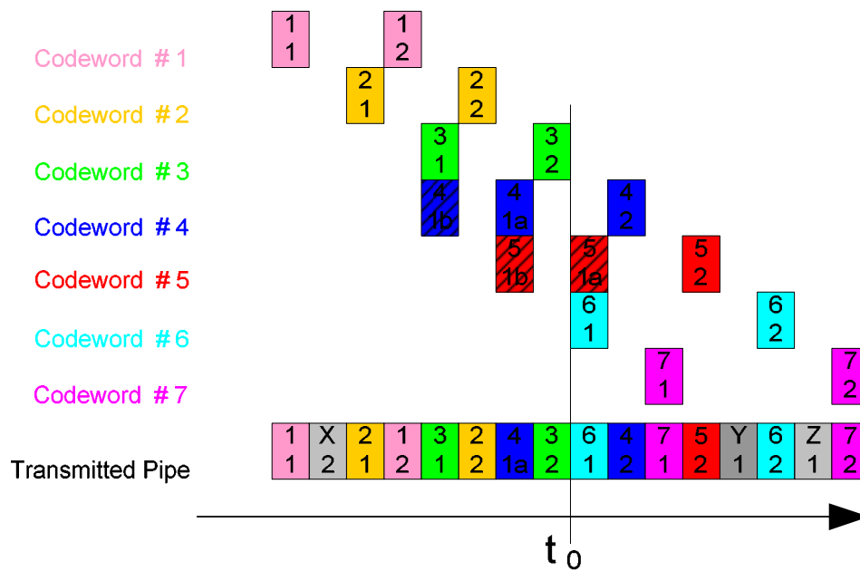
Figure 10: Longer disperser delay after reconfiguration
