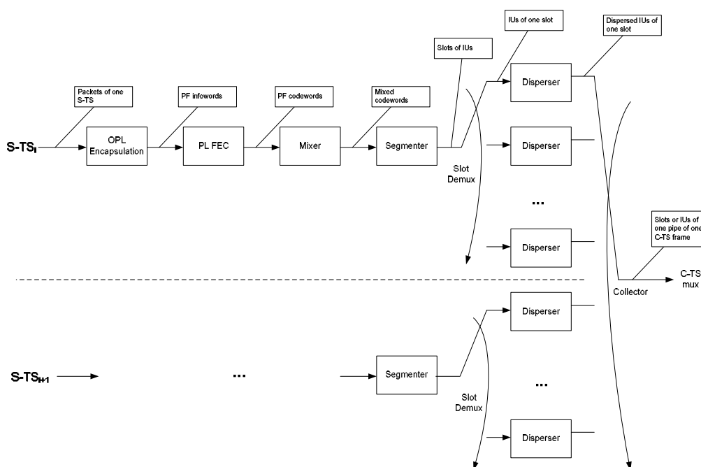
Figure 2: Definition of the different blocks involved in the OPL processing
