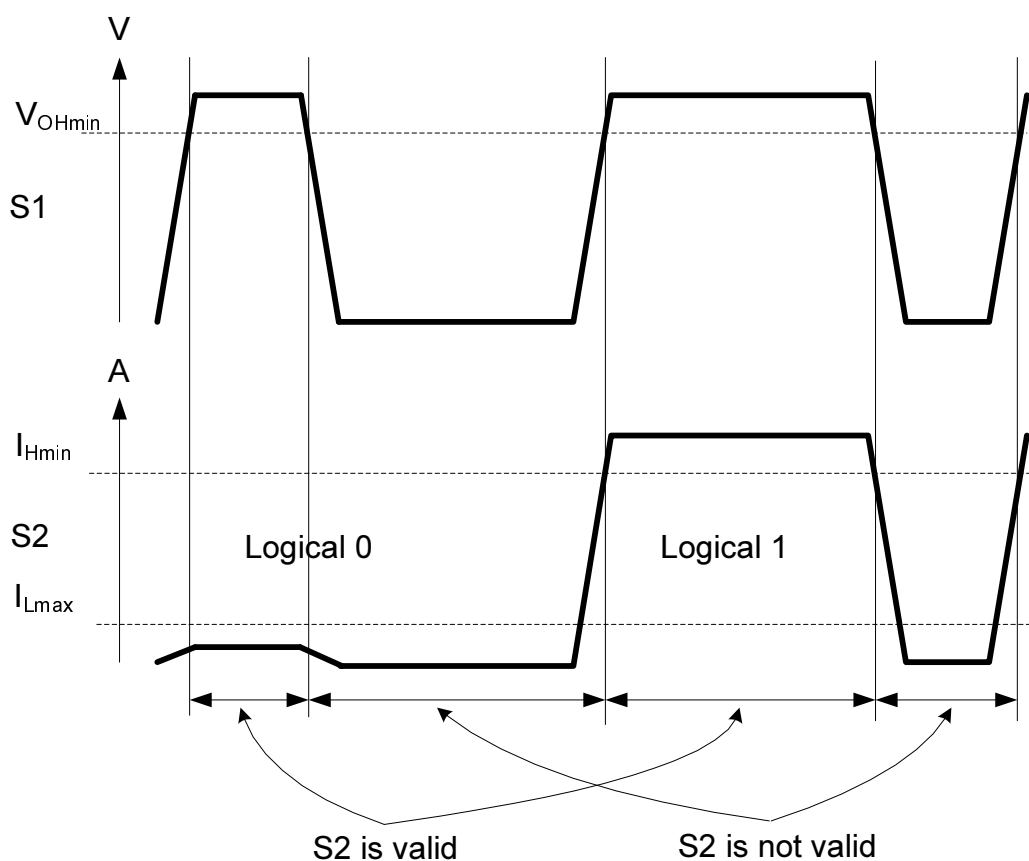
Figure 8.3: S2 timing
