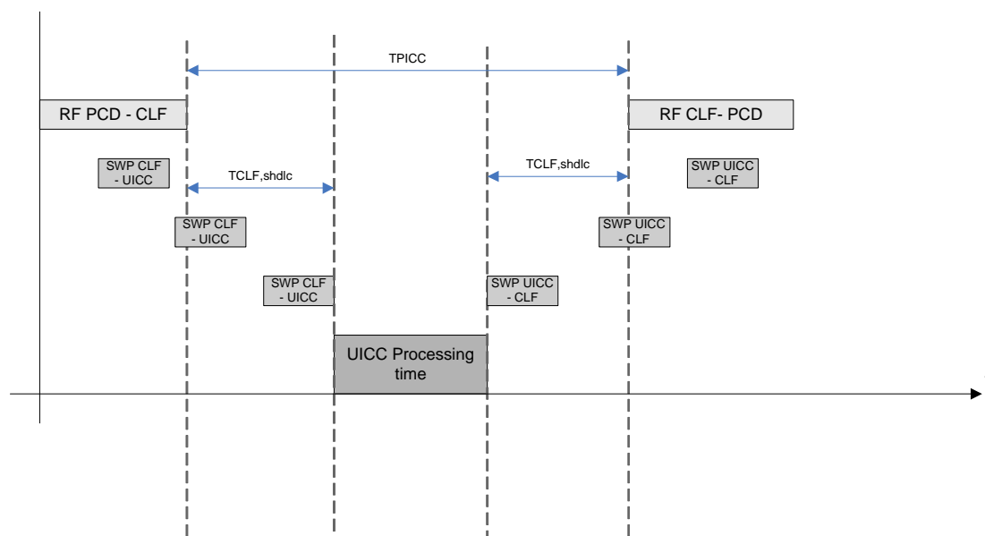
Figure 12.1: SHDLCL transmission timings
