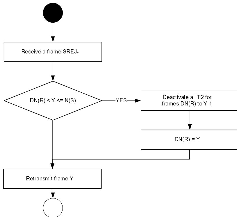
Figure 10.23: SREJ frame reception
