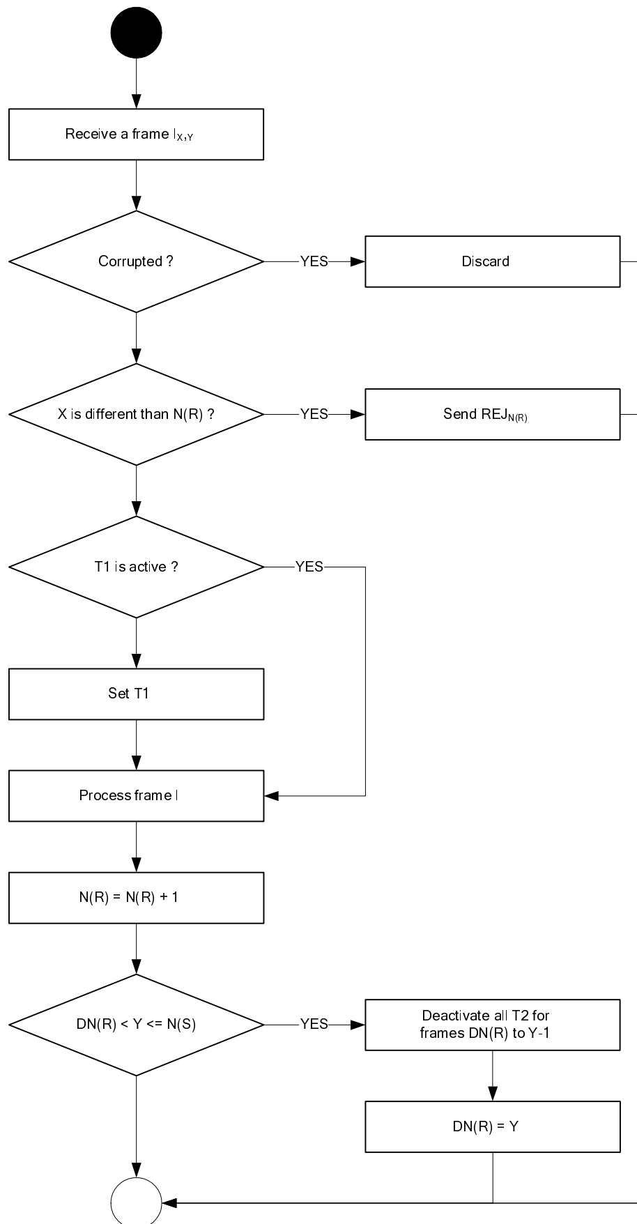
Figure 10.20: Information frame reception
