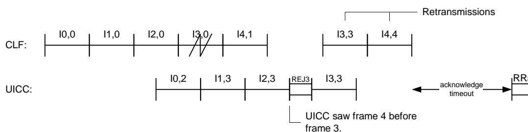
Figure 10.14: Piggybacking with reject frame after mismatching sequence number
