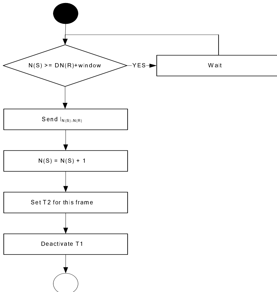
Figure 10.19: Information frame emission.
