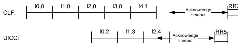
Figure 10.13: Piggybacking and timed acknowledgement
