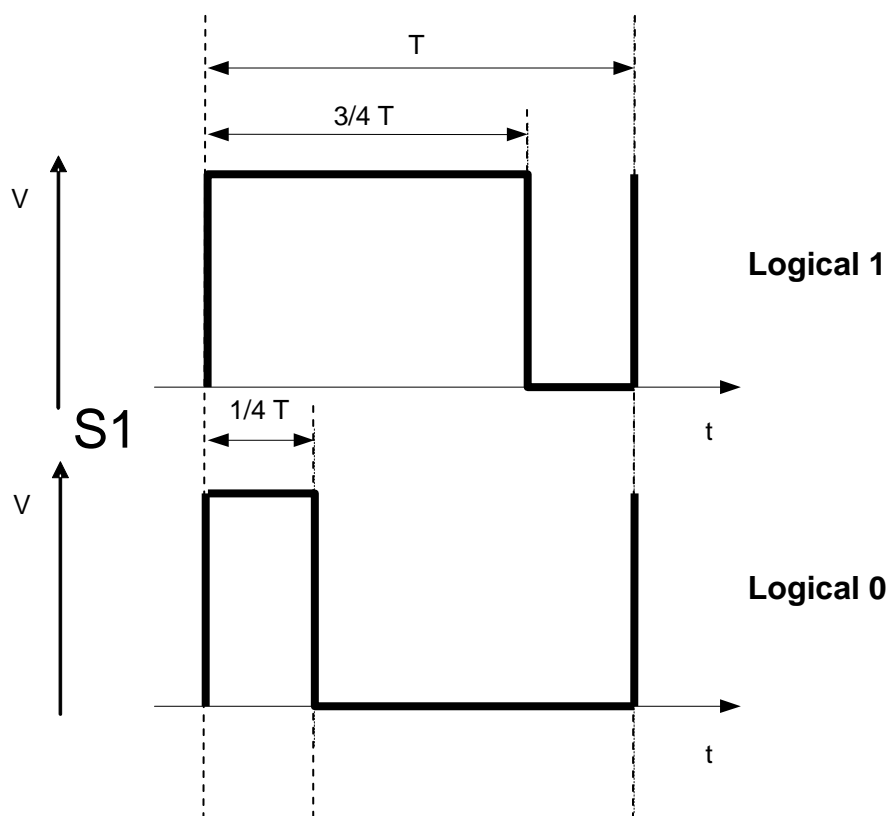
Figure 8.1: Bit-coding of S1
