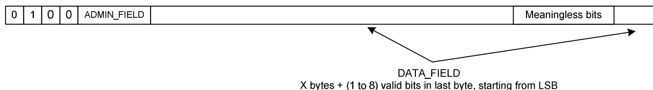
CLT LPDU with DATA_FIELD „byte aligned“ structured
