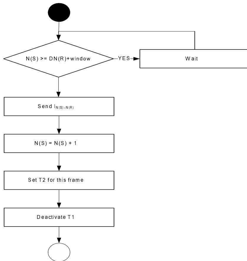
Figure 10.19: Information frame emission.
