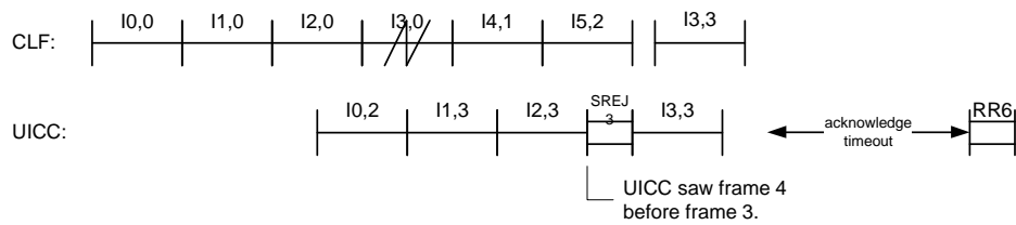
Figure 10.18: One frame loss in stream
