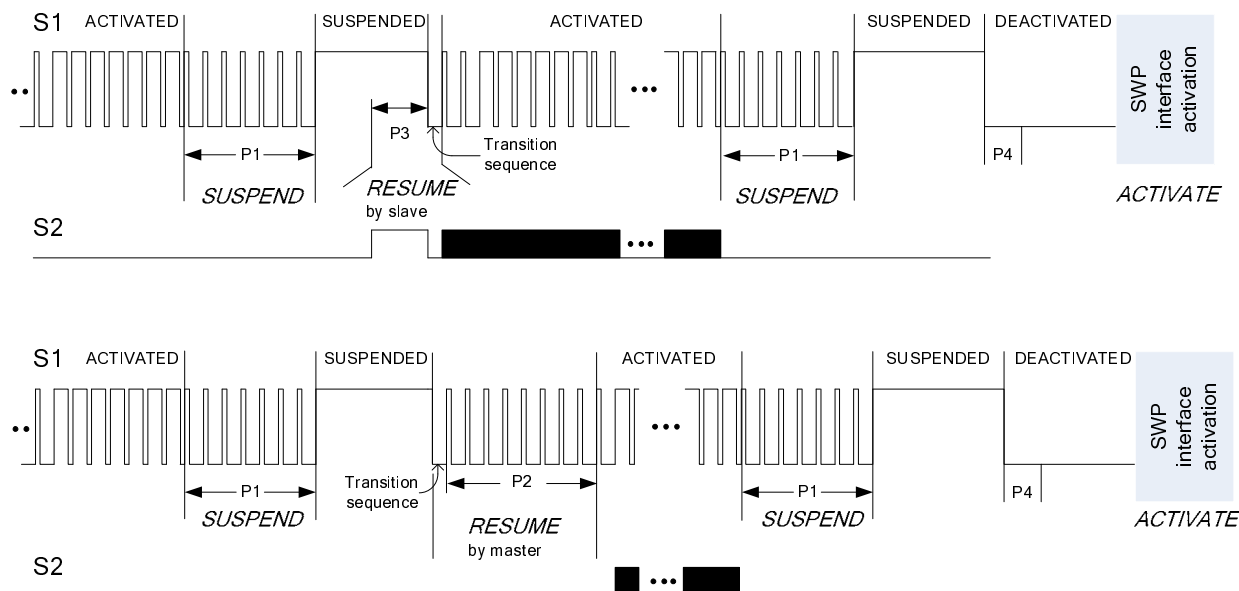
Figure 8.5: SWP states and transitions
