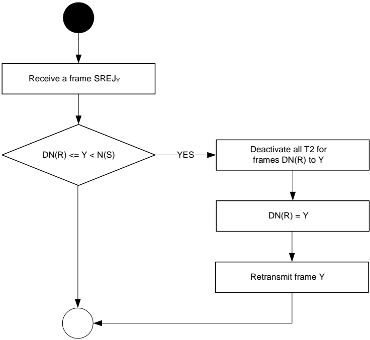
Figure 10.23: SREJ frame reception
