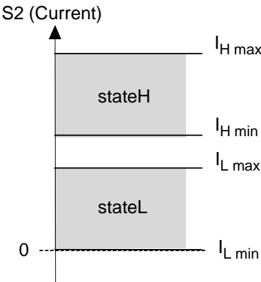
Figure 7.2: Definitions of the current level for S2 on SWIO
