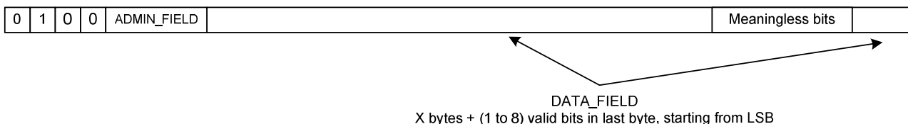
CLT LPDU with DATA_FIELD „byte aligned“ structured
