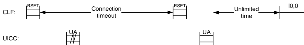
Figure 10.5: Link establishment restart after UA loss
