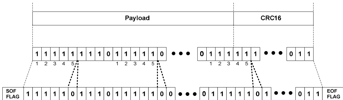
Figure 9.4: Bit stuffing
