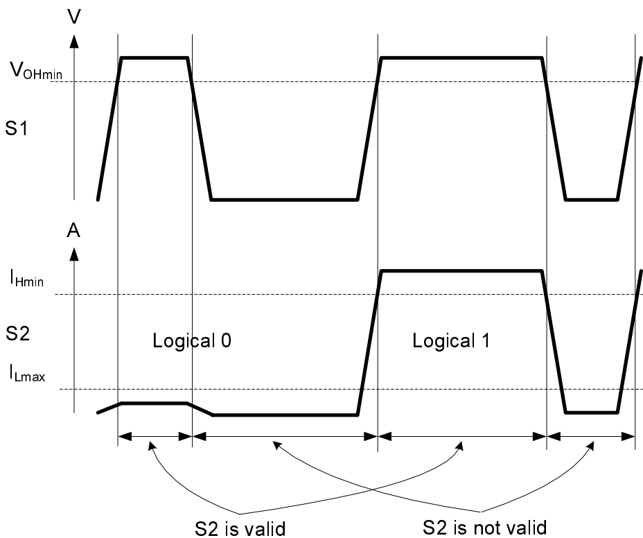
Figure 8.3: S2 timing
