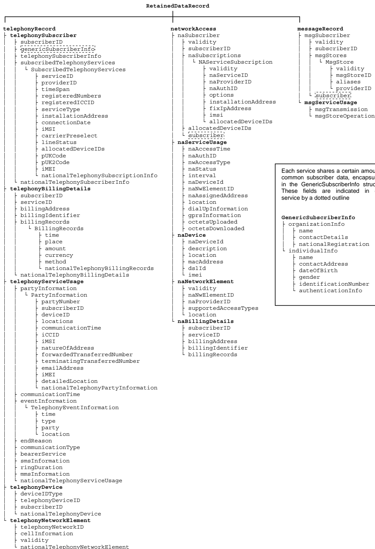
Figure A.2: Schematic representations of the major ASN.1 structures for three services
