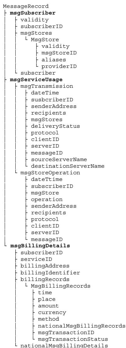
Figure C.2: Schematic representations of the major ASN.1 structures for asynchronous messaging
