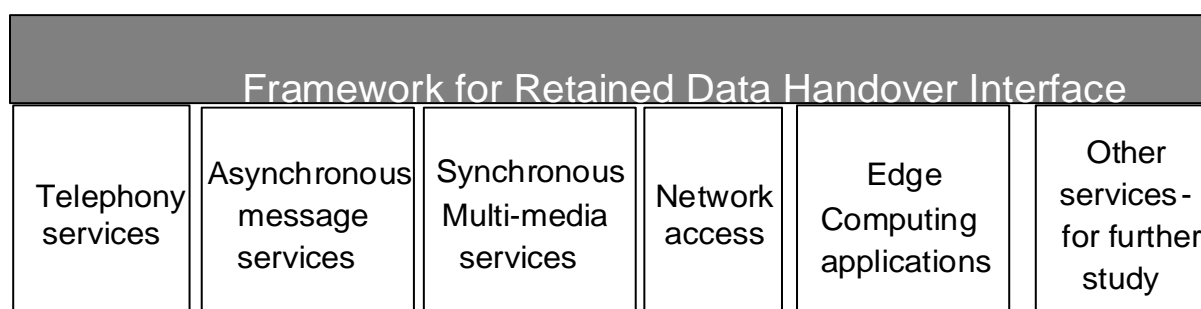
Figure 3: Framework structure
