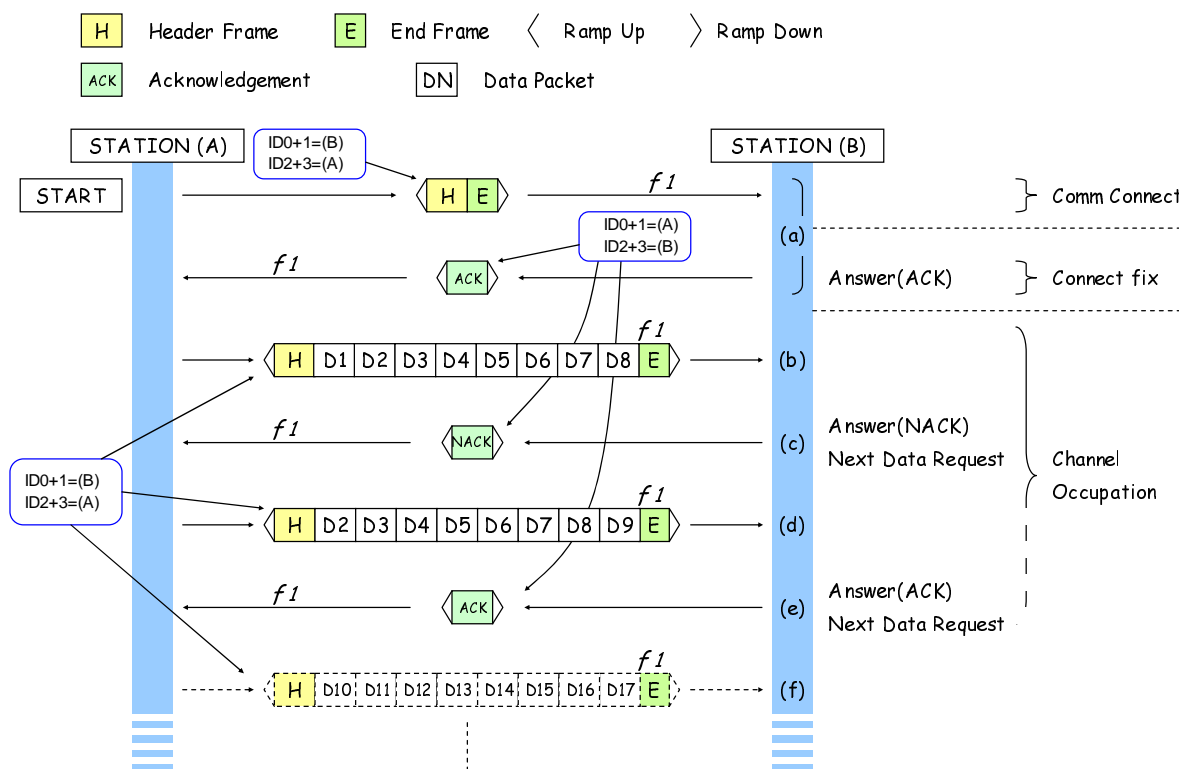
Figure 9.4: Packet retractions
