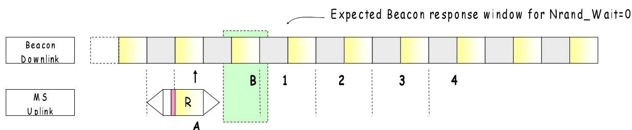
Figure 12.18: Random Backoff Example #1
