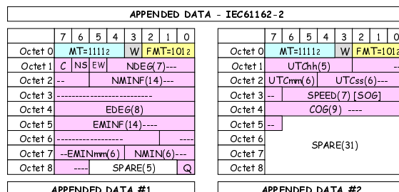
Figure 5.13: UDT Appended_Data EN61162-1 Format
