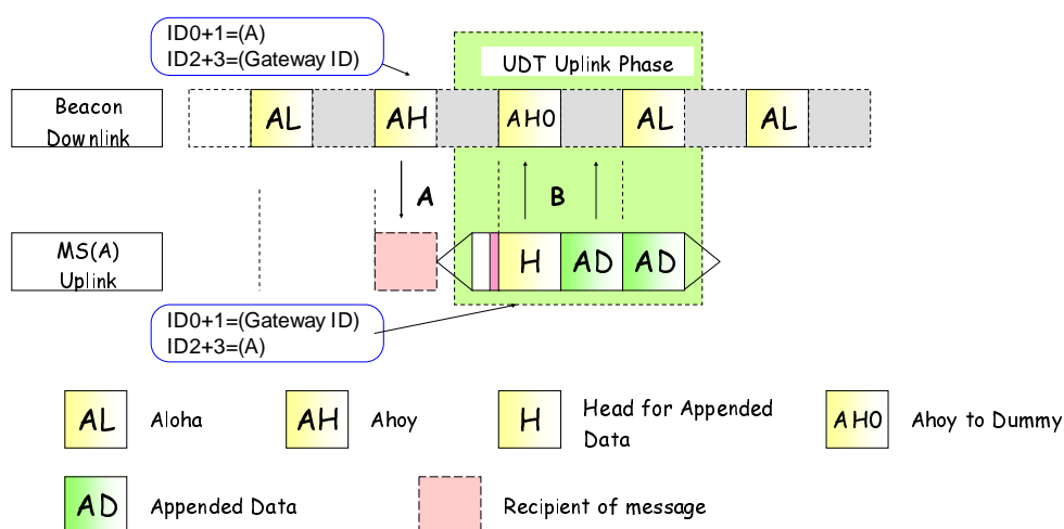
Figure 10.40: Example of short data polling from a gateway
