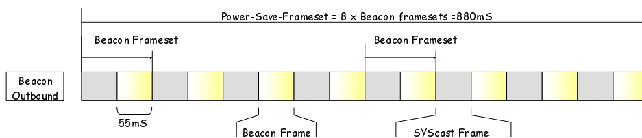
Figure 12.8: Beacon frames and Framesets
