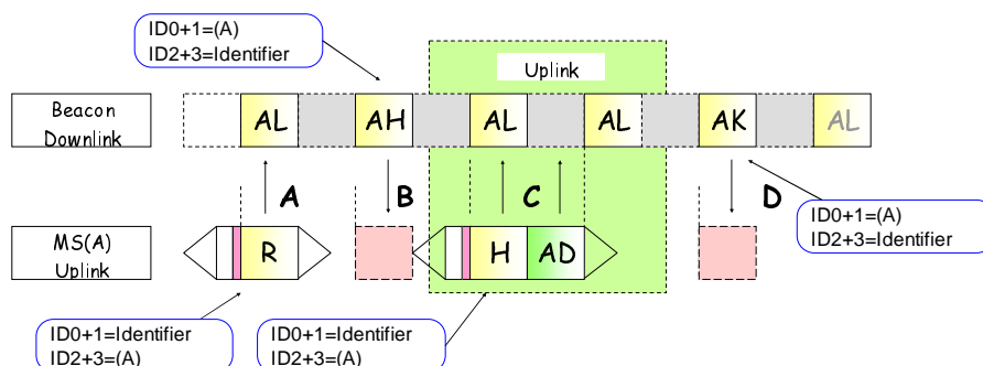
Figure 10.41: Example of a Call Diversion Call
