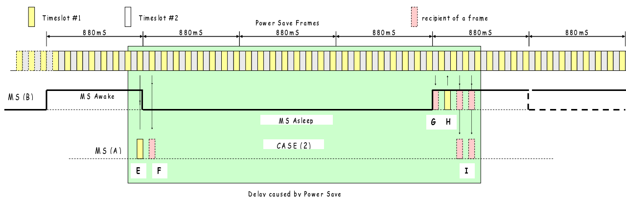
Figure 12.29: Power Save Frame Example #2
