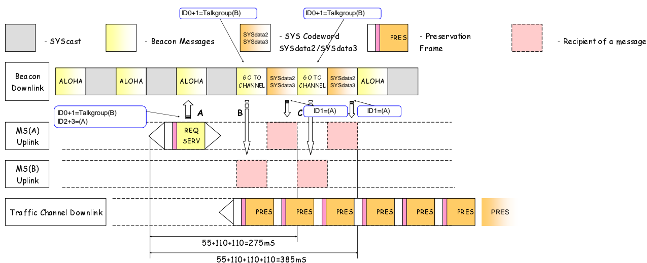
Figure 10.28: Group Call set-up example
