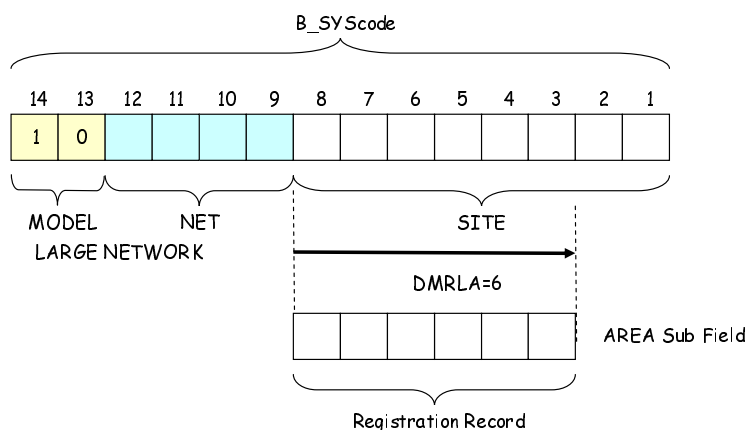
Figure 12.24: Extraction of the registration record from the SYScode
