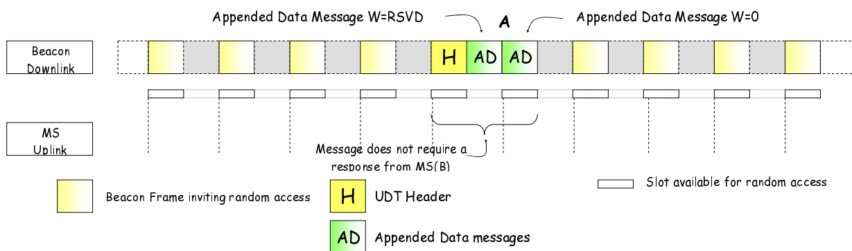
Figure 12.17: Withdrawn Framesets Example #4
