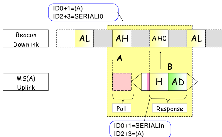
Figure 12.30: Serial Number Check
