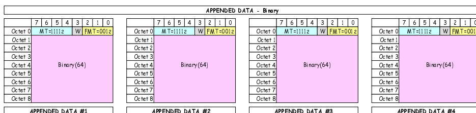
Figure 5.9: Appended_Data (Binary)
