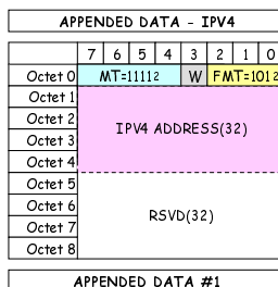
Figure 5.14: UDT Appended_Data IPV4 Format
