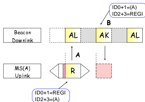
Figure 12.25: Registration Exchange
