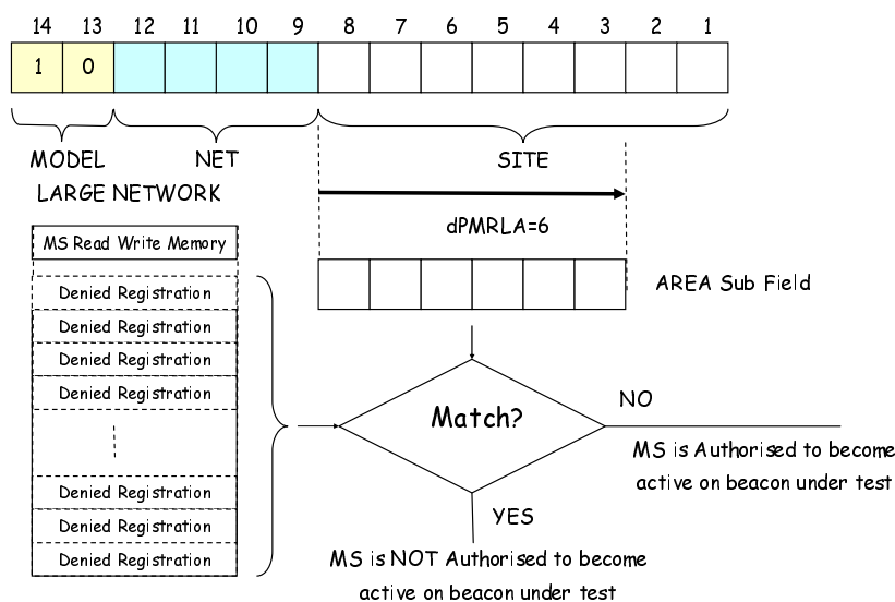
Figure 12.23: SYS_AREA field from the SYScode
