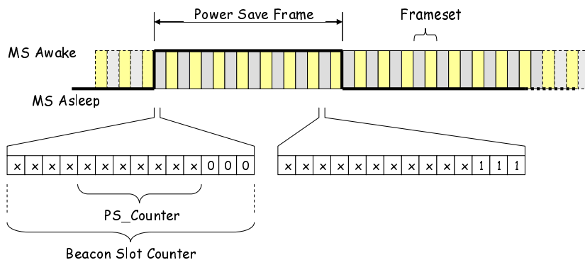
Figure 12.27: Power Save Frame Structure
