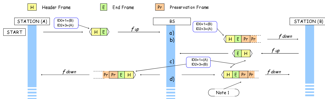
Figure 10.16: Mode 2 Status Polling
