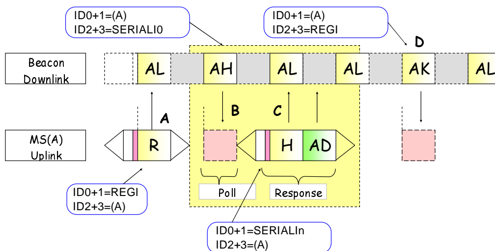
Figure 12.26: Registration with serial check
