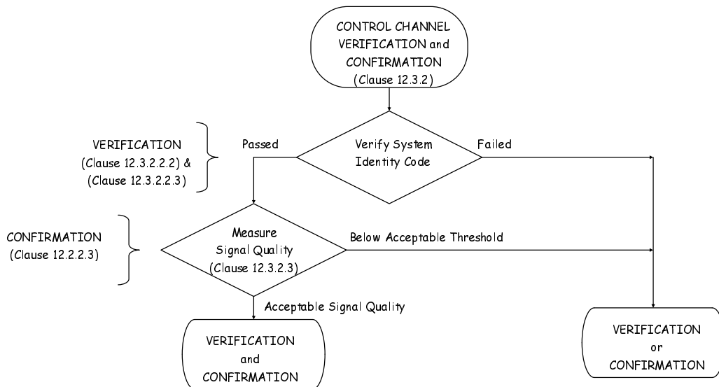
Figure 12.20: Verification and Confirmation Steps
