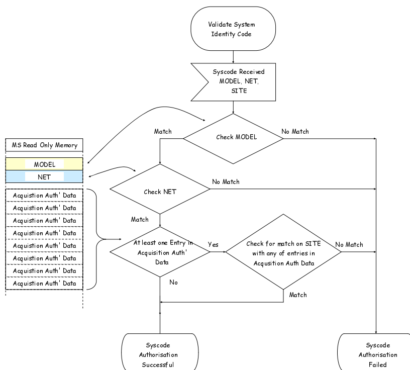
Figure 12.22: Checking the SYScode
