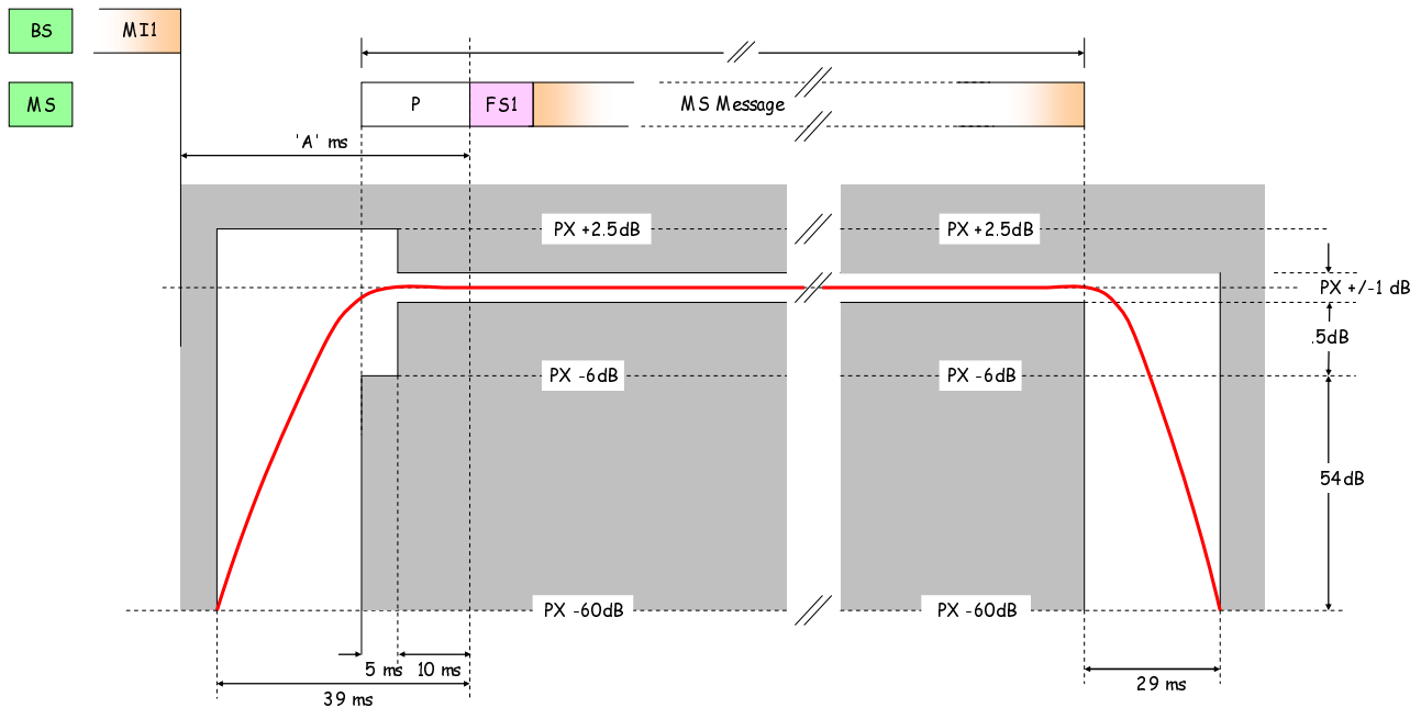
Figure 14.2: MS Power Ramp
