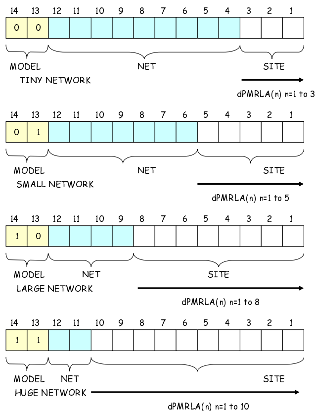
Figure 12.21: Allocation of NET and SITE fields in SYSCode
