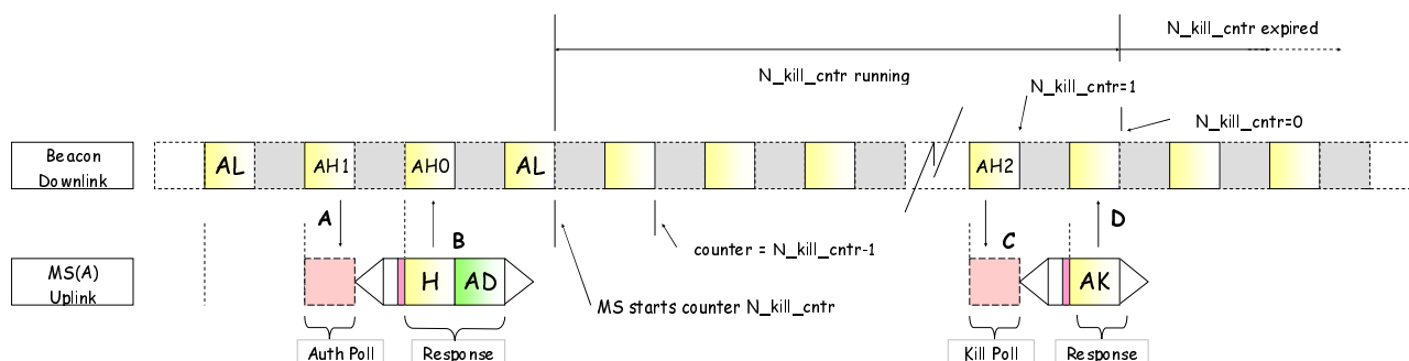
Figure 10.44: Example of successful kill procedure
