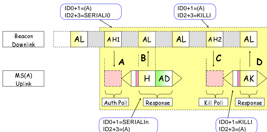
Figure 10.43: MS Kill (with Authentication)
