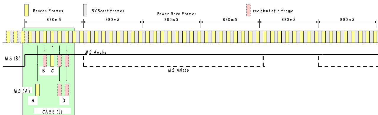
Figure 12.28: Power Save Frame Example #1
