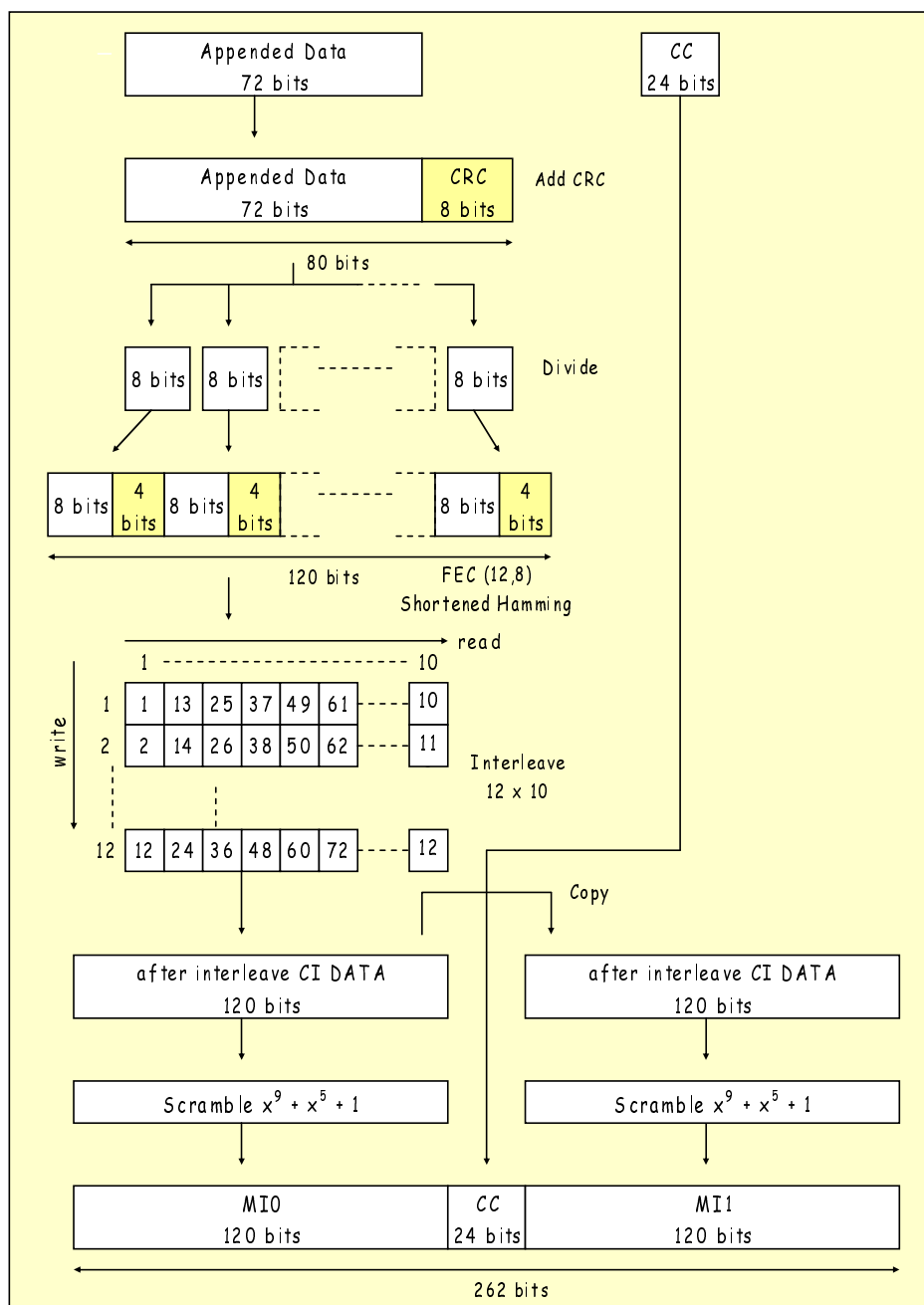
Figure 11.11: Appended Data frame coding
