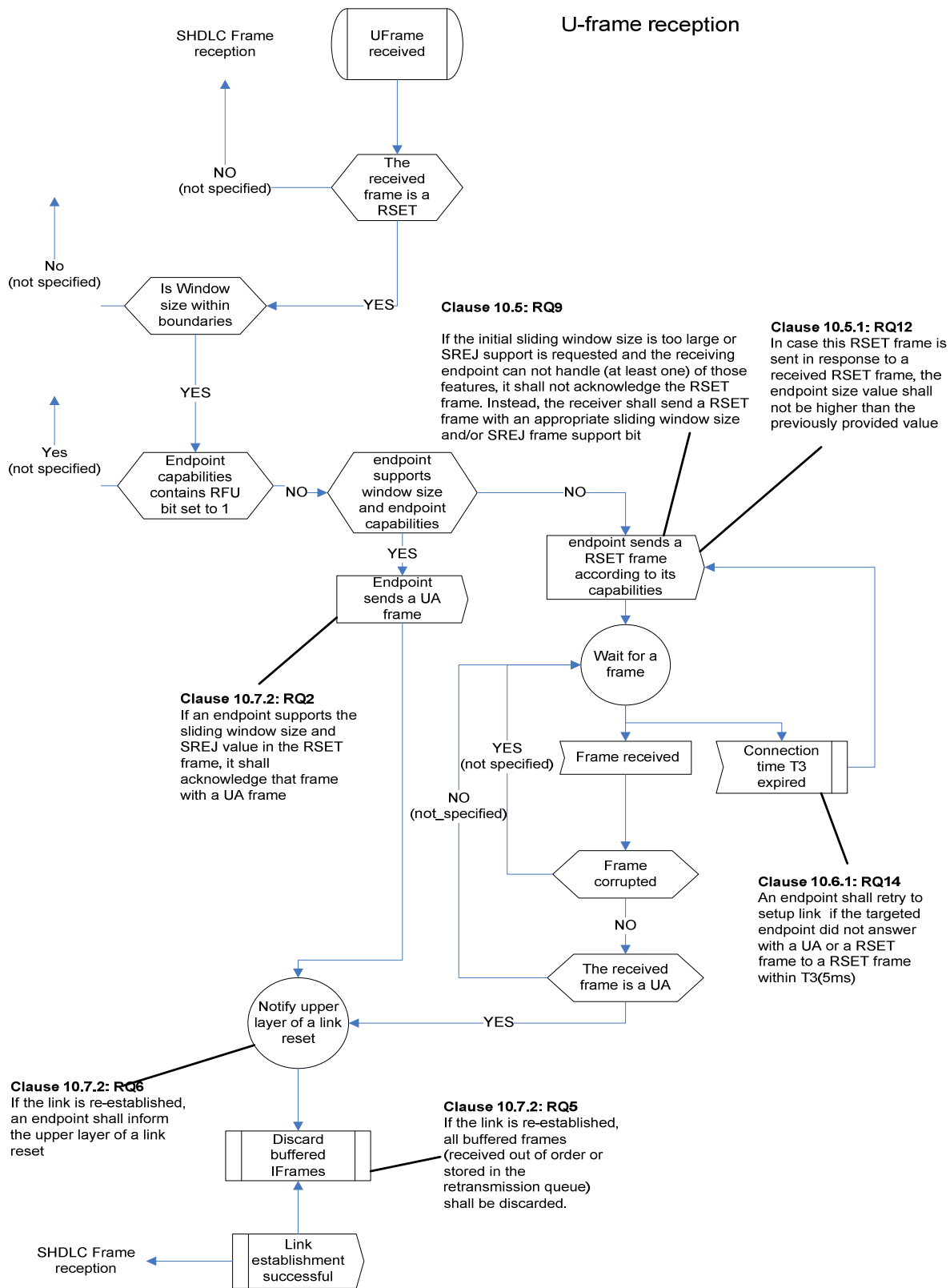
Figure A.3.5: U-frame reception
