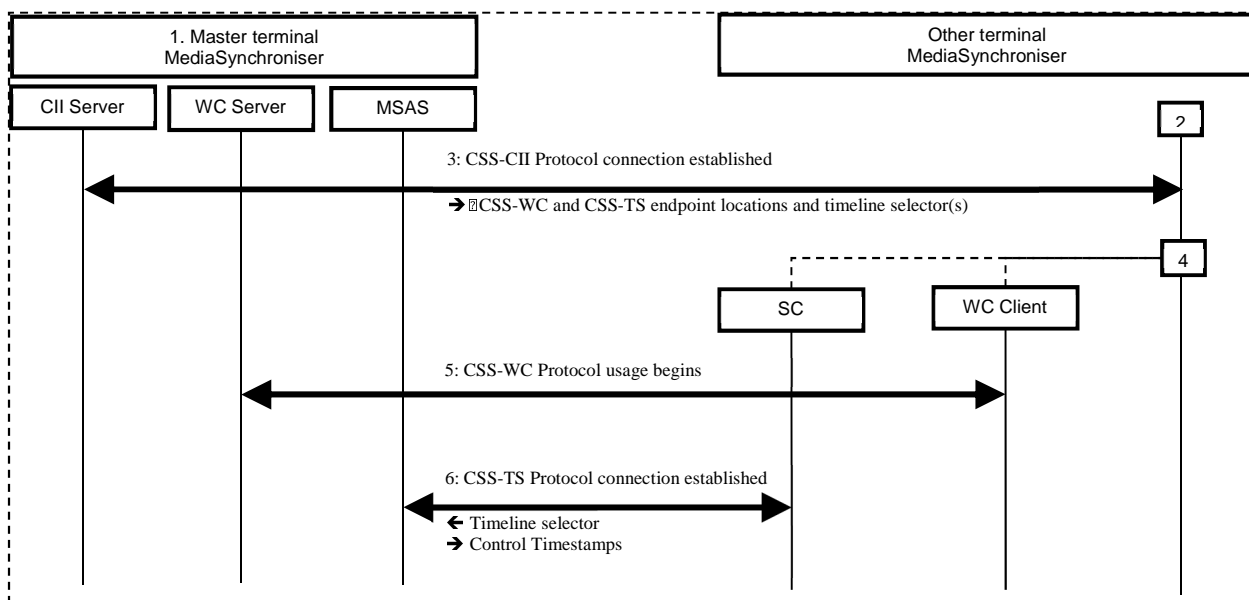
Figure 25: Protocol interactions for inter-device timeline synchronization
