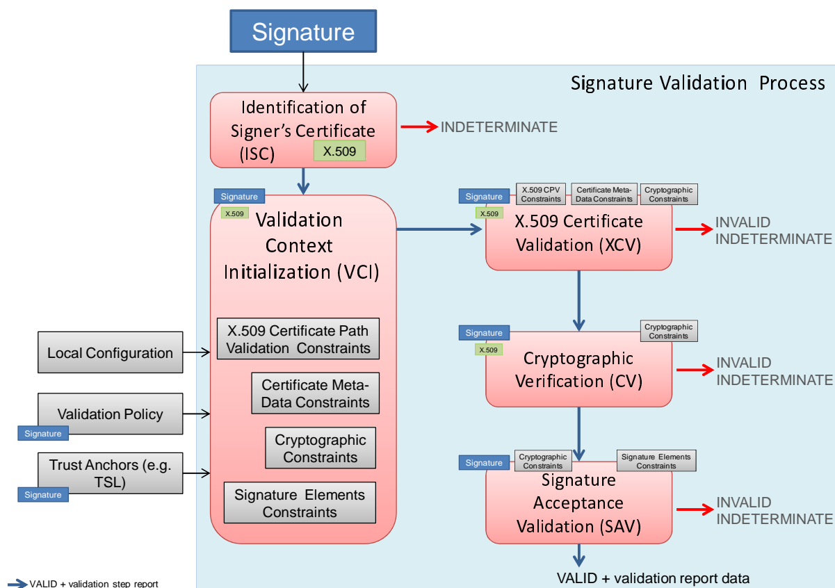
Figure 3: Signature Validation
