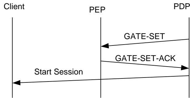
Figure 7: Sample Signalling of Gate-Set
