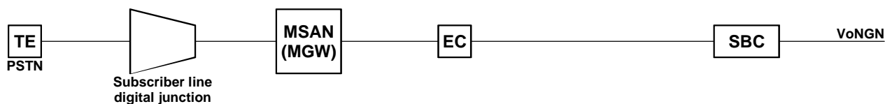
Figure 5: Reference configuration for NGN with PSTN/ISDN access
