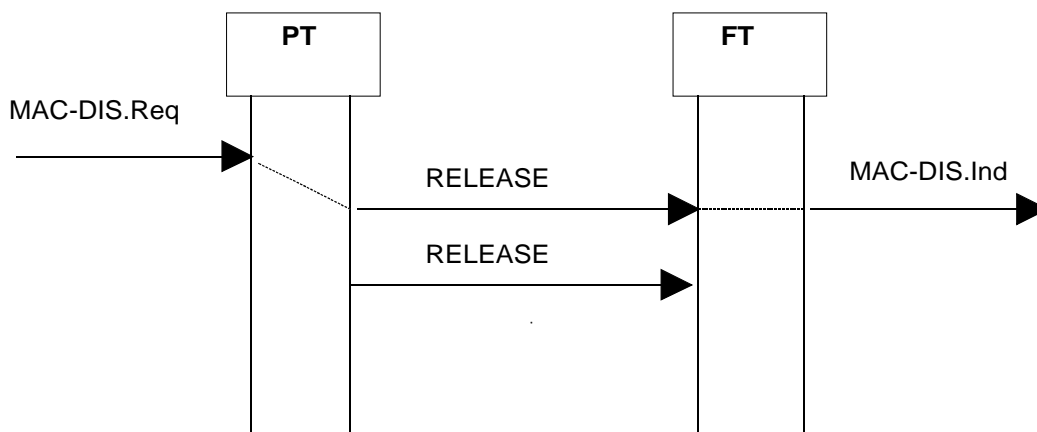
Figure 7: Bearer release
