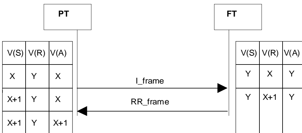
Figure 59: Class A acknowledge information transfer by RR_frame
