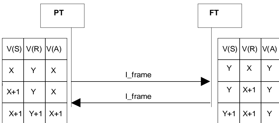
Figure 58: Class A acknowledge information transfer by I_frame, PT initiated
