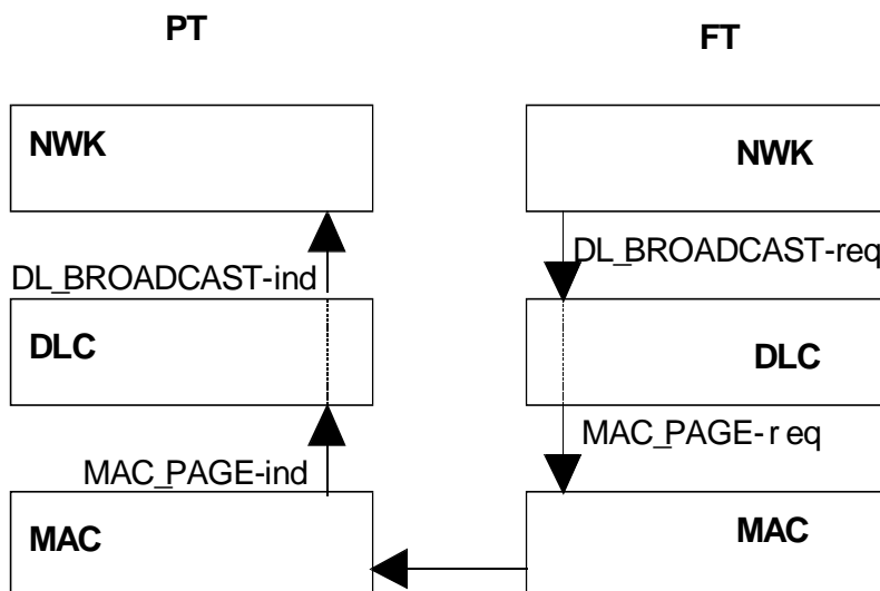
Figure 61: Normal broadcast
