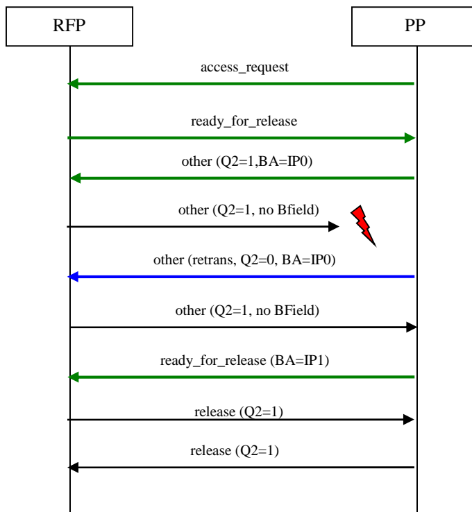
Figure 30: Packet Mode Connection success (2 nd other message retransmitted)
