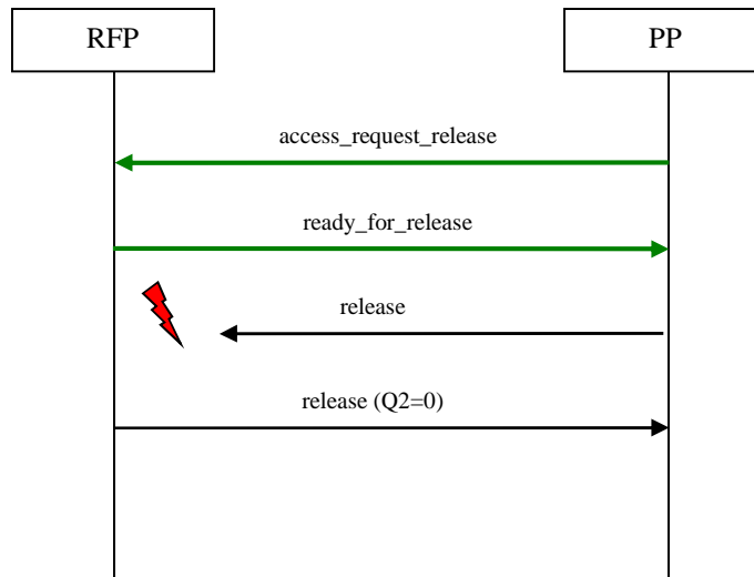
Figure 31: Two-way Single Packet Mode Connection (1 st release message wrong)
