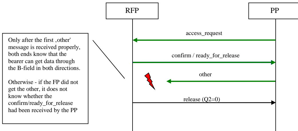
Figure 29: Packet Mode Connection setup fails (other message wrong)
