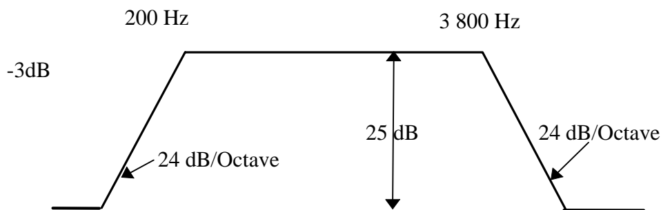
Figure A.1: Response for the band-limiting filter
