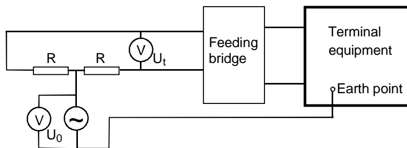
Figure A.3: Loop steady state configuration
