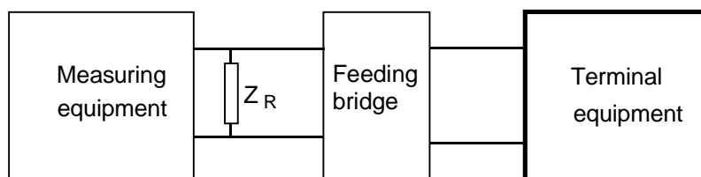
Figure A.8: Sending level above 4,3 kHz configuration
