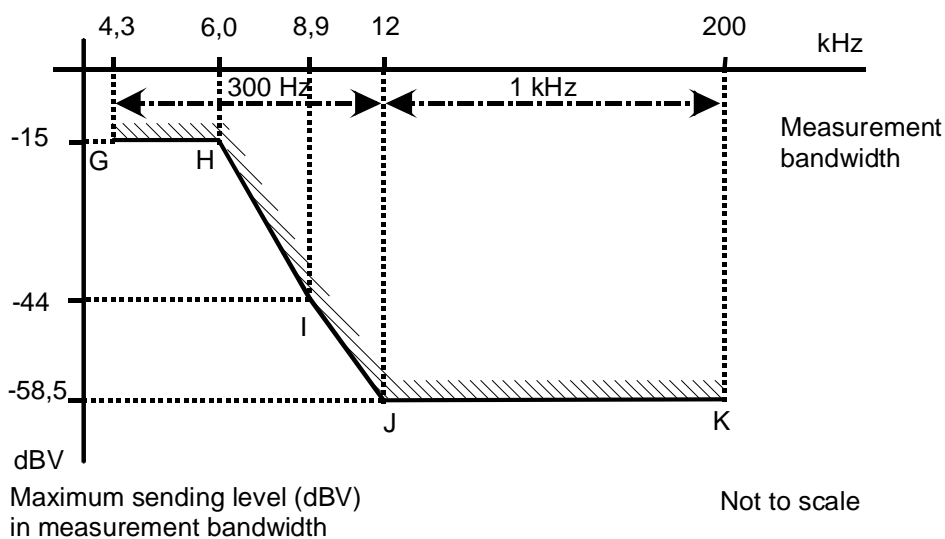
Figure 4: Sending level above 4,3 kHz
