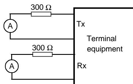
Figure A.10: Power feeding test for 4 wire TE
