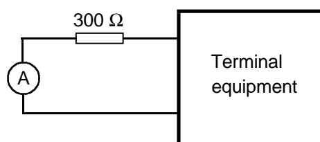
Figure A.9: Power feeding test for 2 wire TE
