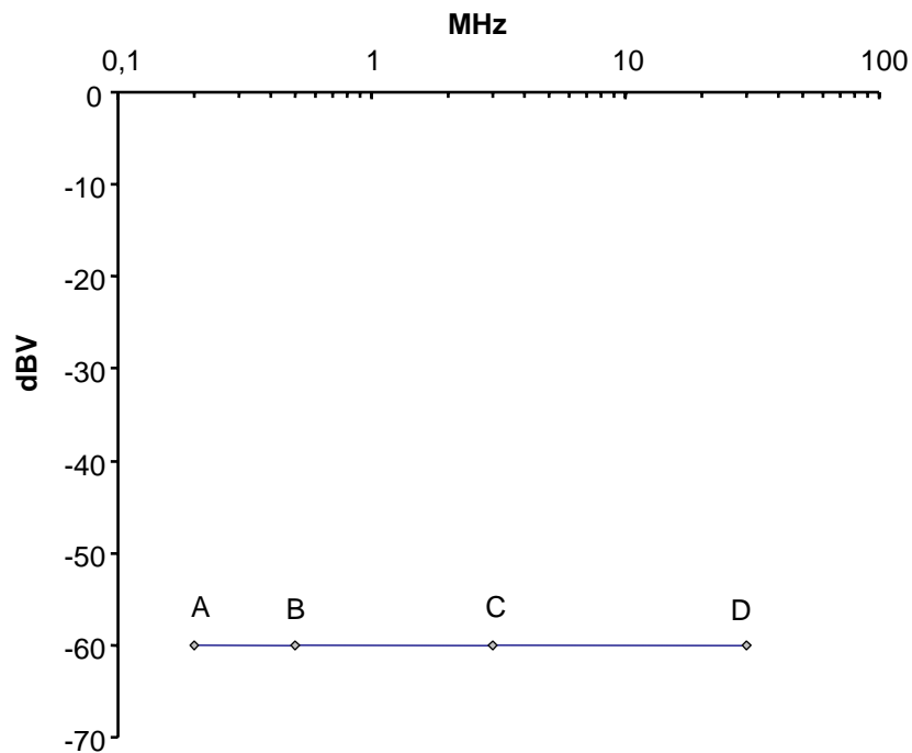
Figure 5: Maximum sending between 200 kHz and 30 MHz
