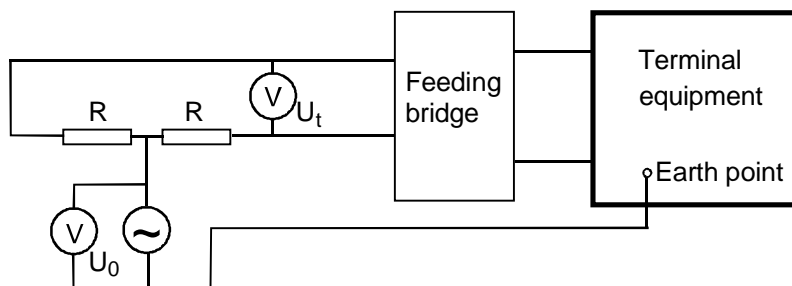
Figure A.2: Impedance balance about earth
