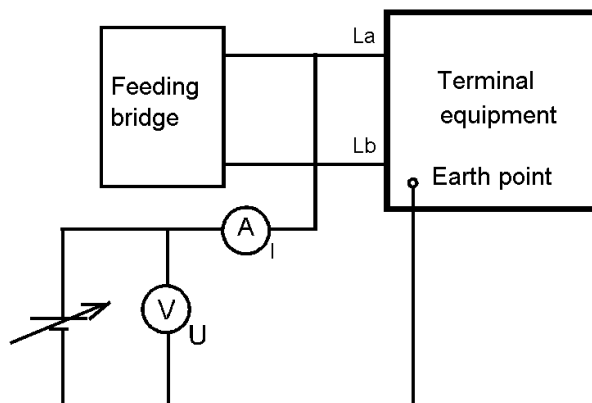
Figure A.13: Resistance to earth configuration
