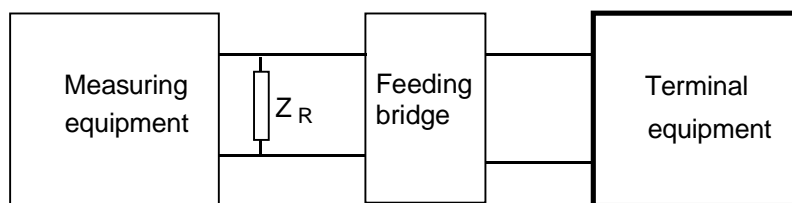
Figure A.22: Call attempt on a low voltage line configuration
