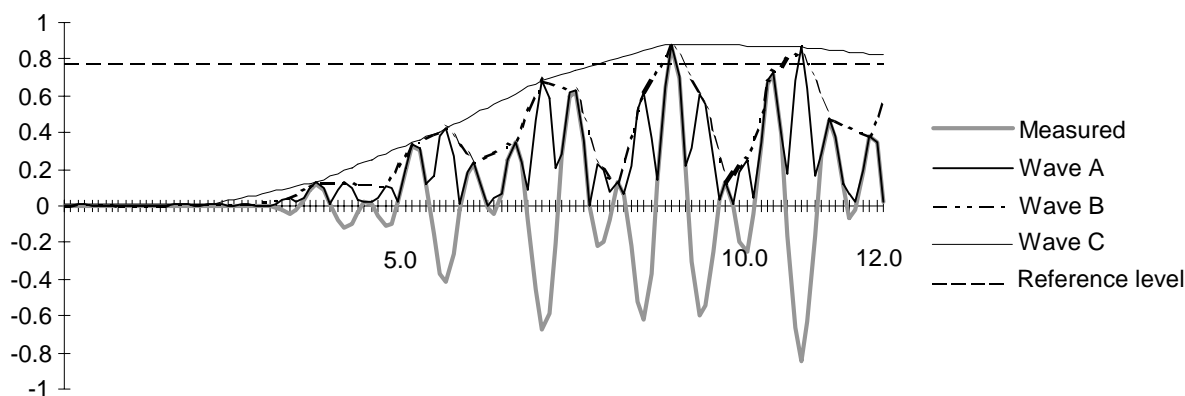
Figure A.20: Relationship between measured wavelength and waveforms A, B and C
