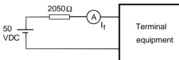
Figure A.23: Transition from loop to quiescent state configuration
