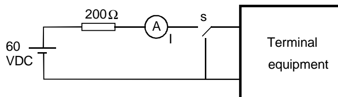
Figure A.3: Transient reponse: configuration
