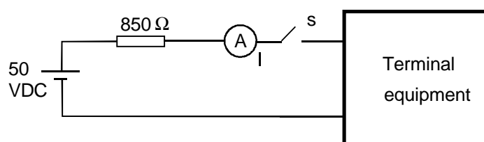
Figure A.8: Acceptance of breaks in the loop in a call attempt configuration
