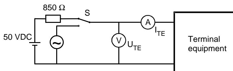
Figure A.10: Ring trip configuration
