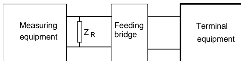
Figure A.21: Pause duration configuration
