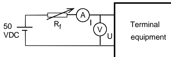
Figure A.11: DC characteristics configuration
