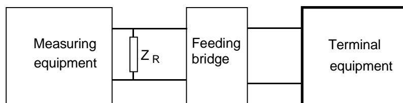
Figure A.14: Dialling without dial tone detection configuration
