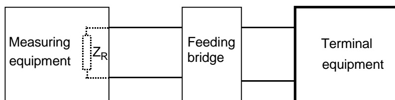
Figure A.12: Impedance configuration
