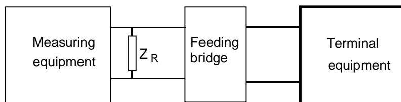
Figure A.17: Signalling levels configuration
