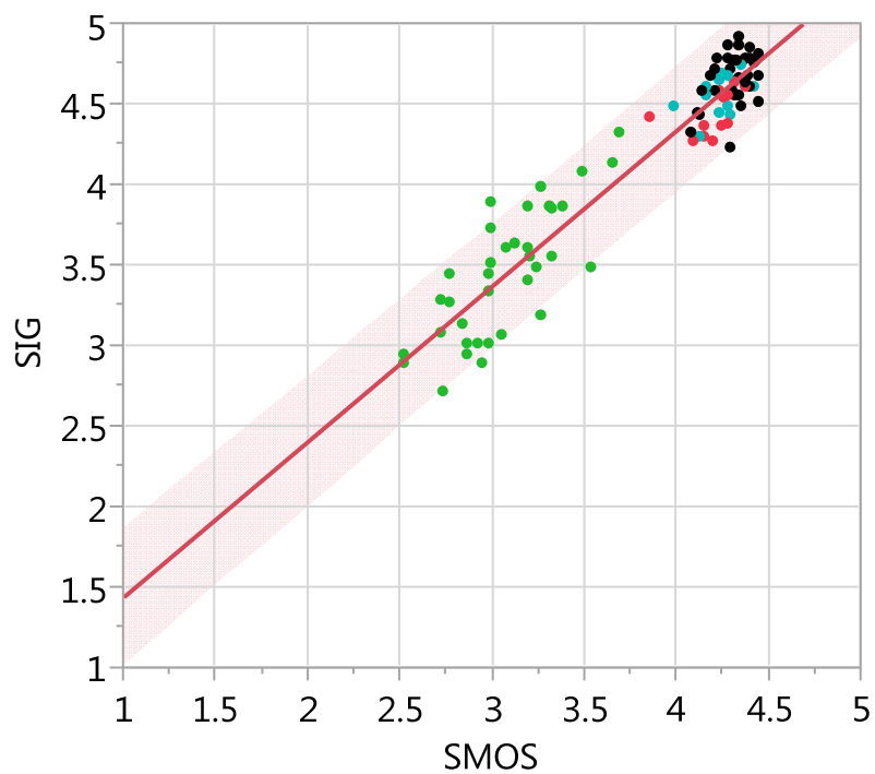
Figure 49: S-MOS fit to SIG, Tests 5 & 6, shaded area is 95 % confidence interval
