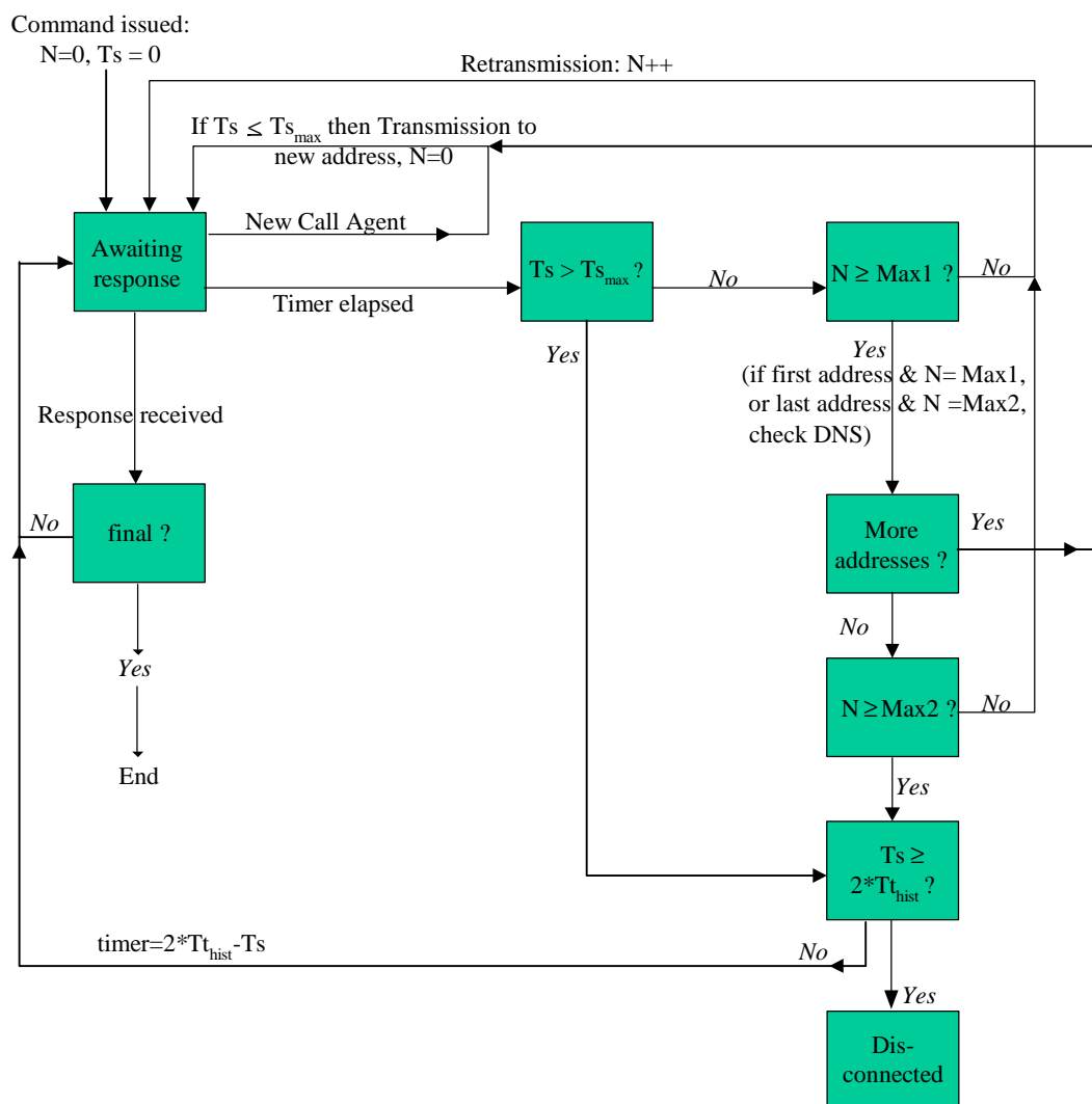
Figure 4: Retransmission Algorithm
