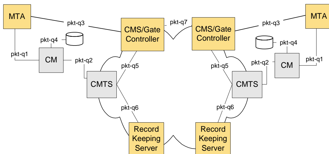
Figure 1: QoS Signalling Interfaces in IPCablecom Network
