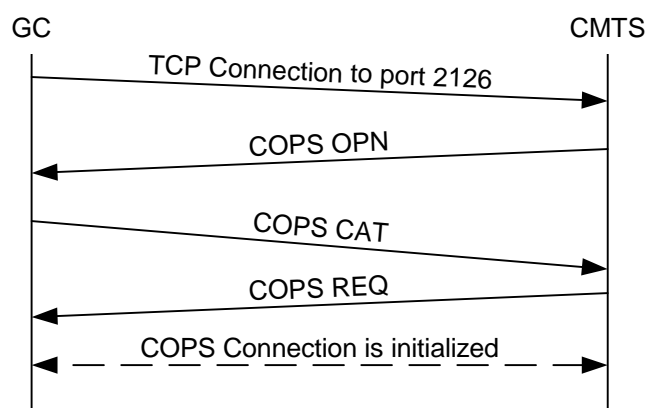
Figure 13: COPS Connection Establishment
