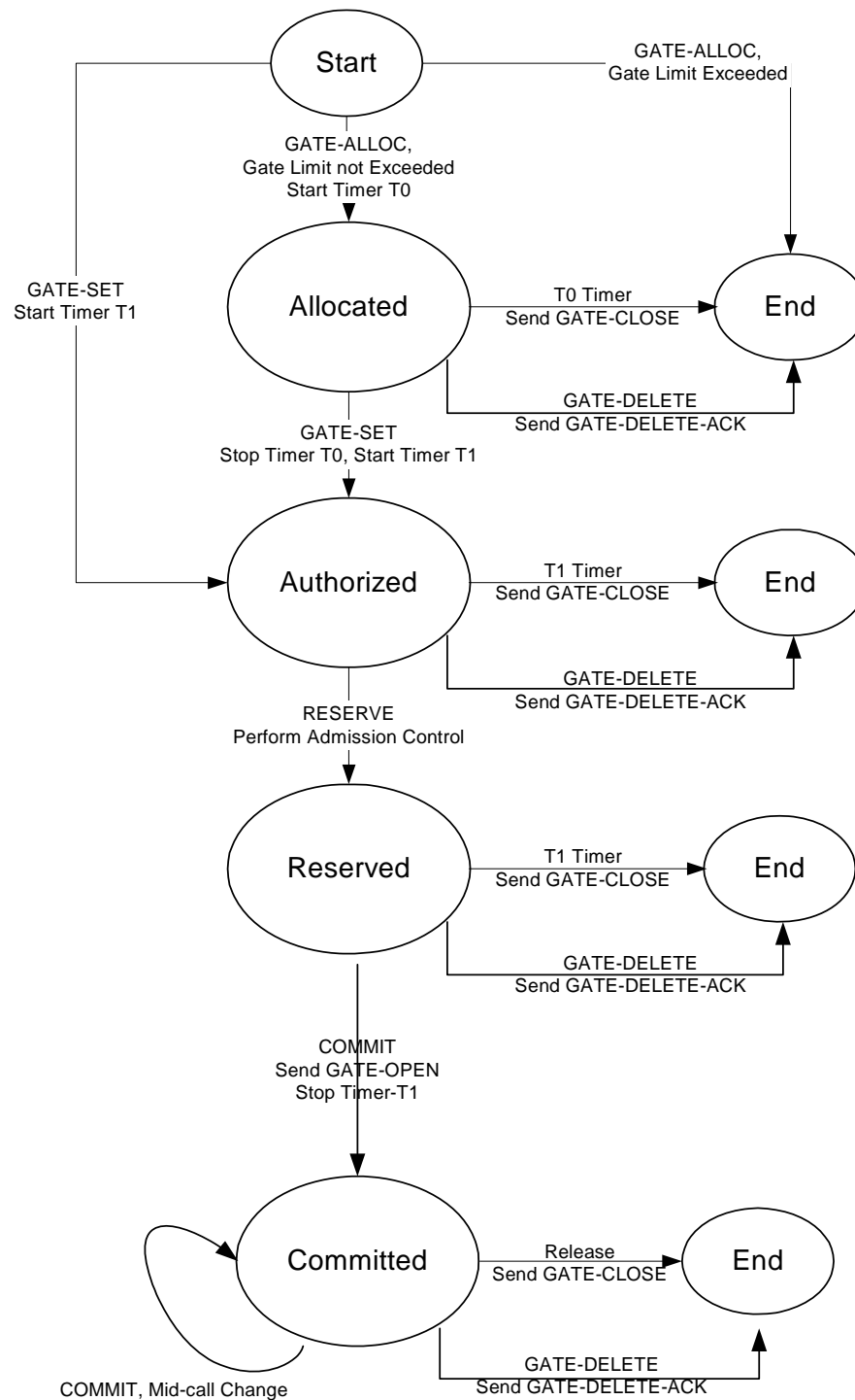
Figure 9: Gate State Transition Diagram
