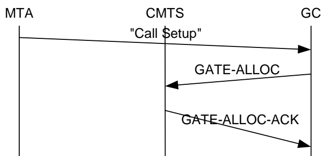
Figure 15: Sample Signalling of Gate-Alloc
