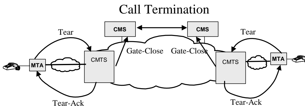
Figure 18: Coordination of Call Termination
