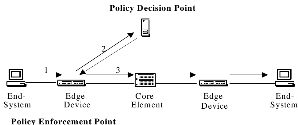
Figure B.1: COPS Protocol
