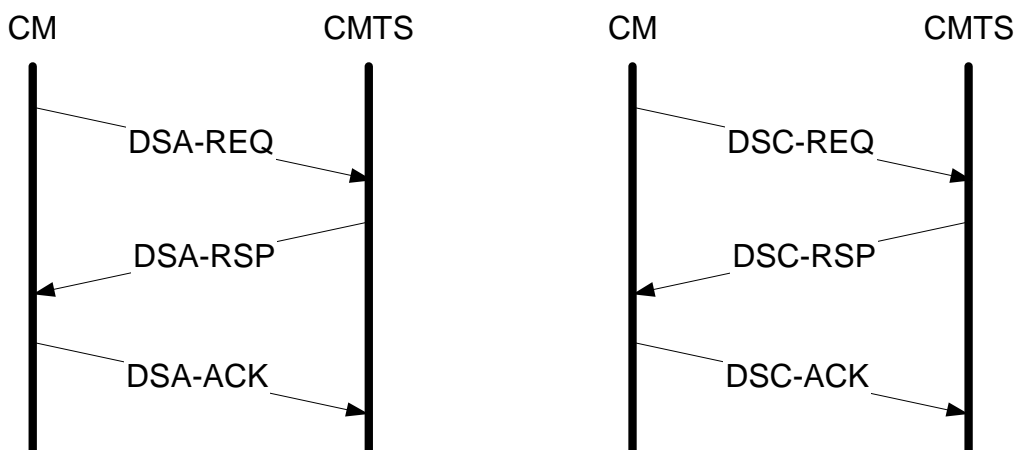
Figure 5: DSA and DSC exchanges between CM and CMTS
