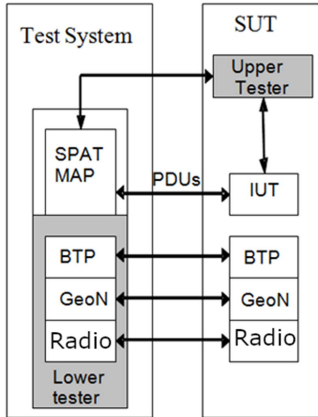
Figure 1: Abstract protocol tester - MAPEM SPATEM case
