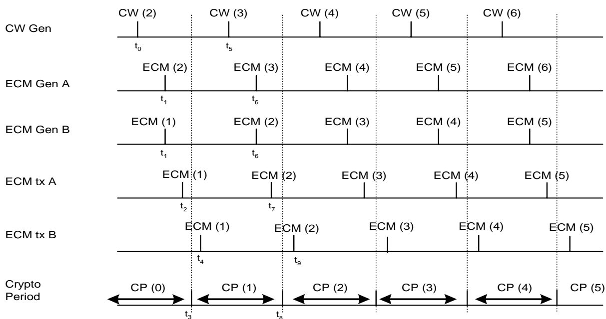
Figure 19: ECM timing diagram
