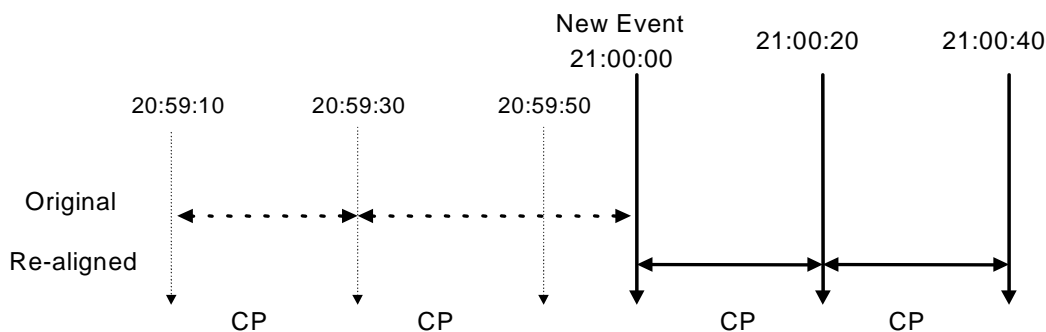
Figure 22: Event realignment
