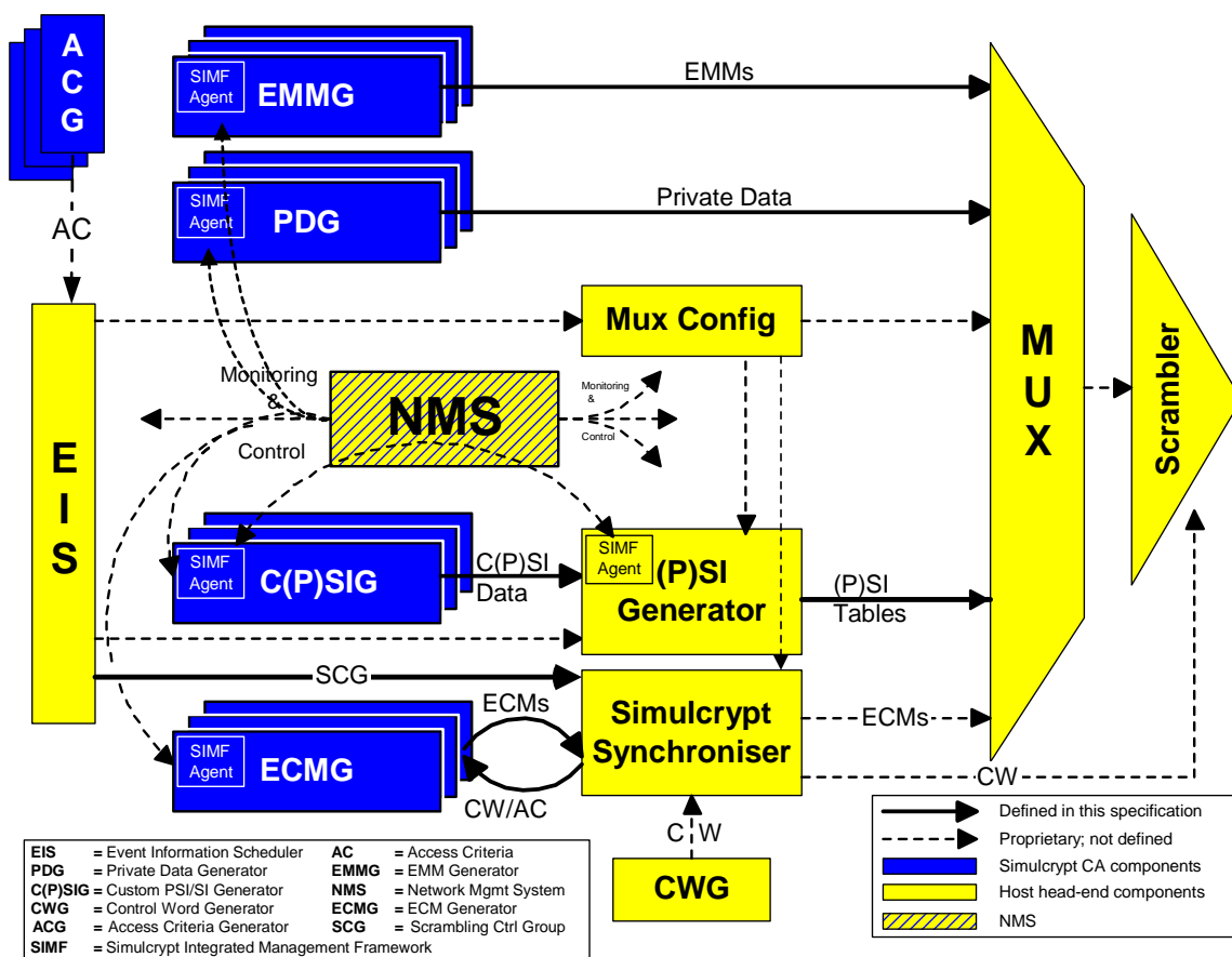
Figure 1: System architecture
