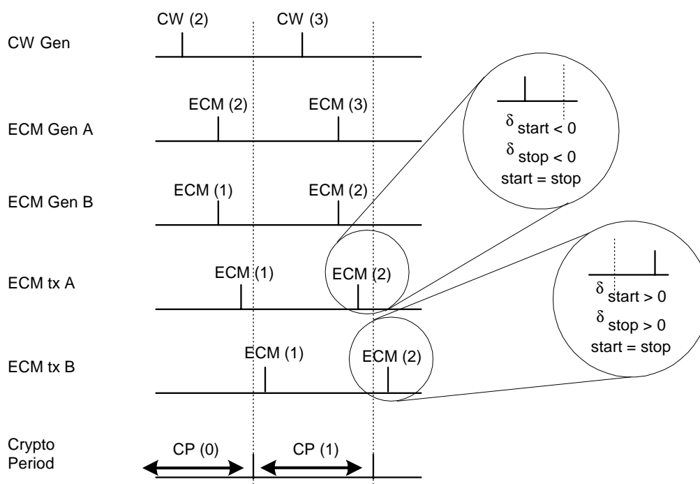
Figure 20: Delay_start and Delay_stop
