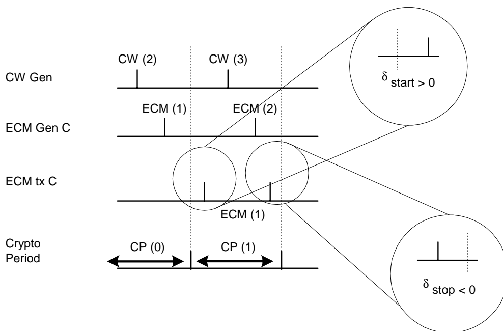
Figure 21: End of ECM transmission around cryptoperiod boundary
