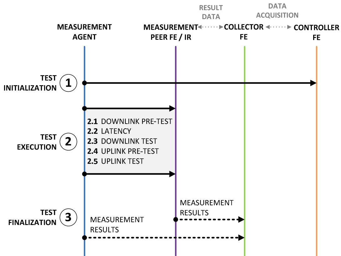
Figure 54: The workflow of the measurement system
