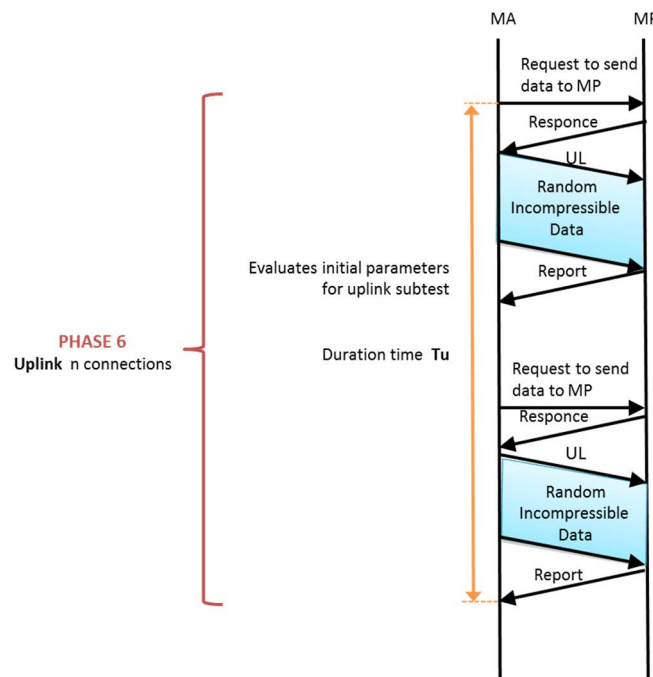
Figure 59: Sample diagram of phase 6 of measurement algorithm
