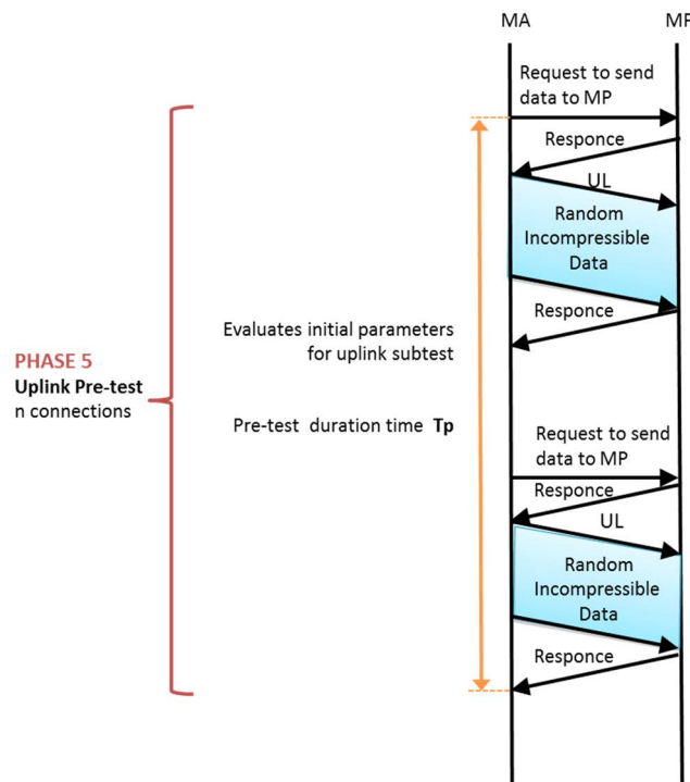
Figure 58: Sample diagram of phase 5 of measurement algorithm
