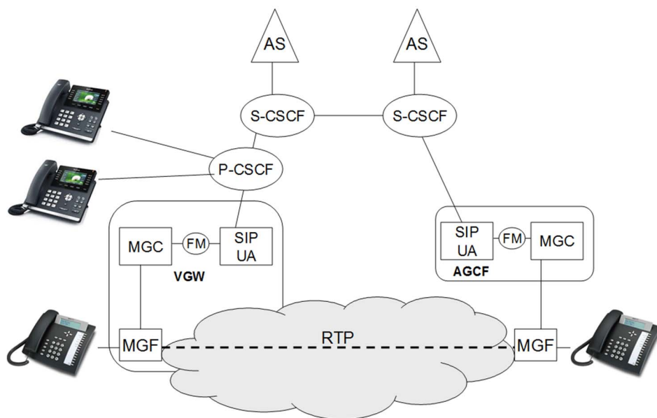
Figure 3: AGCF/VGW session processing models
