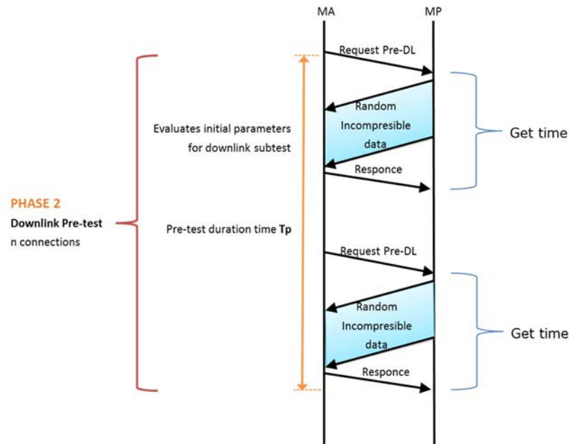
Figure 55: Sample diagram of phase 2 of measurement algorithm
