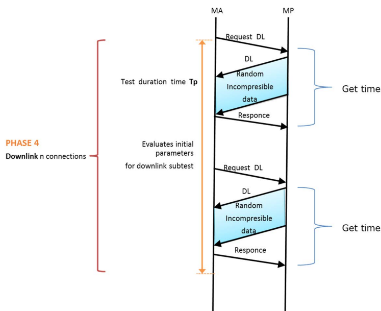
Figure 57: Sample diagram of phase 4 of measurement algorithm
