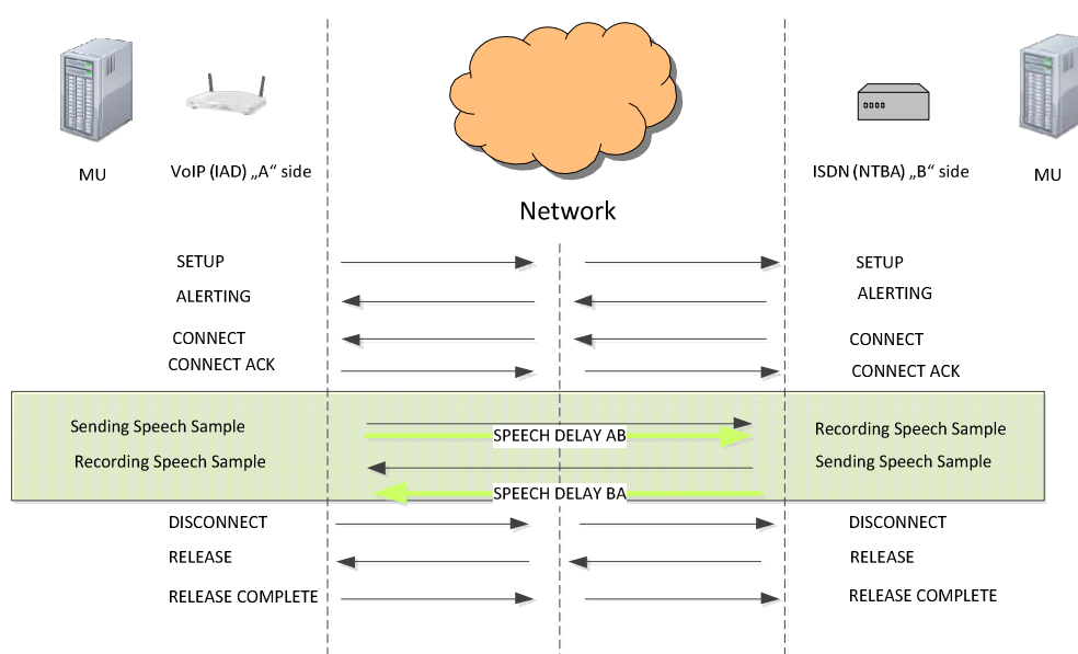
Figure 26: Measurement of the speech delay
