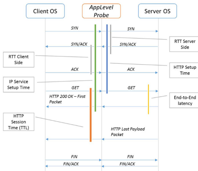
Figure 5.2.1-1: Web browsing
