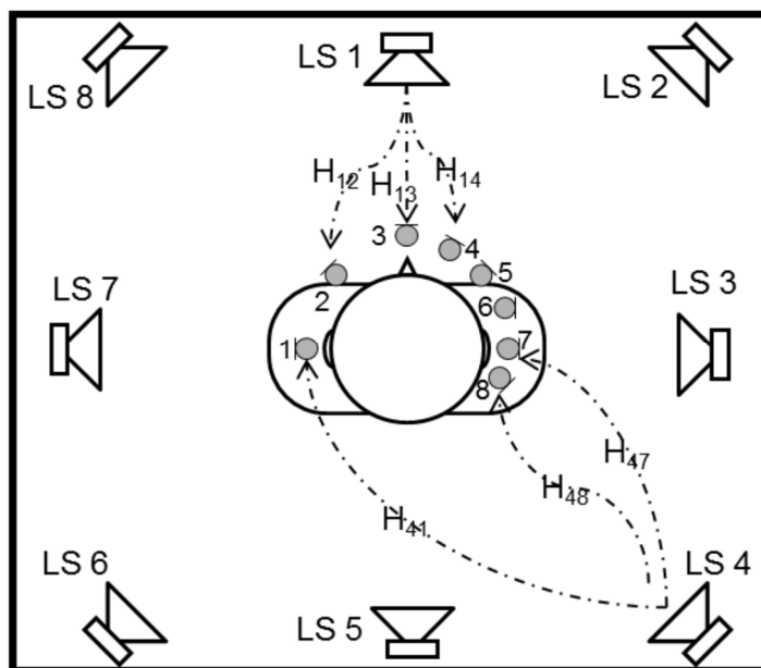
Figure 5: General loudspeaker setup and principle of the equalization paths for the handset and headset measurement setup
