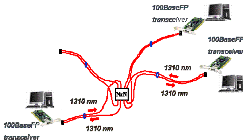
Figure D.10: "LAN-like" application implementation
