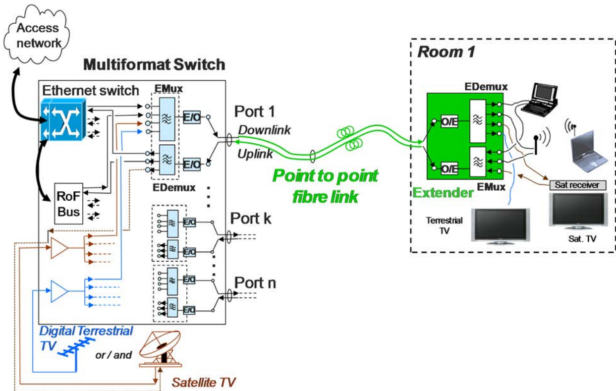
Figure C.2: Network architecture
