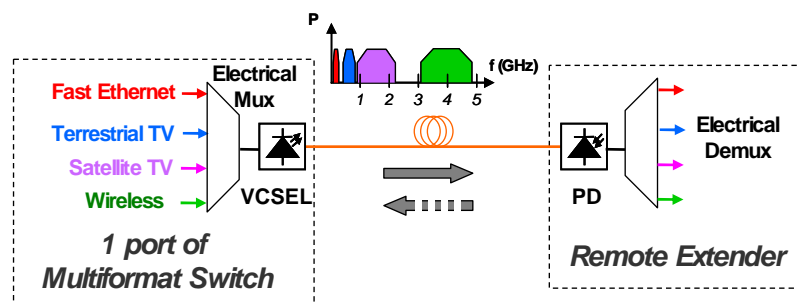
Figure 5: Multiformat link based on electrical multiplexing
