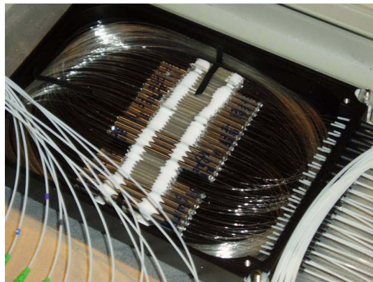
Figure D.4: Picture of the 16 \times 16 optical splitter
