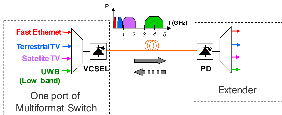
Figure C.1: Electrical multiplex of the different signals
