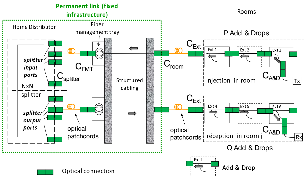
Figure 12: Possible implementation for CWDM passive star based multifformat home network
