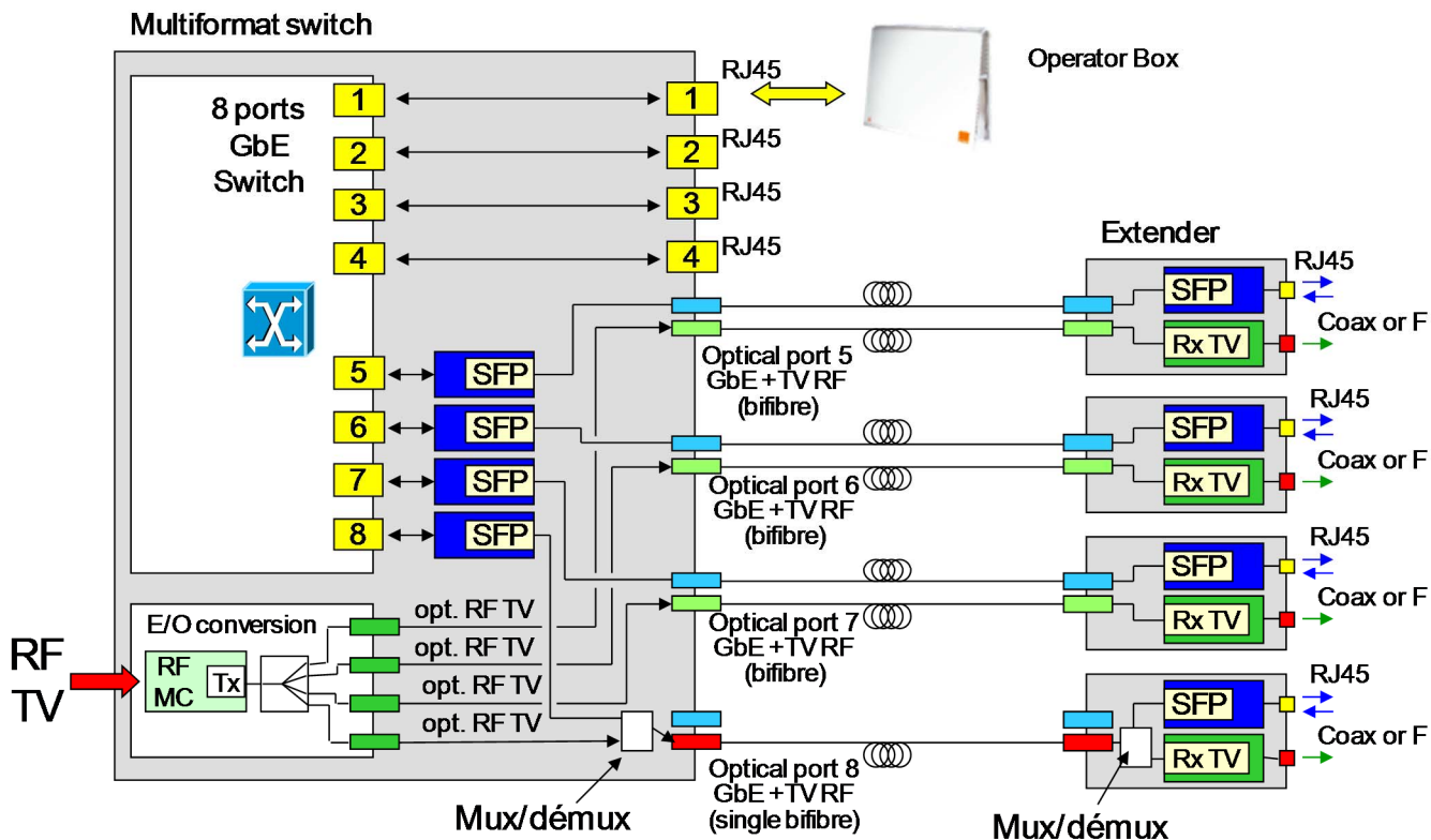
Figure C.15: complete setup configuration
