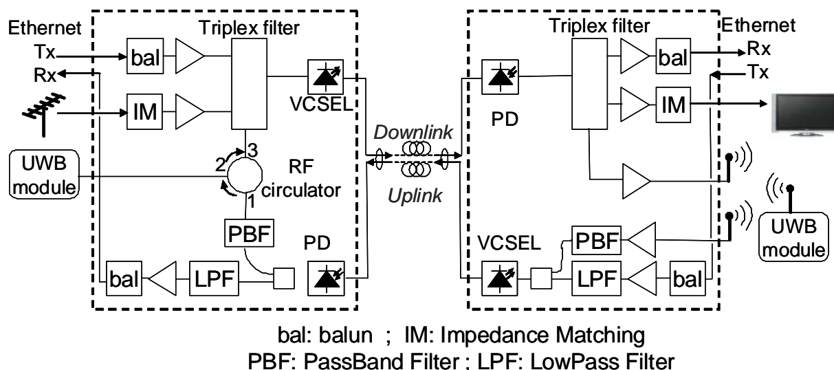
Figure C.4: Realized setup
