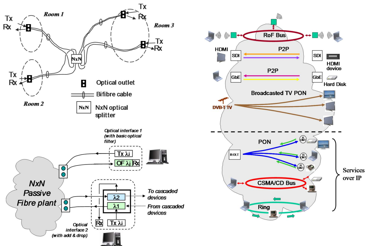
Figure 8: The multifformat passive star solution (CWDM Broadcast & Select architecture)
