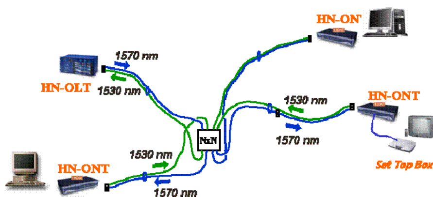
Figure D.8: Implementation of PON-like application
