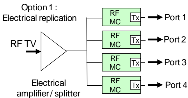
Figure C.13: TV signal replication using electrical splitting
