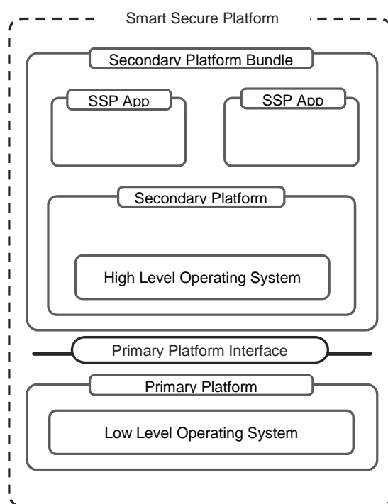
Figure 2: iSSP architecture
