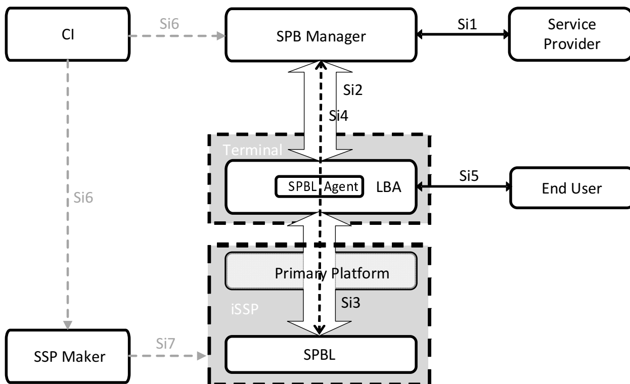
Figure 4: iSSP external interfaces
