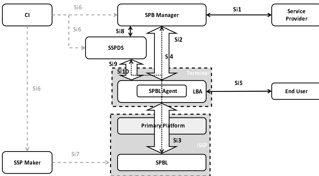
Figure 4: SSP external interfaces
