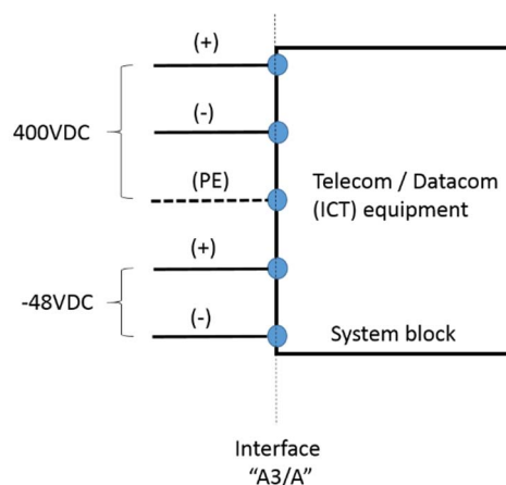
Figure 6: General identification of the A/A3 interface for multiple power feed for up to 400 VDC and -48 VDC inputs
