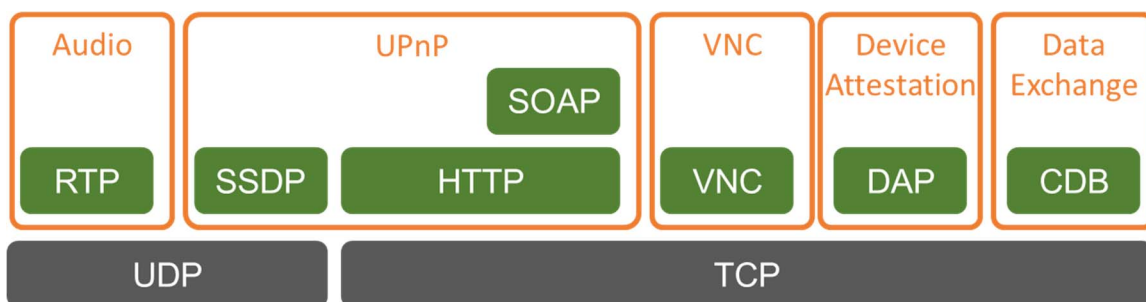
Figure 2: Session Layer
