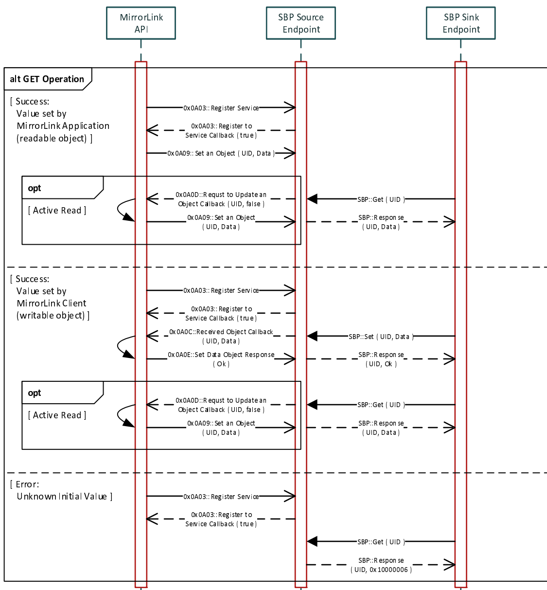
Figure 3: SBP Get Operation Examples
