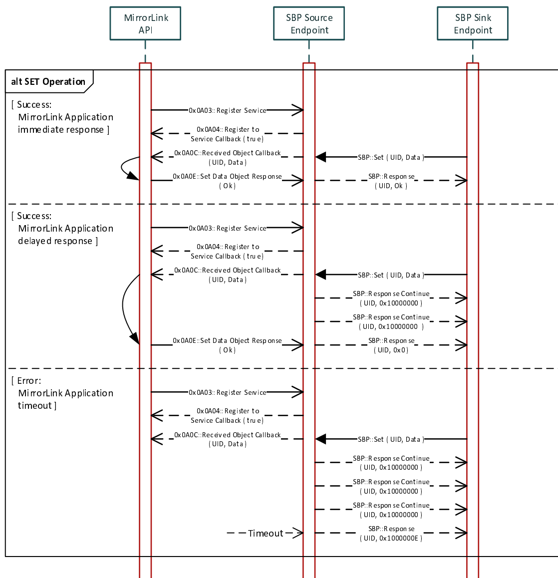
Figure 4: SBP Set Operation Examples
