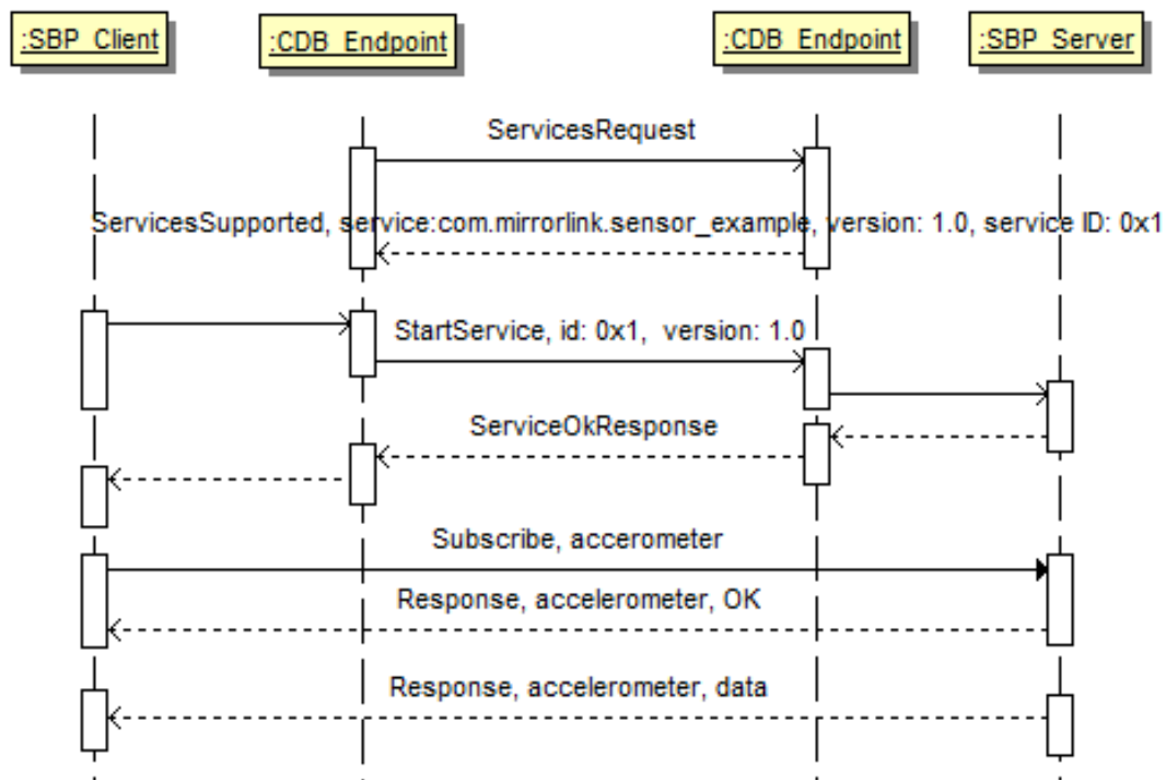
Figure 7: Example starting sequence of CDB/SBP
