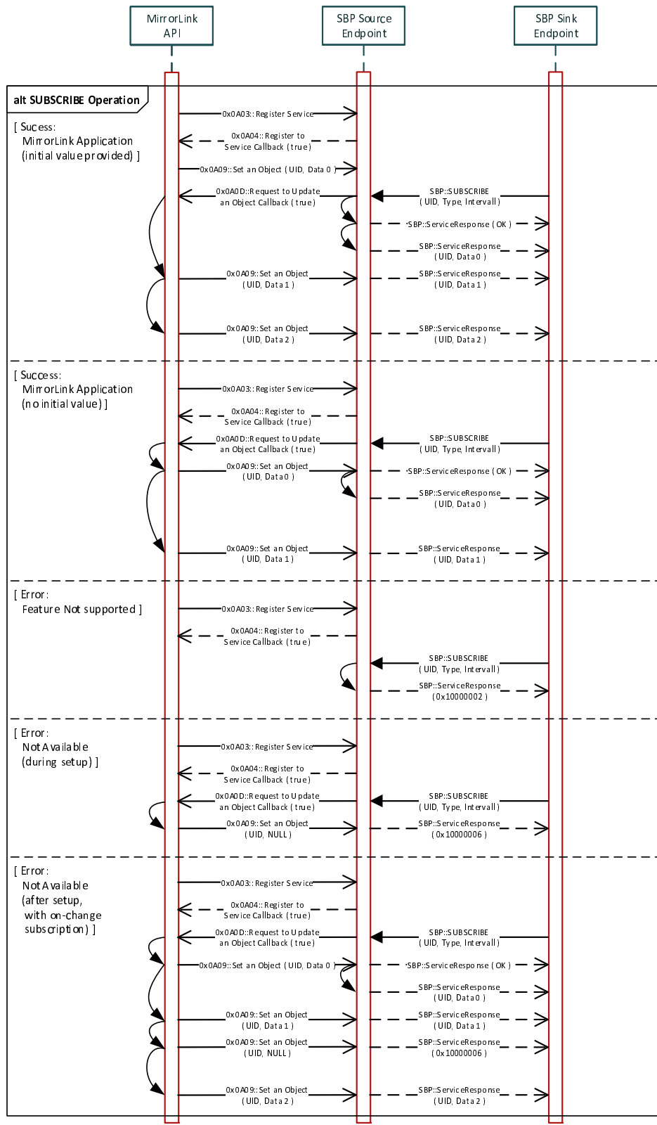
Figure 5: SBP Subscribe Operation Examples
