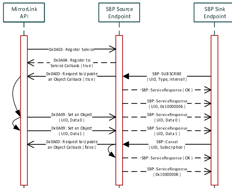
Figure 6: SBP Cancel Subscription Operation Example
