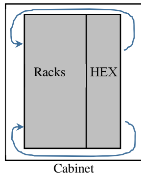
Figure B.1g: Air issuing racks are cooled with rear heat exchanger, air return is on the bottom and top
