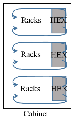
Figure B.1h: Air issuing racks are cooled with rear heat exchanger, air return is on the bottom and top in the rack
