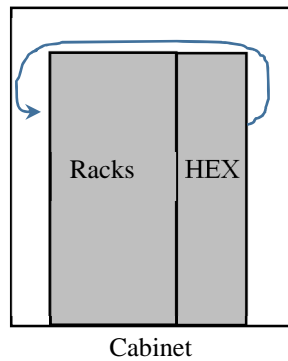
Figure B.1f: Air issuing racks are cooled with rear heat exchanger, air return is on the top
