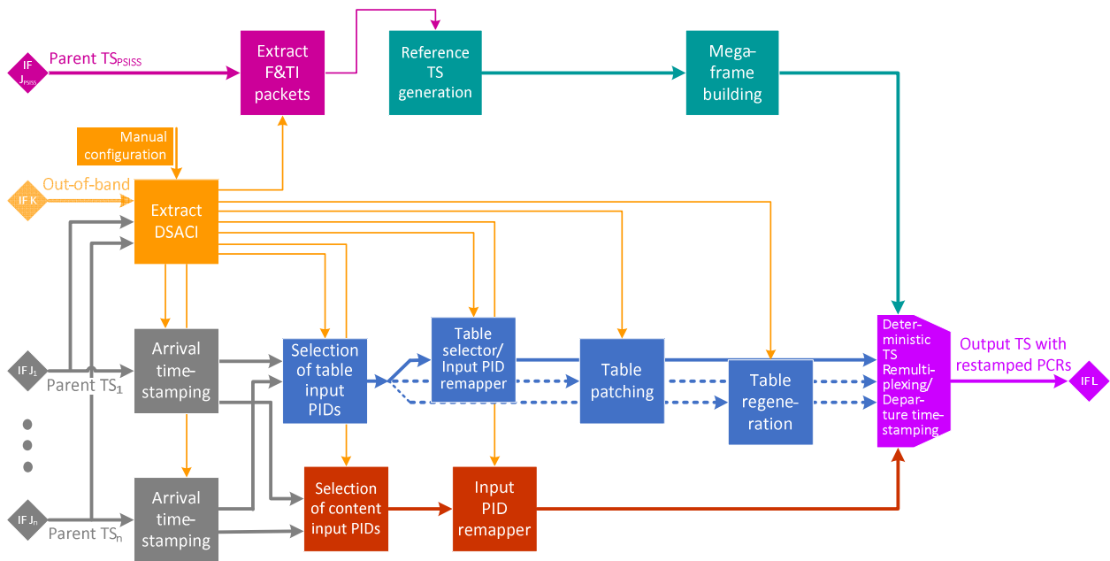
Figure 6: DSA processing (DVB-T case)
