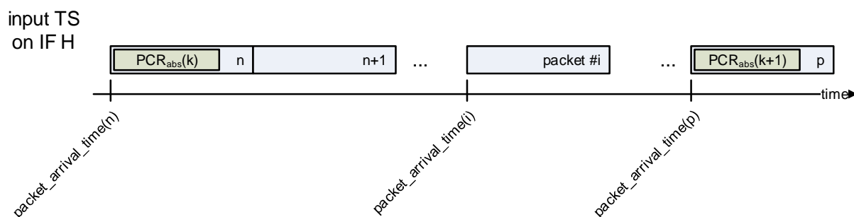
Figure 7: Arrival timestamping mechanism
