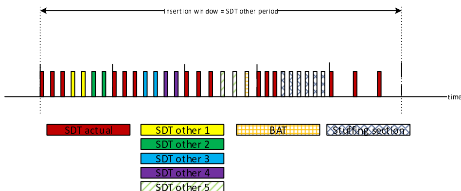
Figure 11: Example resulting packet distribution with 3 packets per SDT actual, 2 packets per SDT others, 1 packet per BAT, 6 stuffing sections of 1 packet
