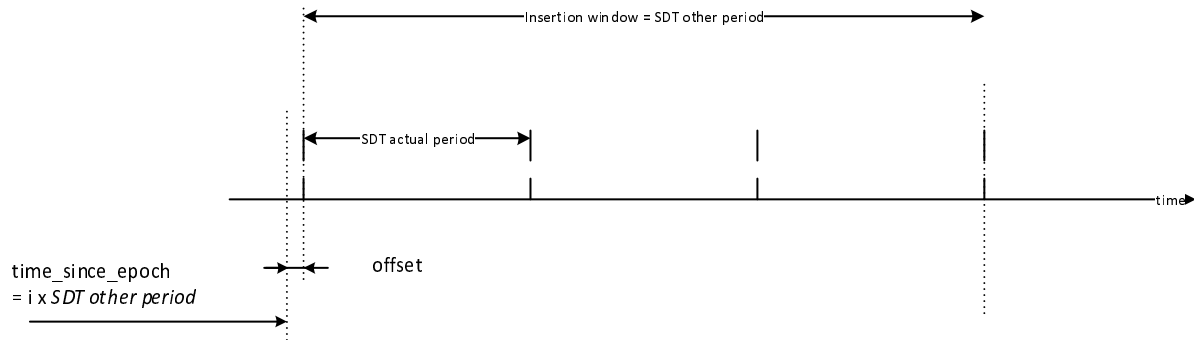
Figure 9: Definition of an SDT insertion window
