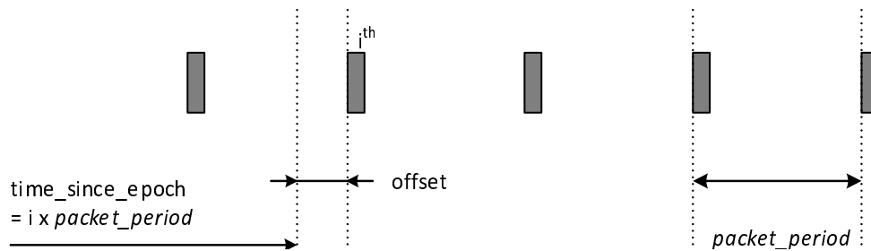
Figure 8: Generation of Virtual Arrival Timestamp for packets in CBR mode
