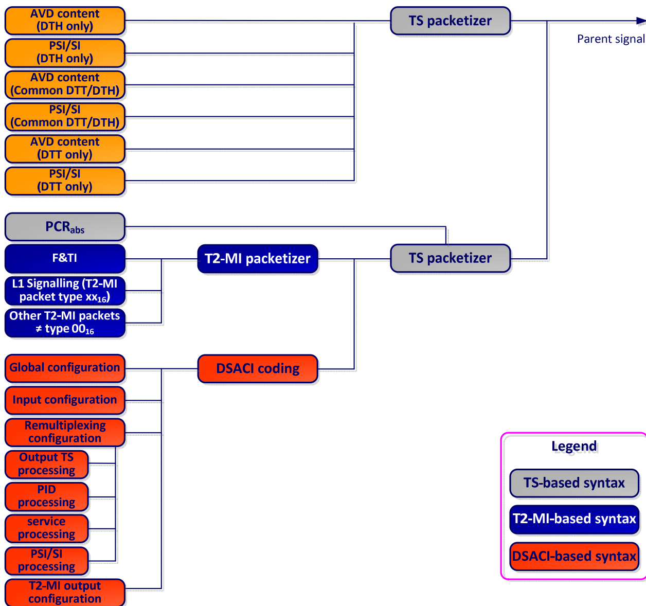
Figure 3: Parent Signal composition illustrating metadata and Audio/Video/Data content, DVB-T2 case
