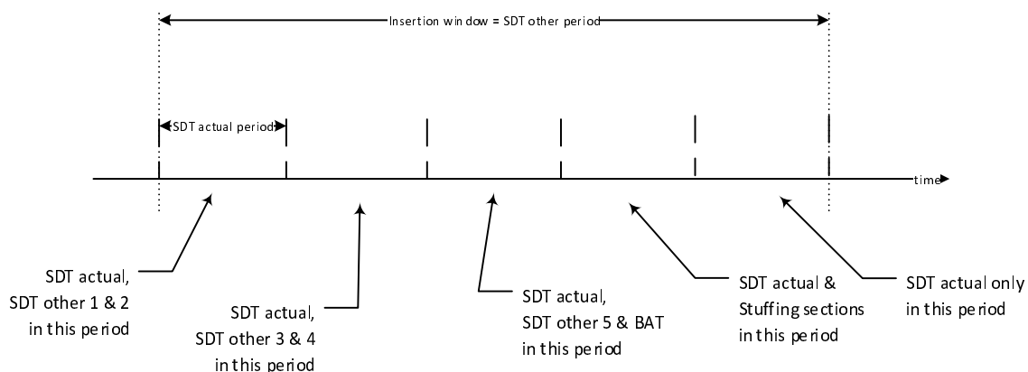
Figure 10: Example of repartitioning content within SDT actual interval, with P = 3 ( M_{\text{actual}} = 5 , n_{\text{oth}} = 5 , n_{\text{bat}} = 1 , n_{\text{stuff}} = 1 )
