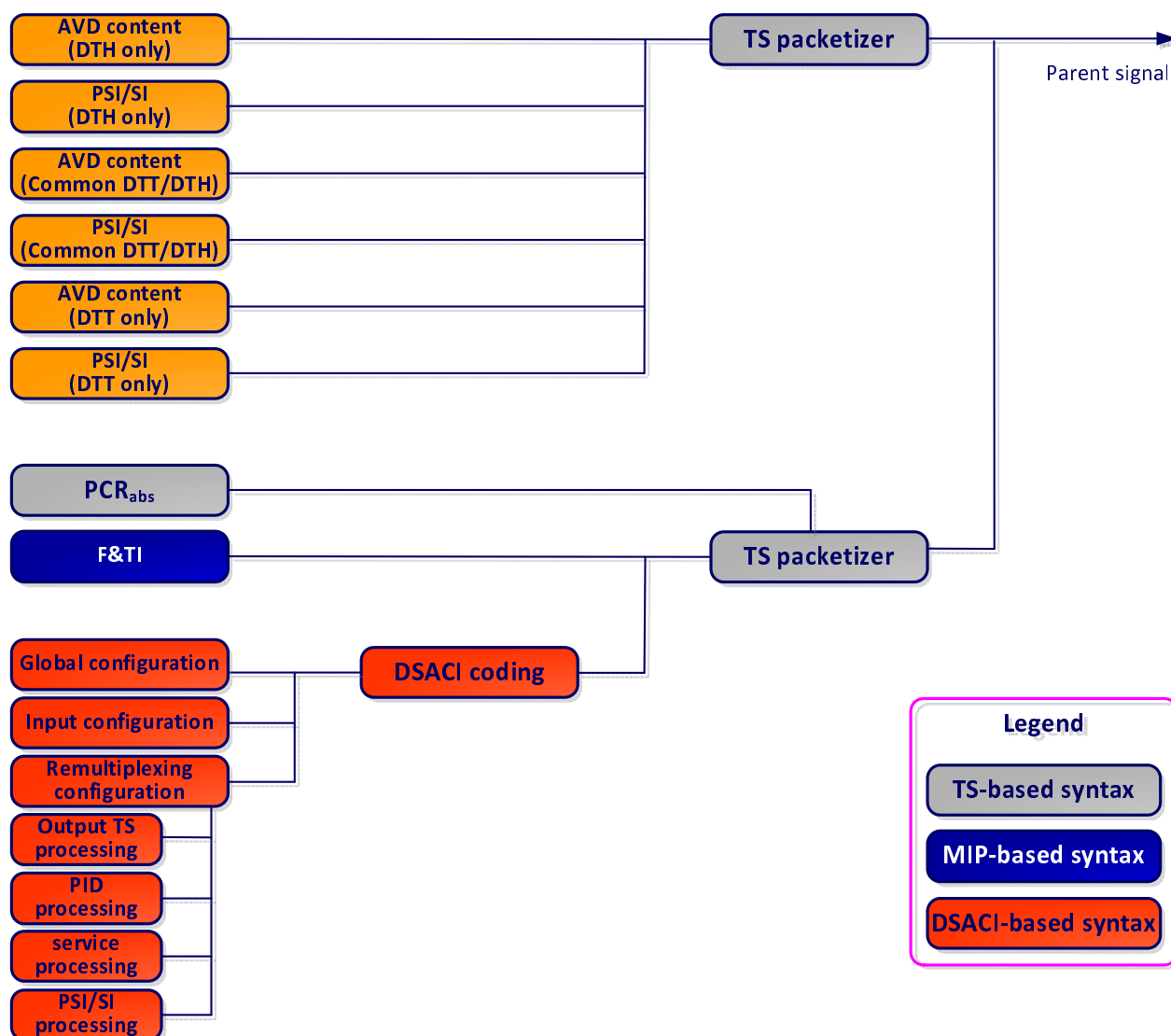
Figure 4: Parent Signal composition illustrating metadata and Audio/Video/Data content, DVB-T case
