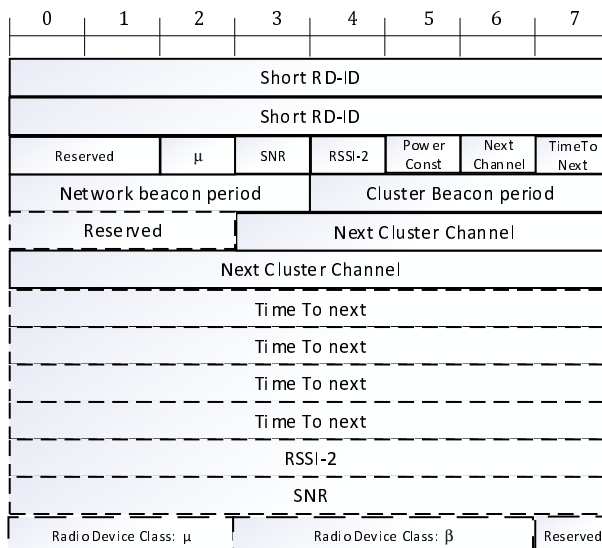
Figure 6.4.3.6-1: Neighbouring IE
