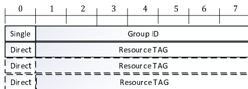
Figure 6.4.3.9-1: Group Assignment IE
