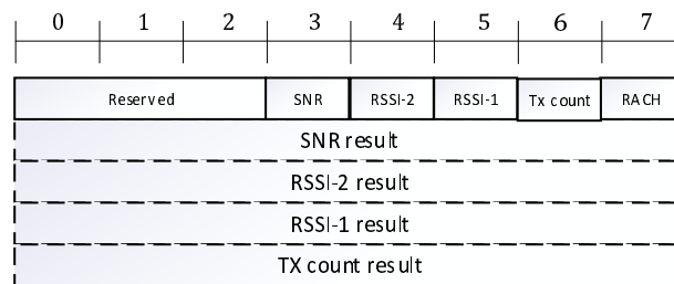
Figure 6.4.3.12-1: Measurement report IE
