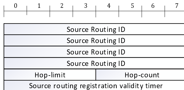
Figure 6.4.3.16-1: Source Routing IE
