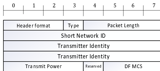
Figure 6.2.1-1: Physical Layer Control Field: Type 1
