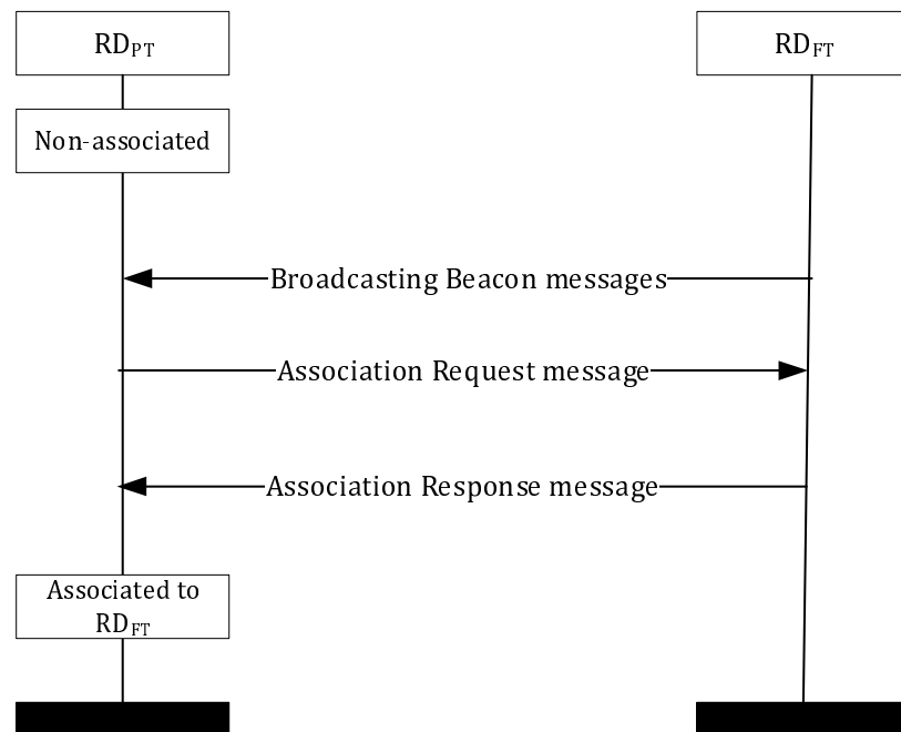
Figure 5.8.1-1: Association signalling
