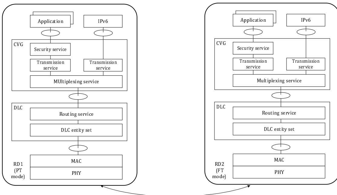
Figure 4.2.1-1: Illustration of overall protocol architecture
