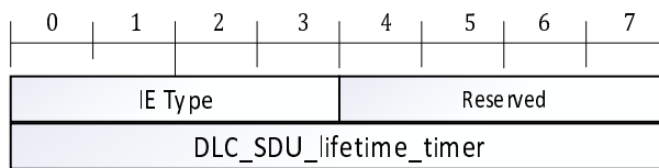
Figure 5.3.3.2-1: DLC Timer configuration PDU
