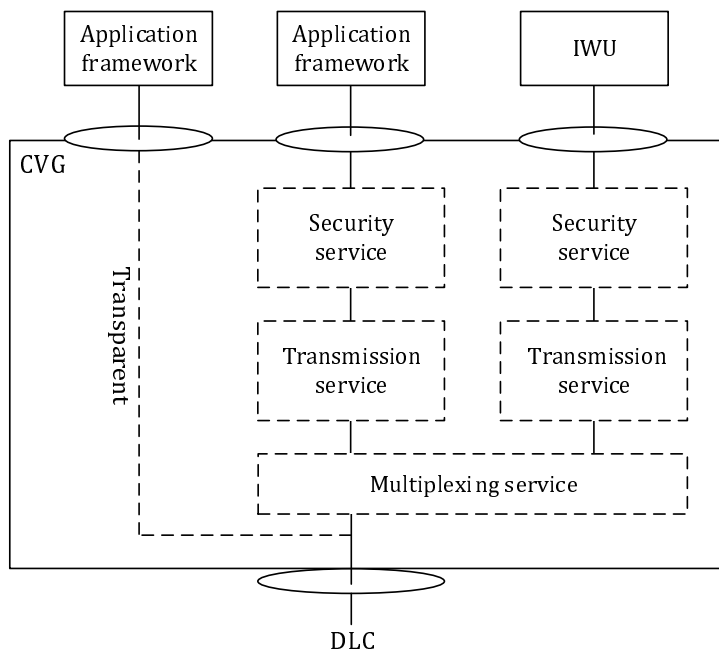
Figure 4.2.3-1: CVG architecture
