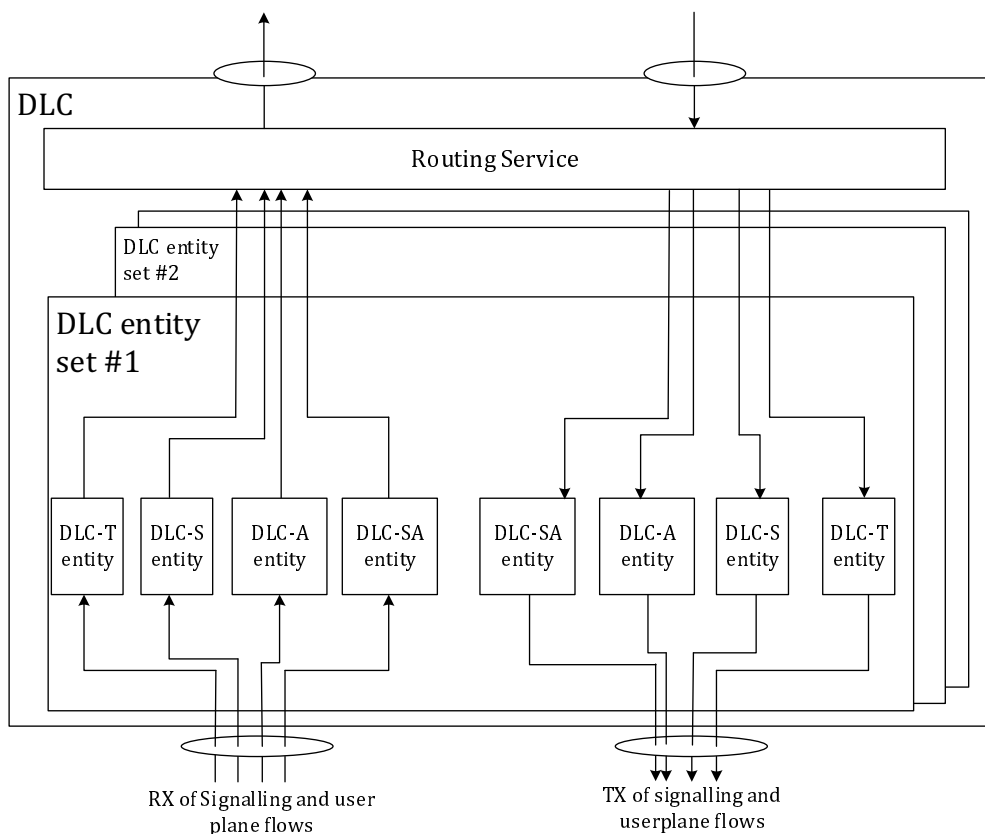
Figure 4.2.2-2: DLC architecture
