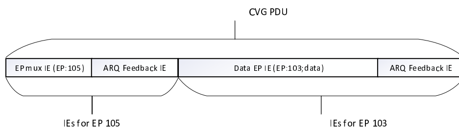
Figure 6.2.4.2-1: An example of organizing multiple IEs in CVG PDU
