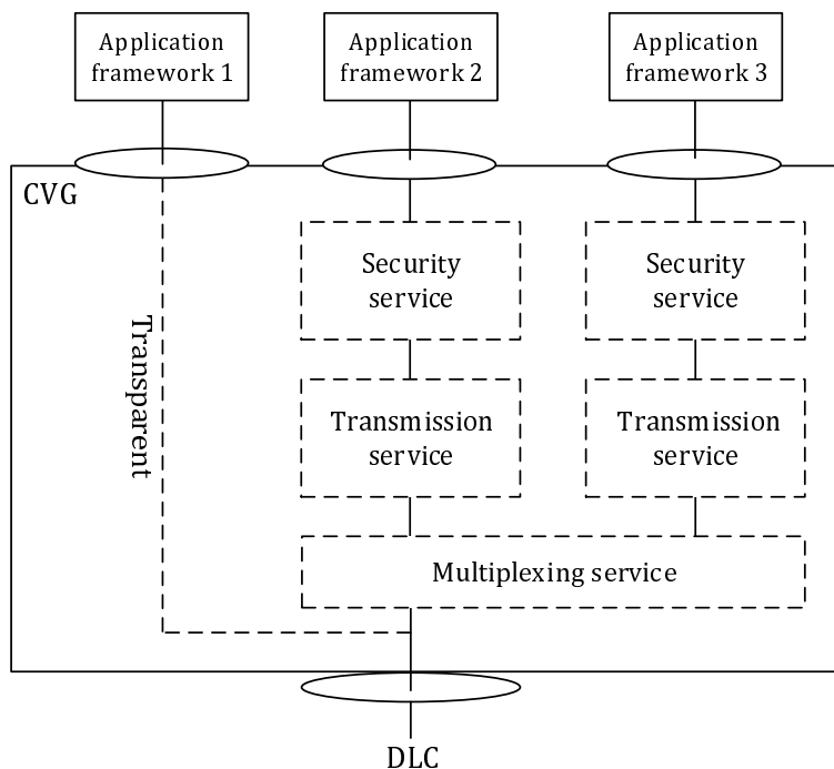
Figure 4.2.3-1: CVG architecture
