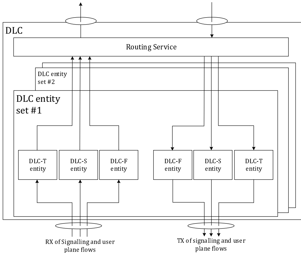
Figure 4.2.2-2: DLC architecture
