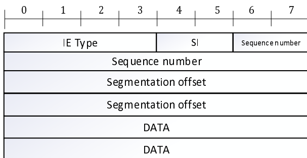
Figure 5.3.3.1-2: Segmentation PDU, for SDU Segment
