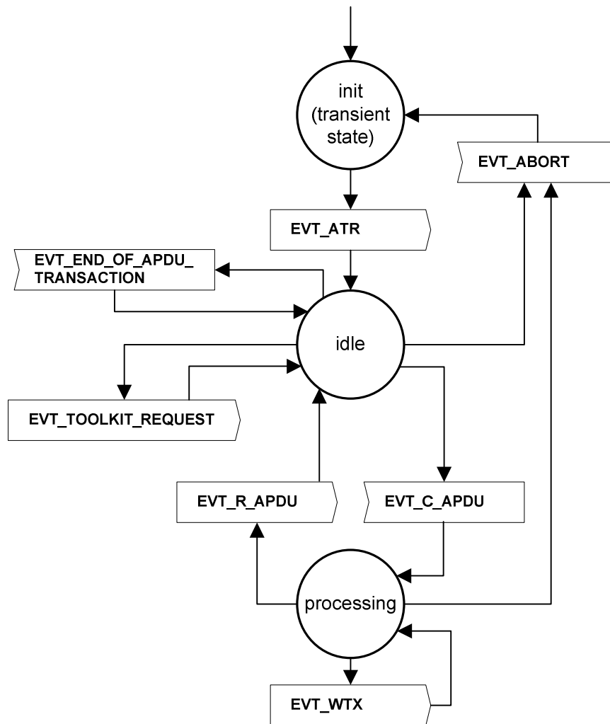
Figure 10.2: State transitions
