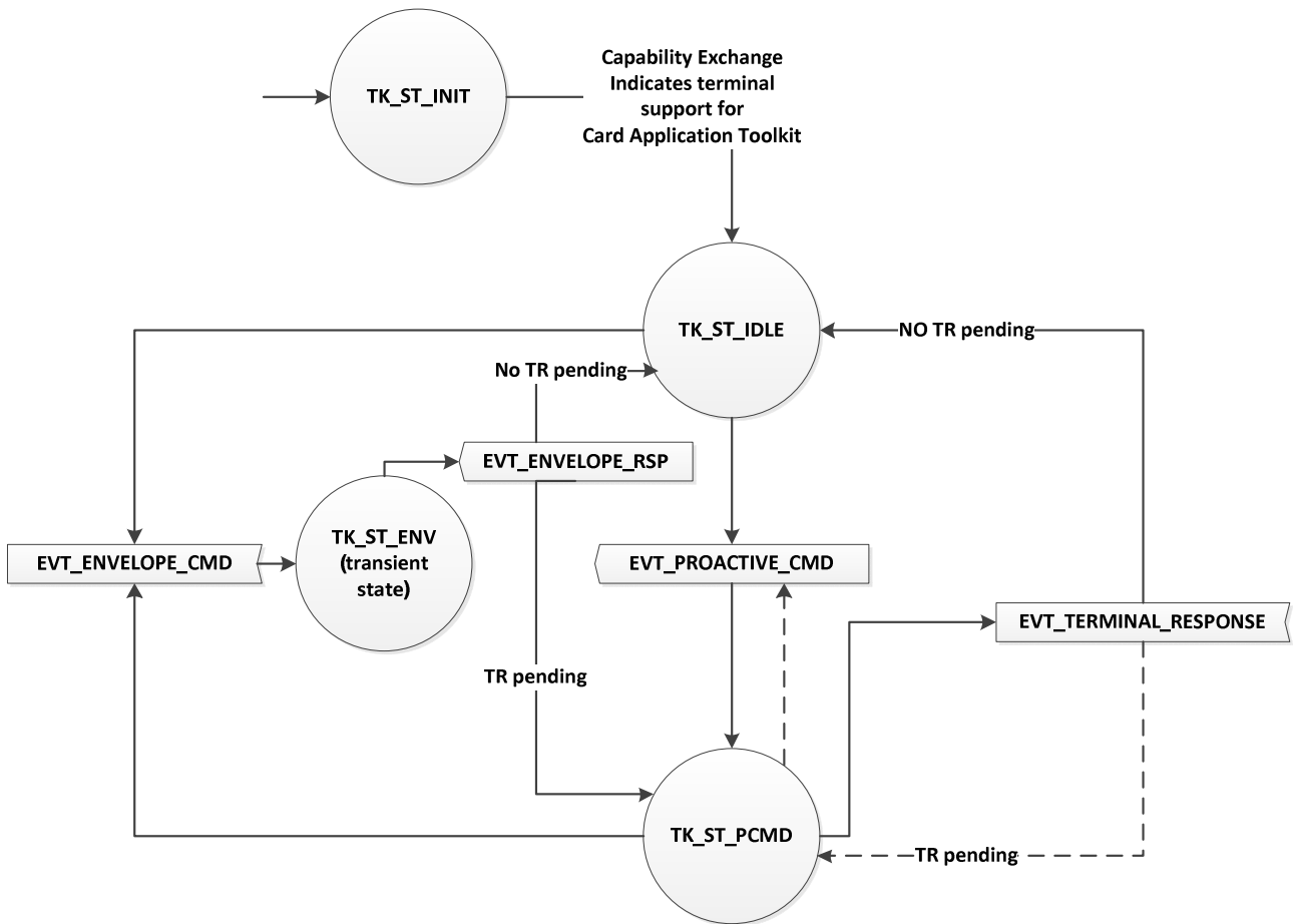
Figure 10.10: State transitions
