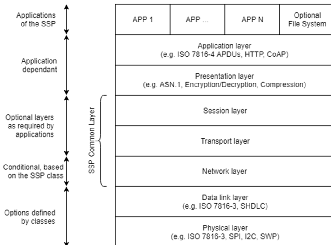
Figure 5.3: SSP protocol stack
